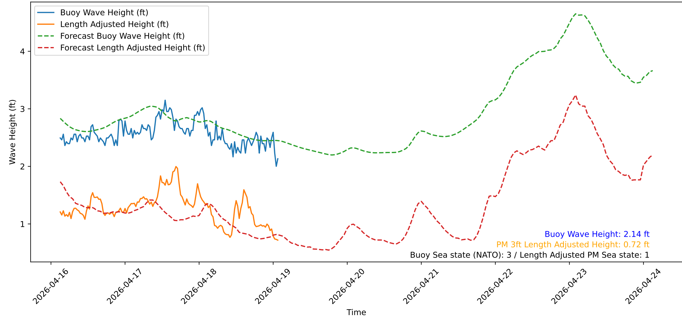
Wave Heights over Time for Red Beach at 2026-04-19 02:50:51
