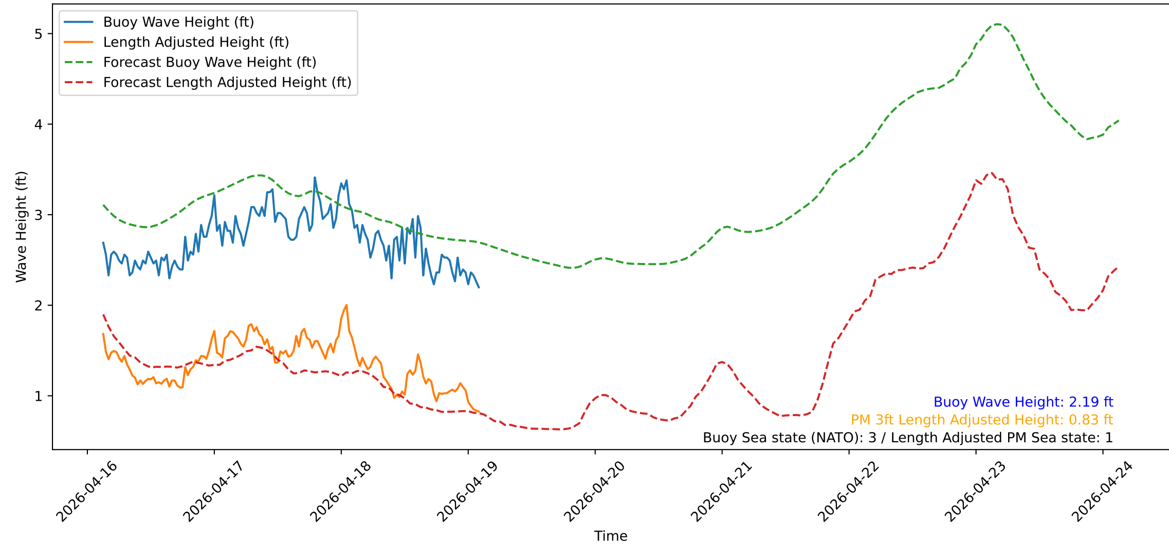
Wave Heights over Time for Oceanside Harbor at 2026-04-19 02:50:31
