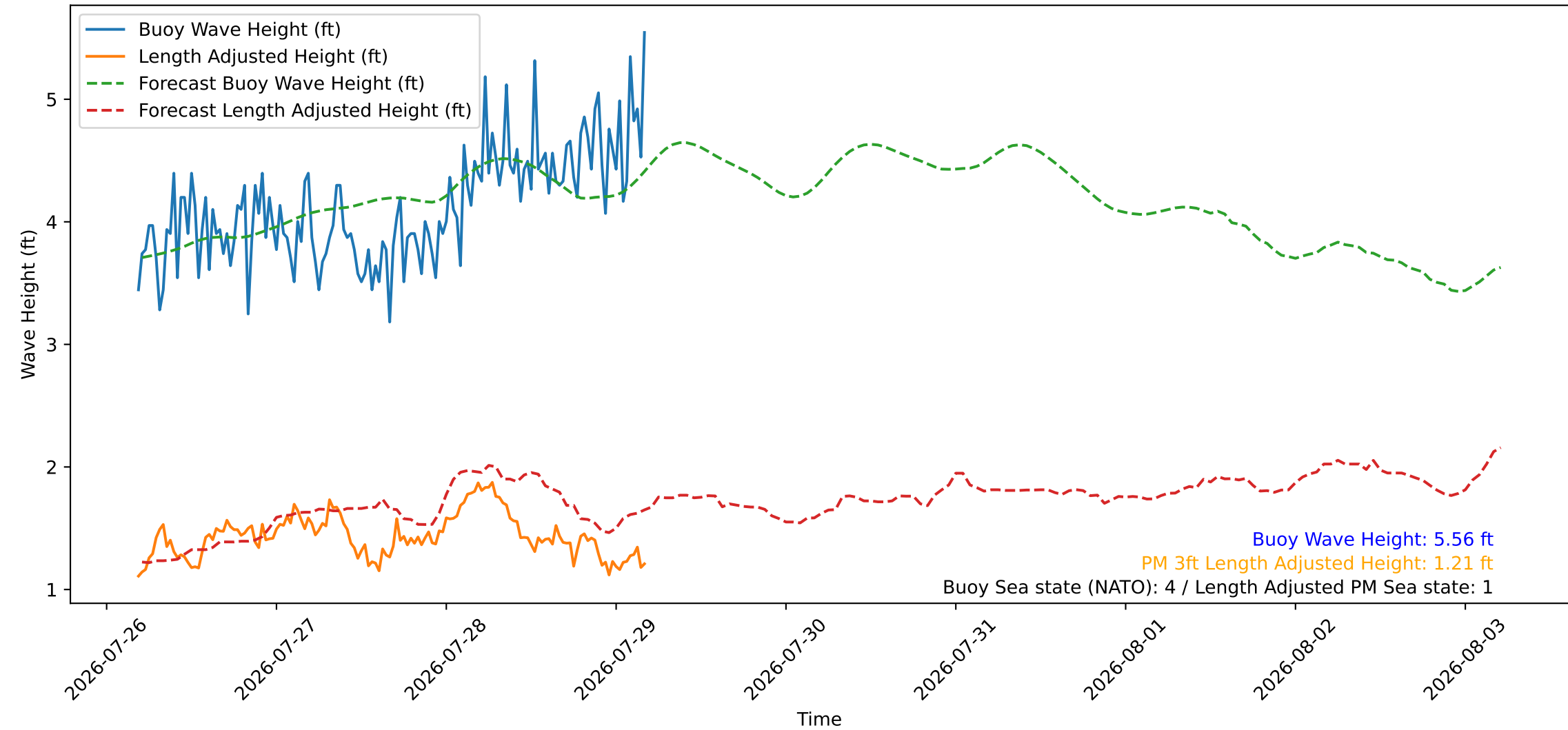
Wave Heights over Time for Oceanside Harbor at 2026-07-29 04:40:27
