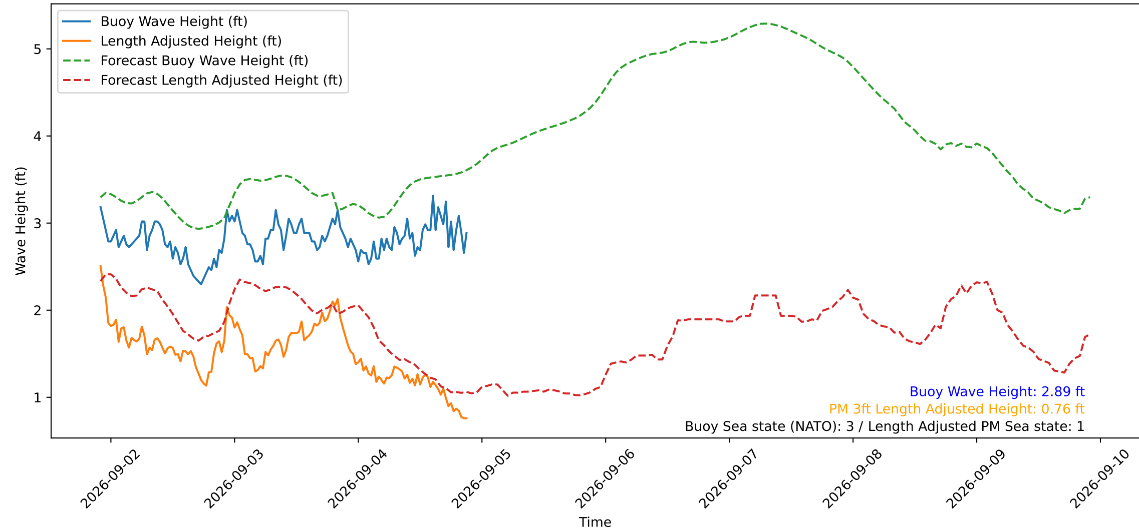
Wave Heights over Time for Red Beach at 2026-09-04 21:50:50
