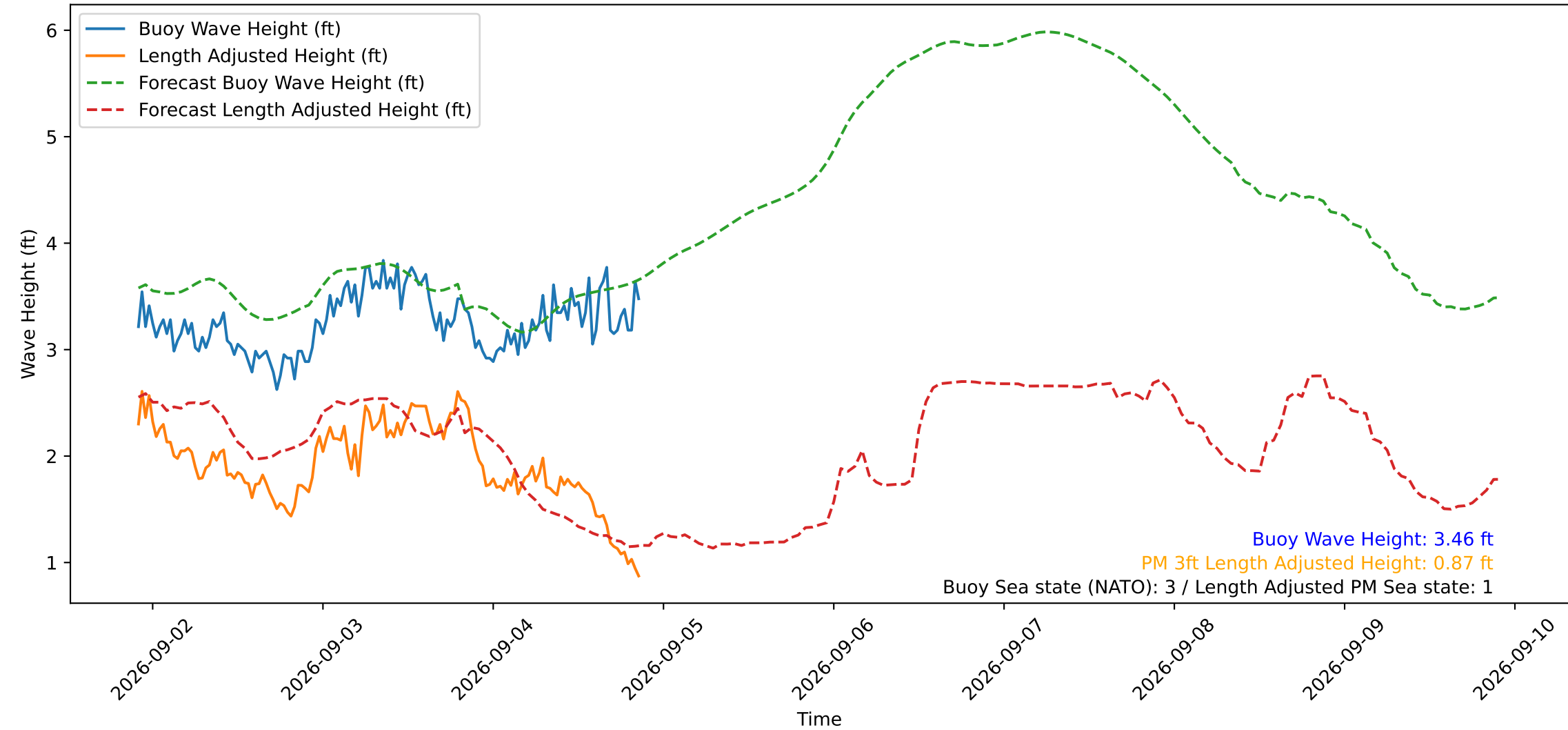
Wave Heights over Time for Oceanside Harbor at 2026-09-04 21:50:30
