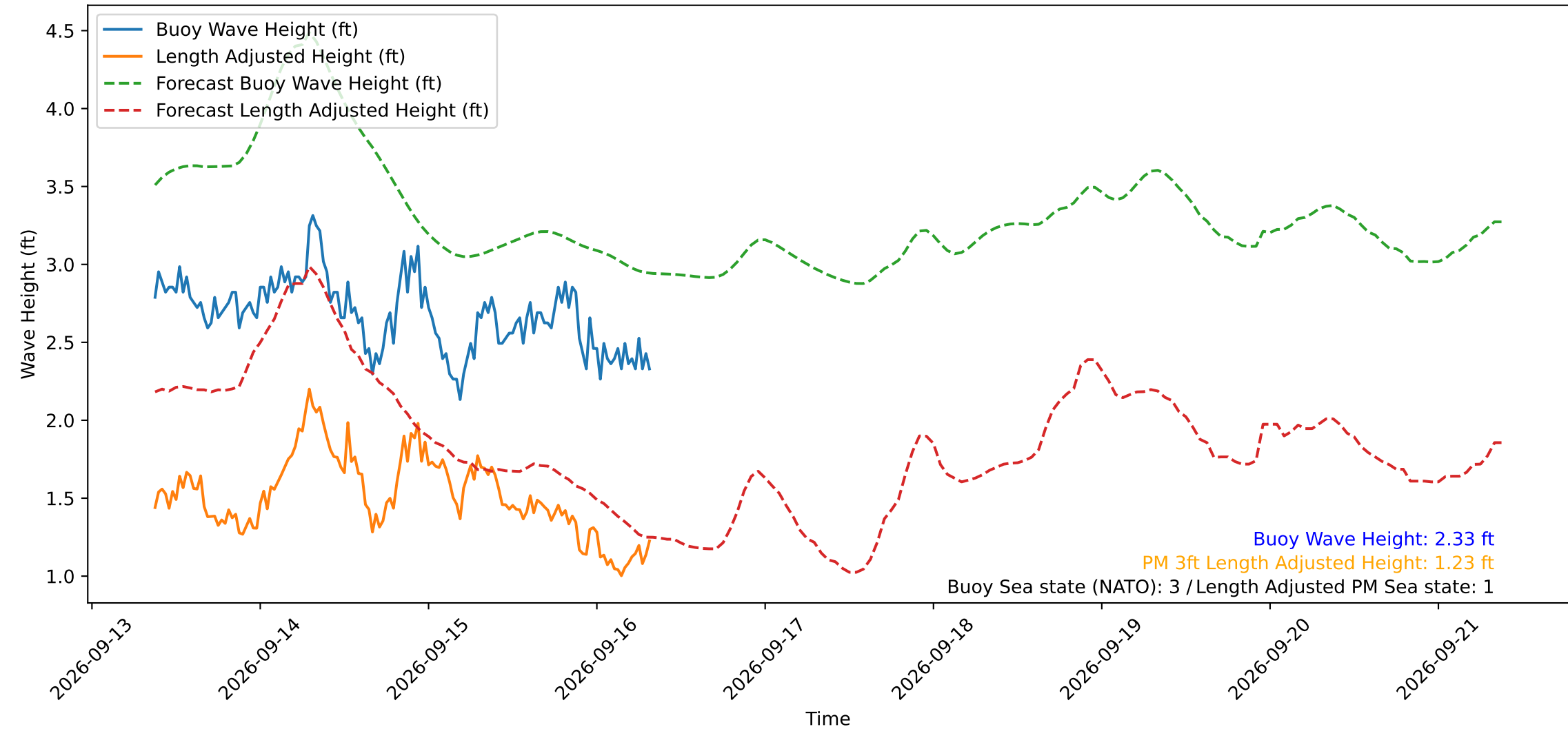
Wave Heights over Time for Green Beach at 2026-09-16 08:31:12
