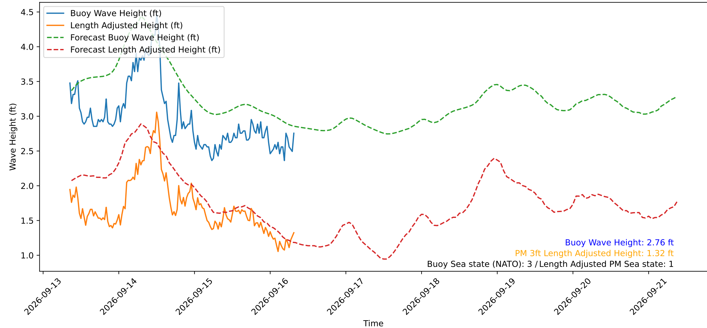
Wave Heights over Time for Oceanside Harbor at 2026-09-16 08:30:30
