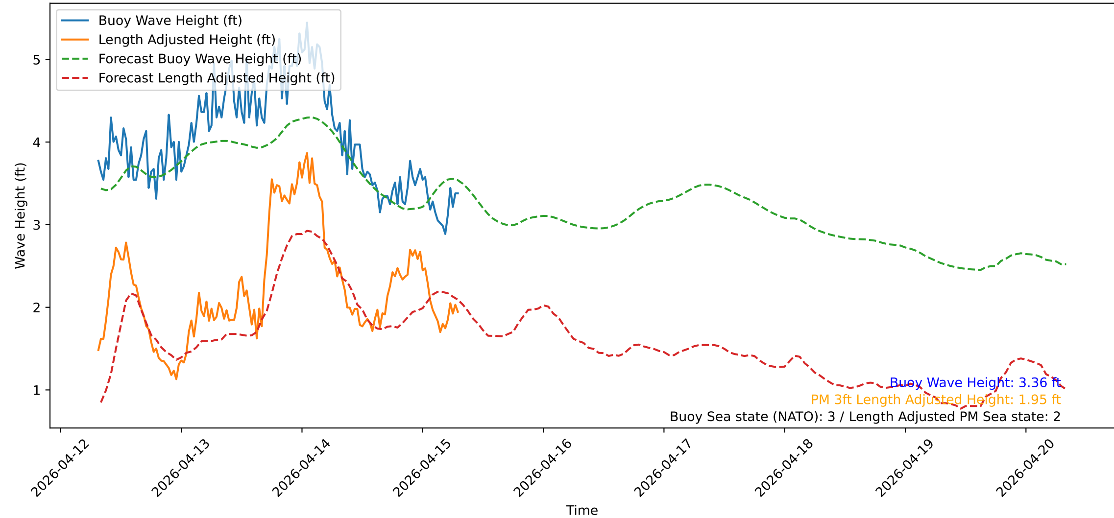
Wave Heights over Time for Oceanside Harbor at 2026-04-15 07:30:32
