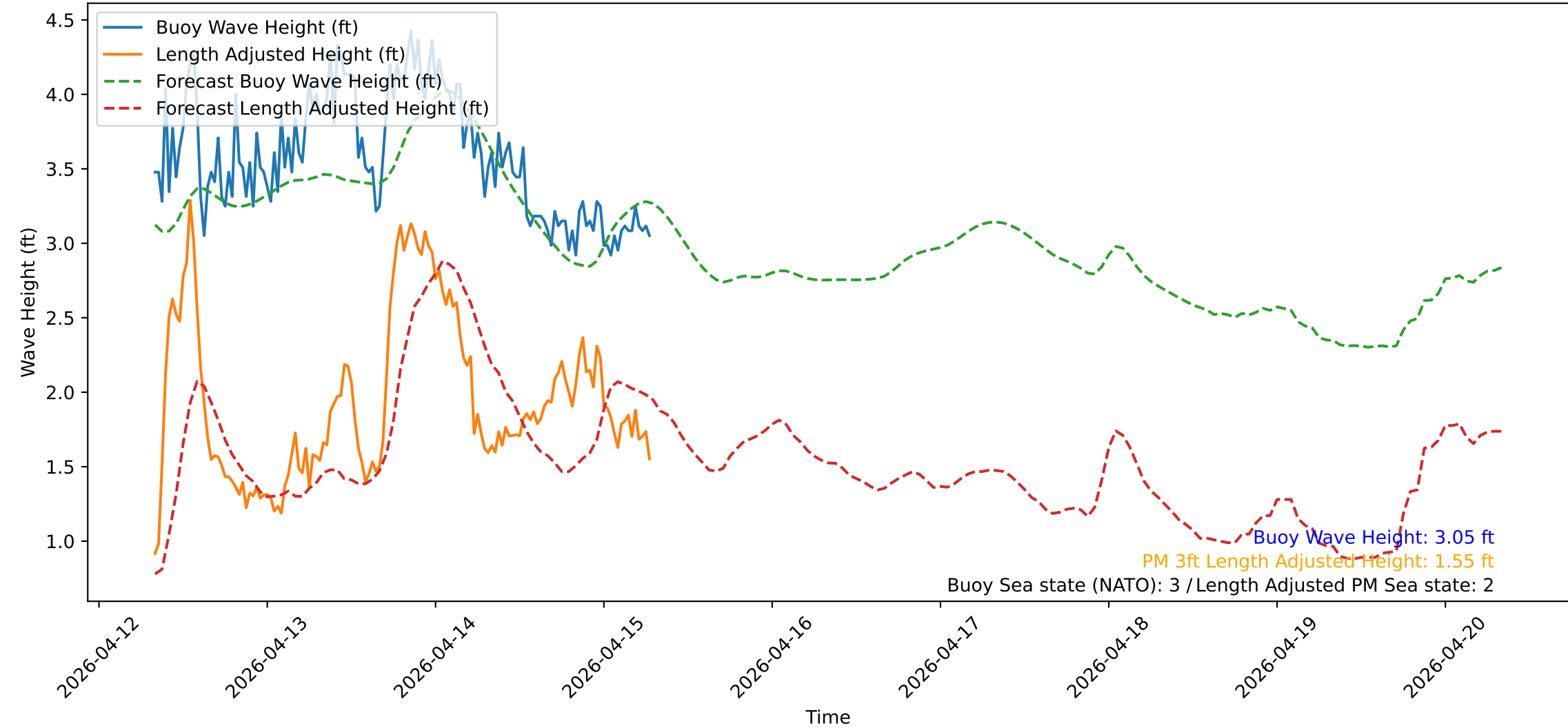
Wave Heights over Time for Red Beach at 2026-04-15 07:30:51
