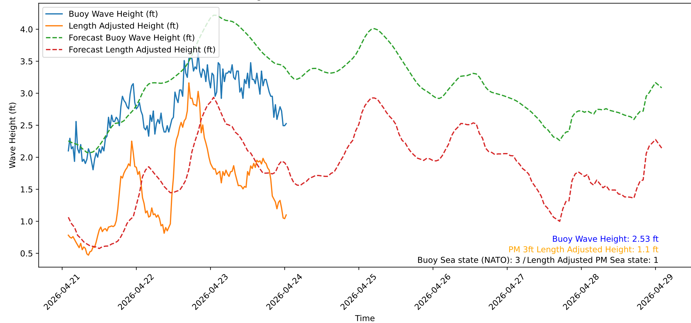
Wave Heights over Time for Red Beach at 2026-04-24 01:30:50
