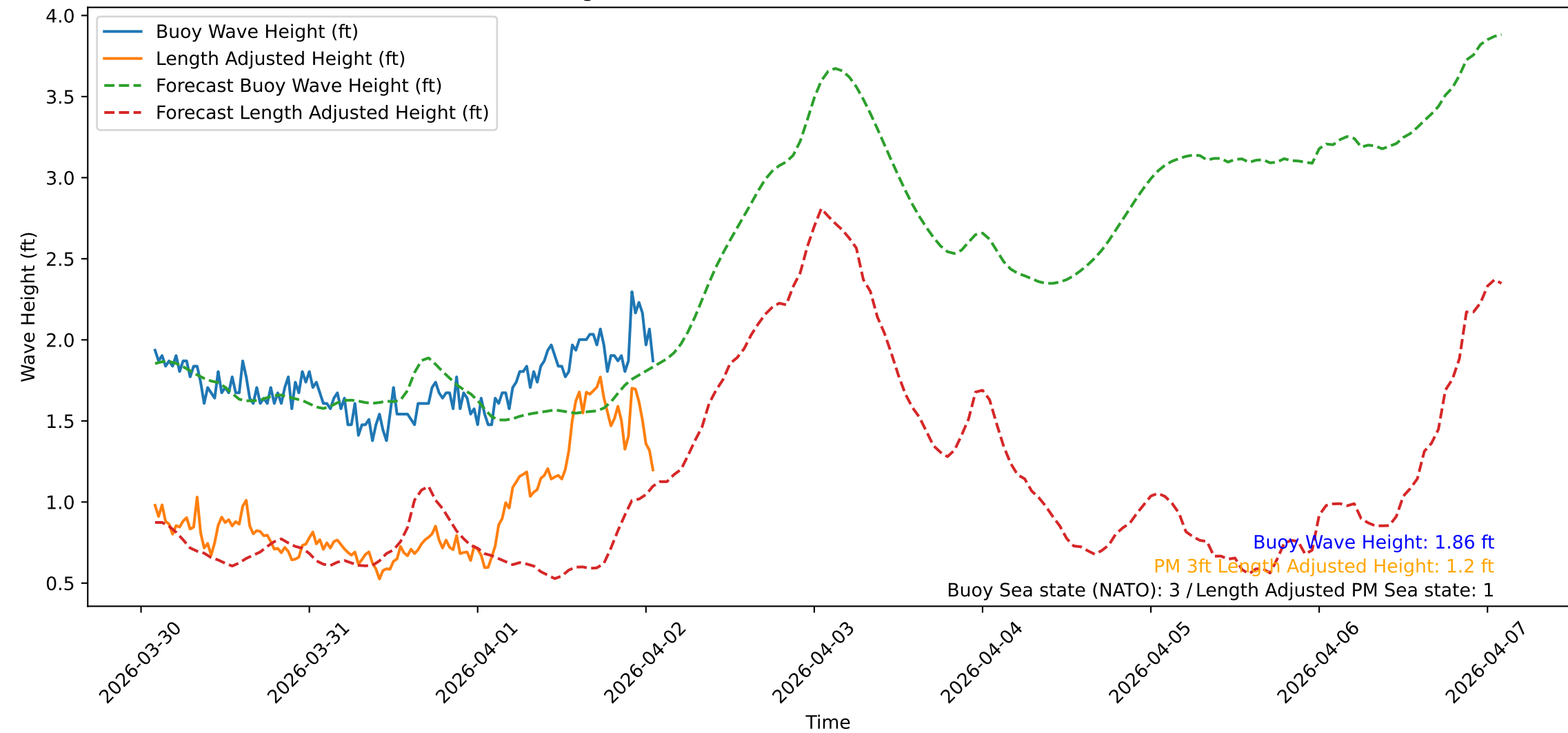
Wave Heights over Time for Red Beach at 2026-04-02 01:50:47
