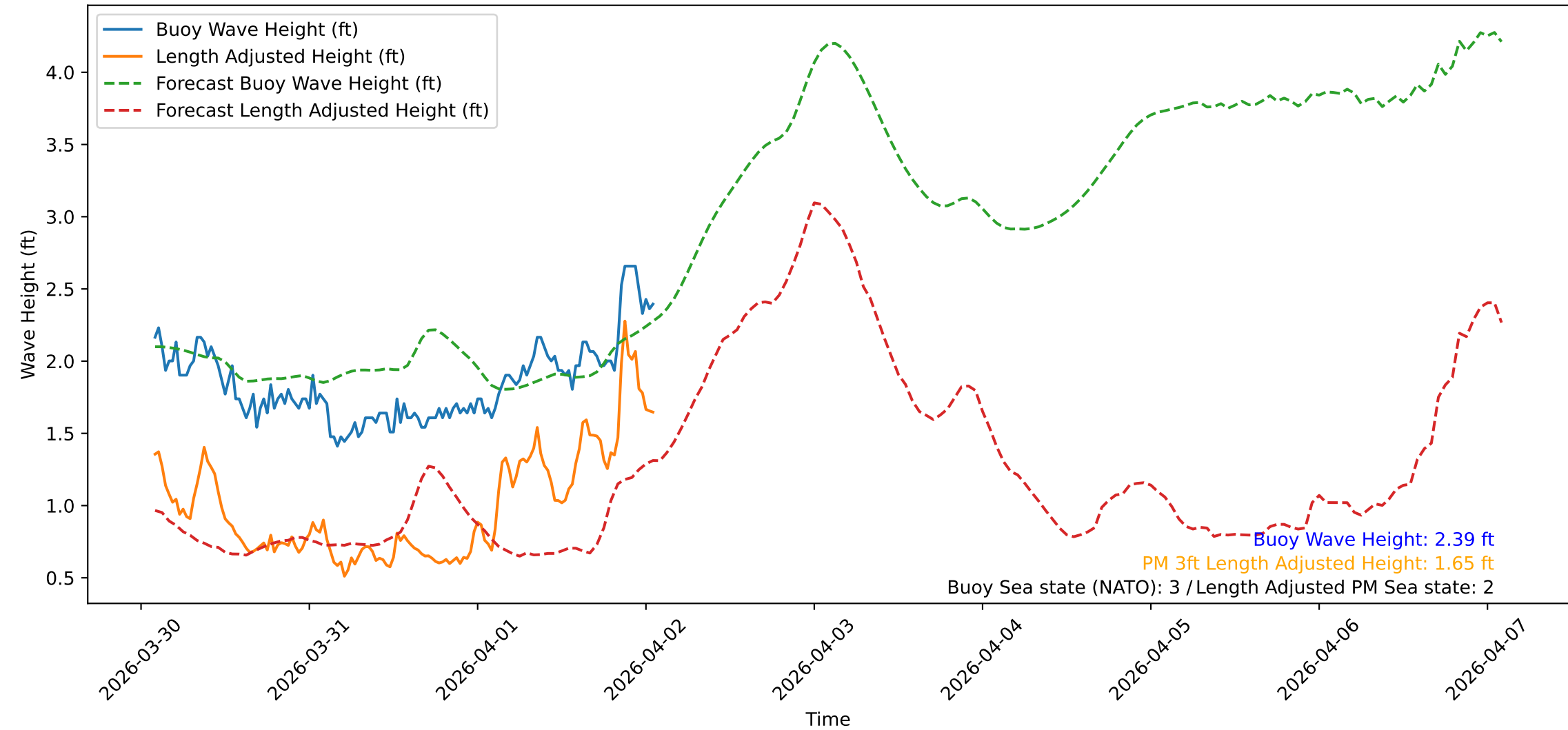
Wave Heights over Time for Green Beach at 2026-04-02 01:51:09
