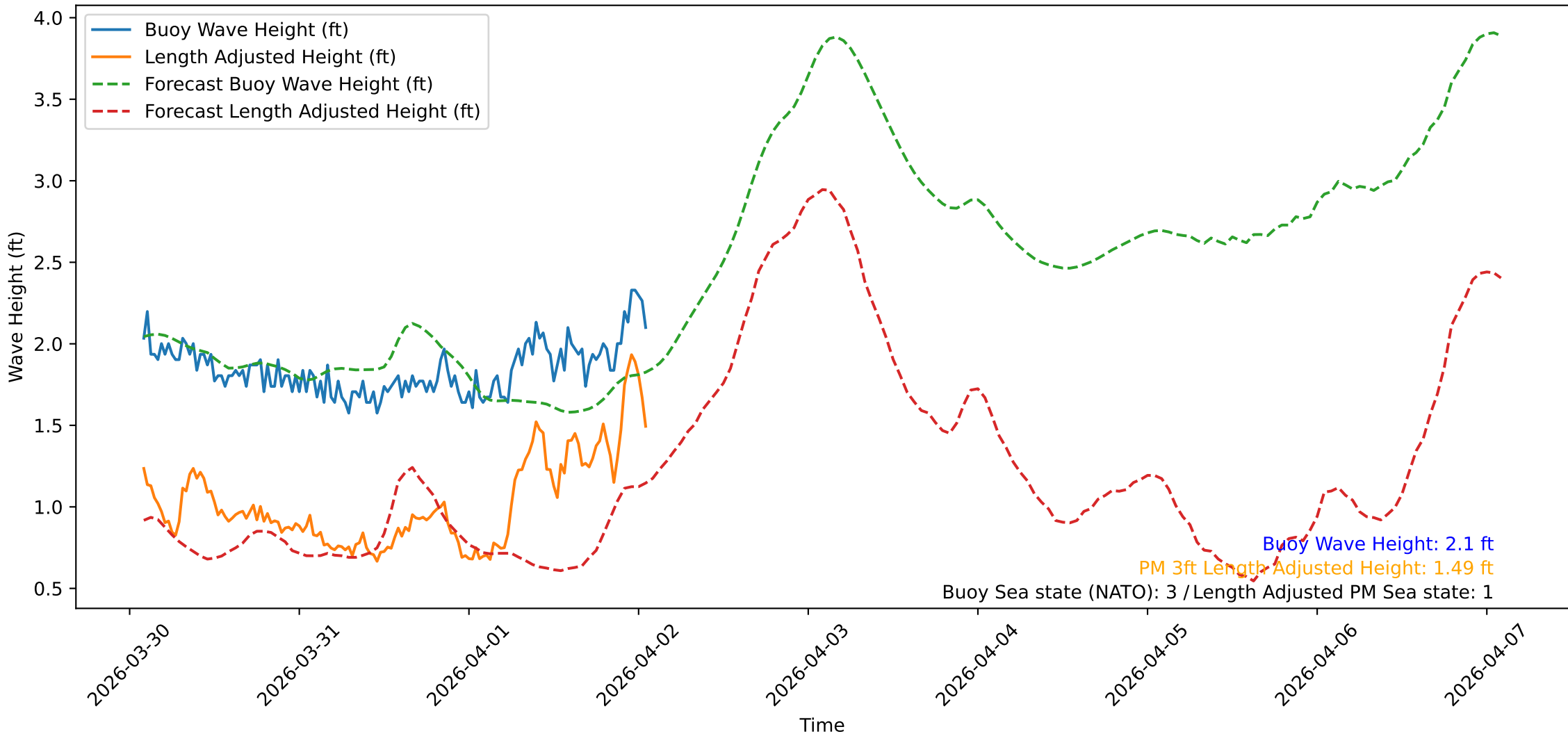
Wave Heights over Time for Oceanside Harbor at 2026-04-02 01:50:31
