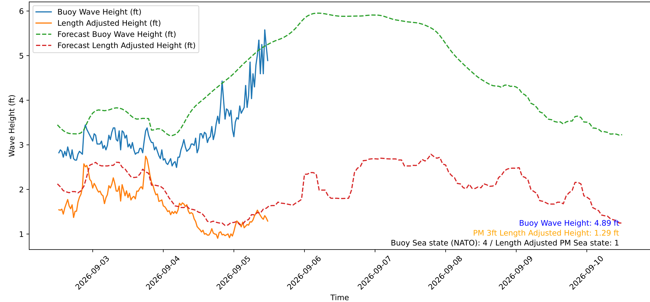
Wave Heights over Time for Green Beach at 2026-09-05 12:21:14
