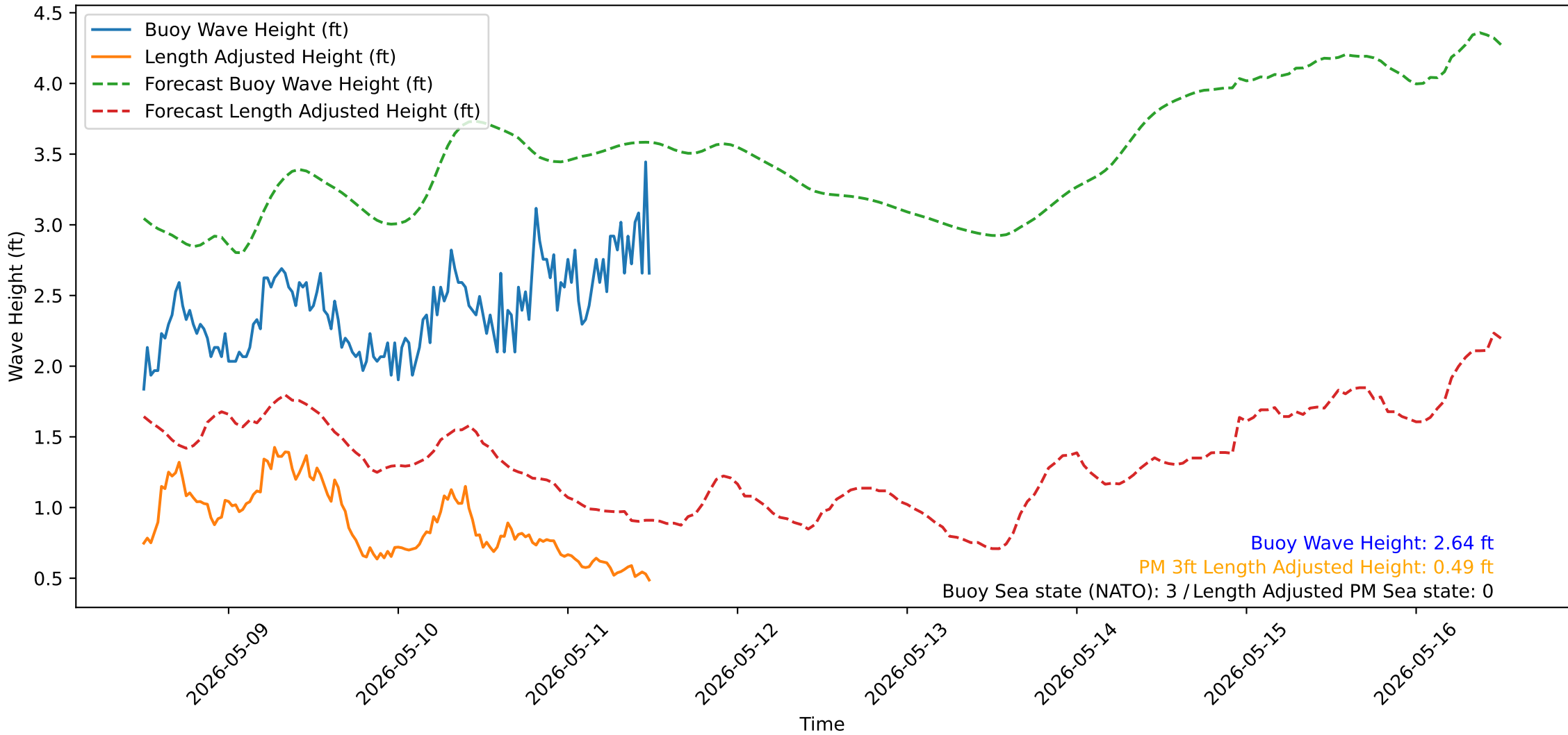
Wave Heights over Time for Green Beach at 2026-05-11 12:11:13
