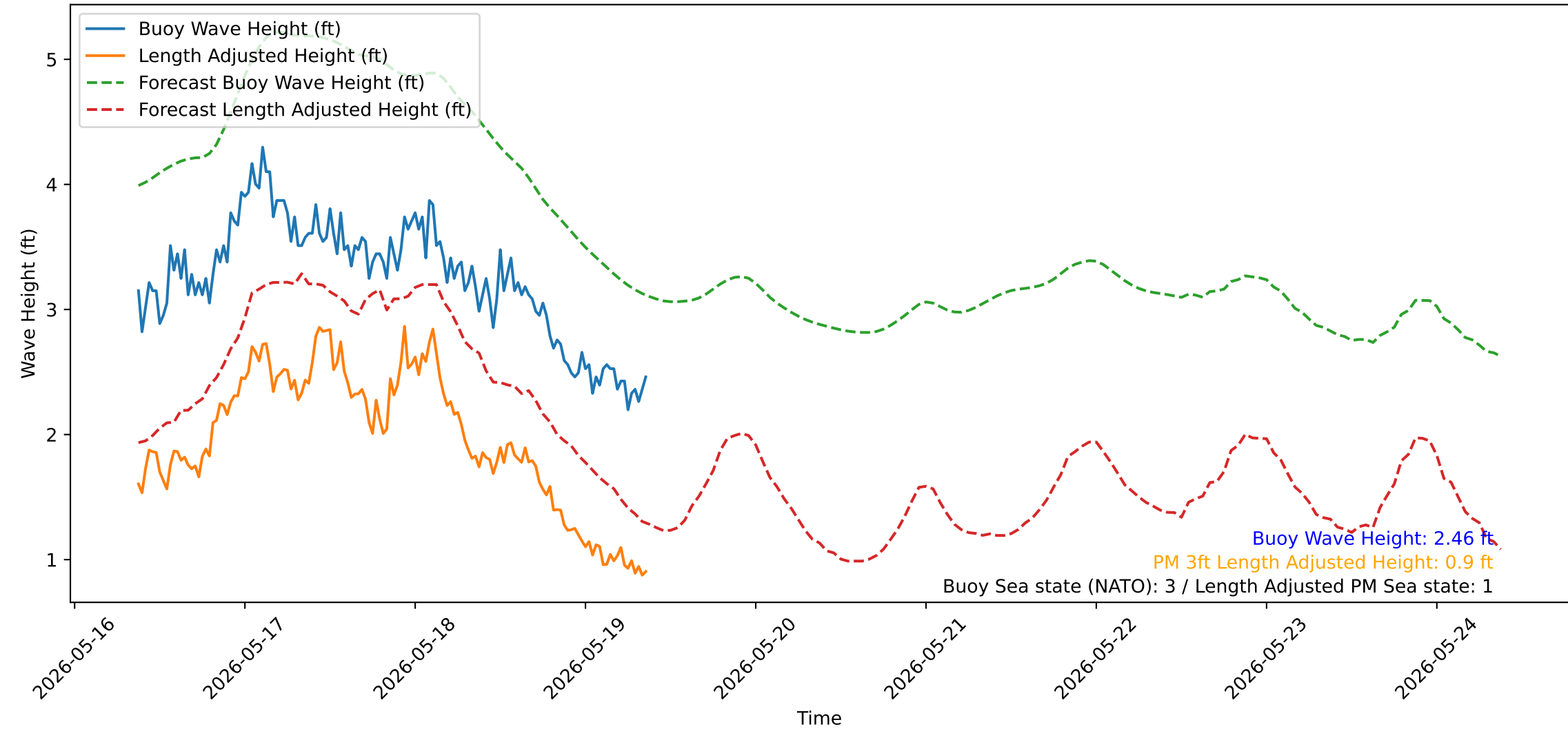
Wave Heights over Time for Oceanside Harbor at 2026-05-19 09:10:32
