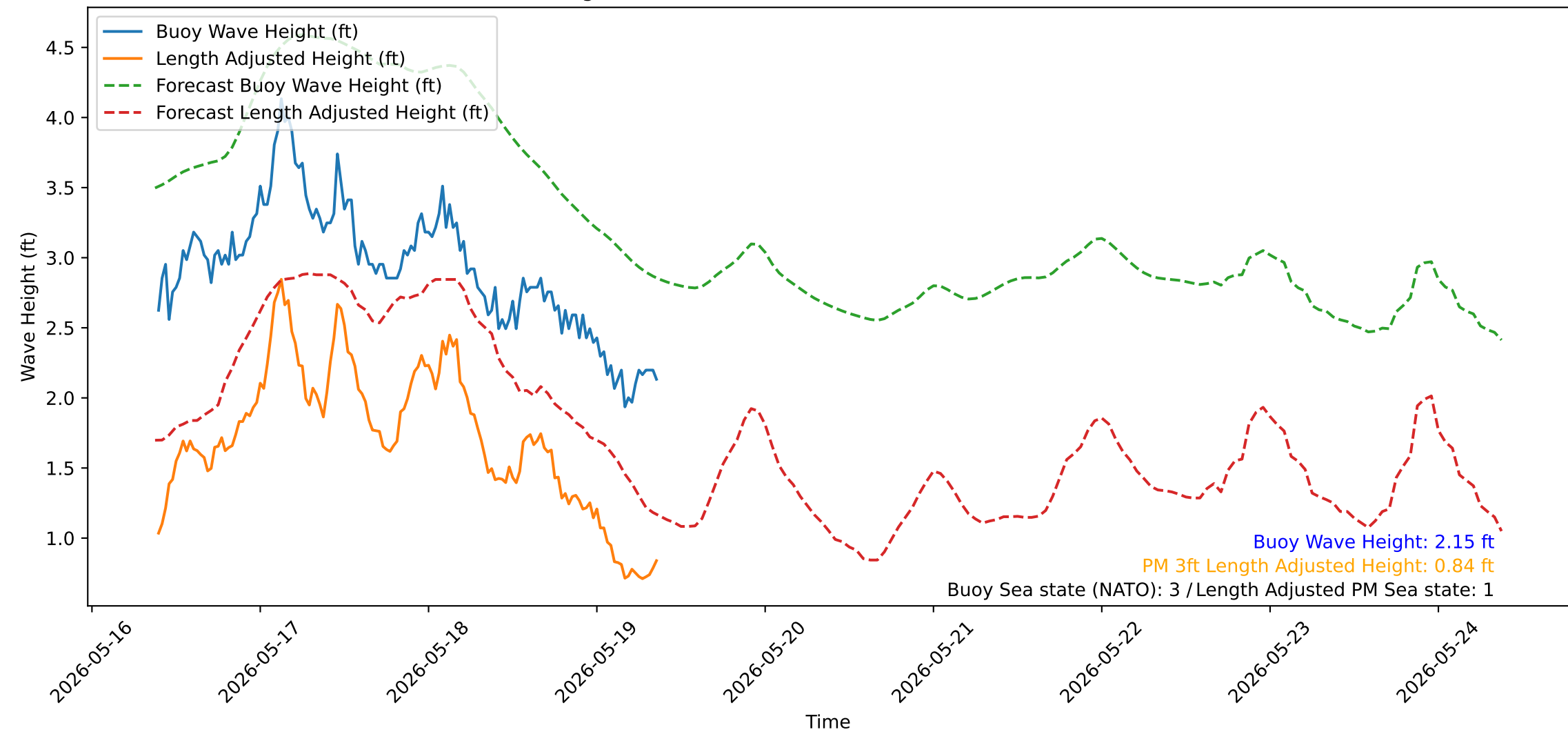
Wave Heights over Time for Red Beach at 2026-05-19 09:10:51
