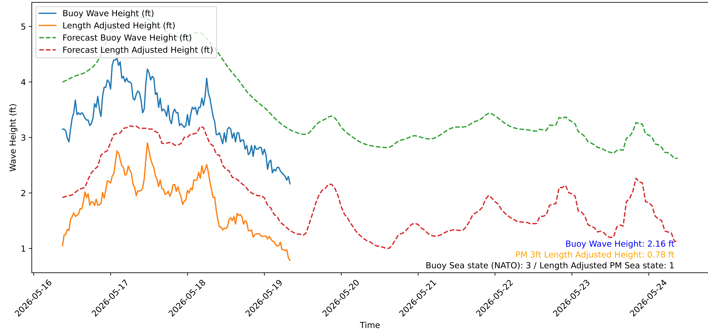
Wave Heights over Time for Green Beach at 2026-05-19 09:11:13
