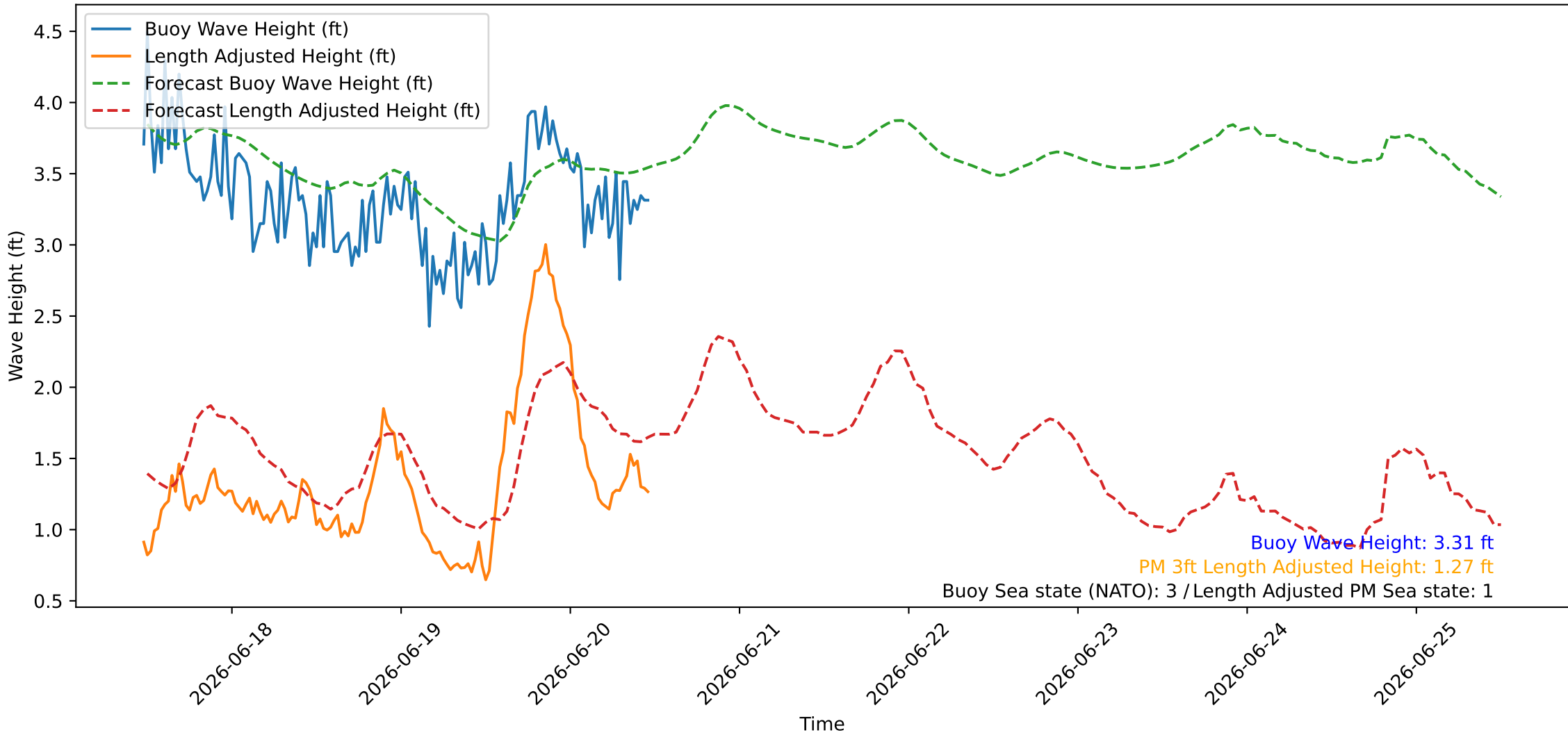
Wave Heights over Time for Green Beach at 2026-06-20 11:41:08
