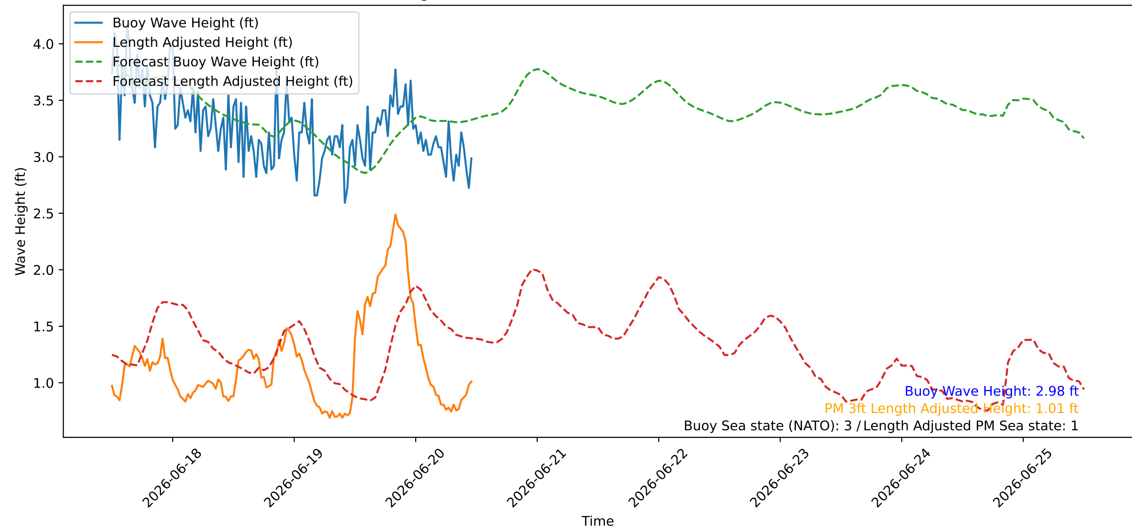
Wave Heights over Time for Red Beach at 2026-06-20 11:40:45
