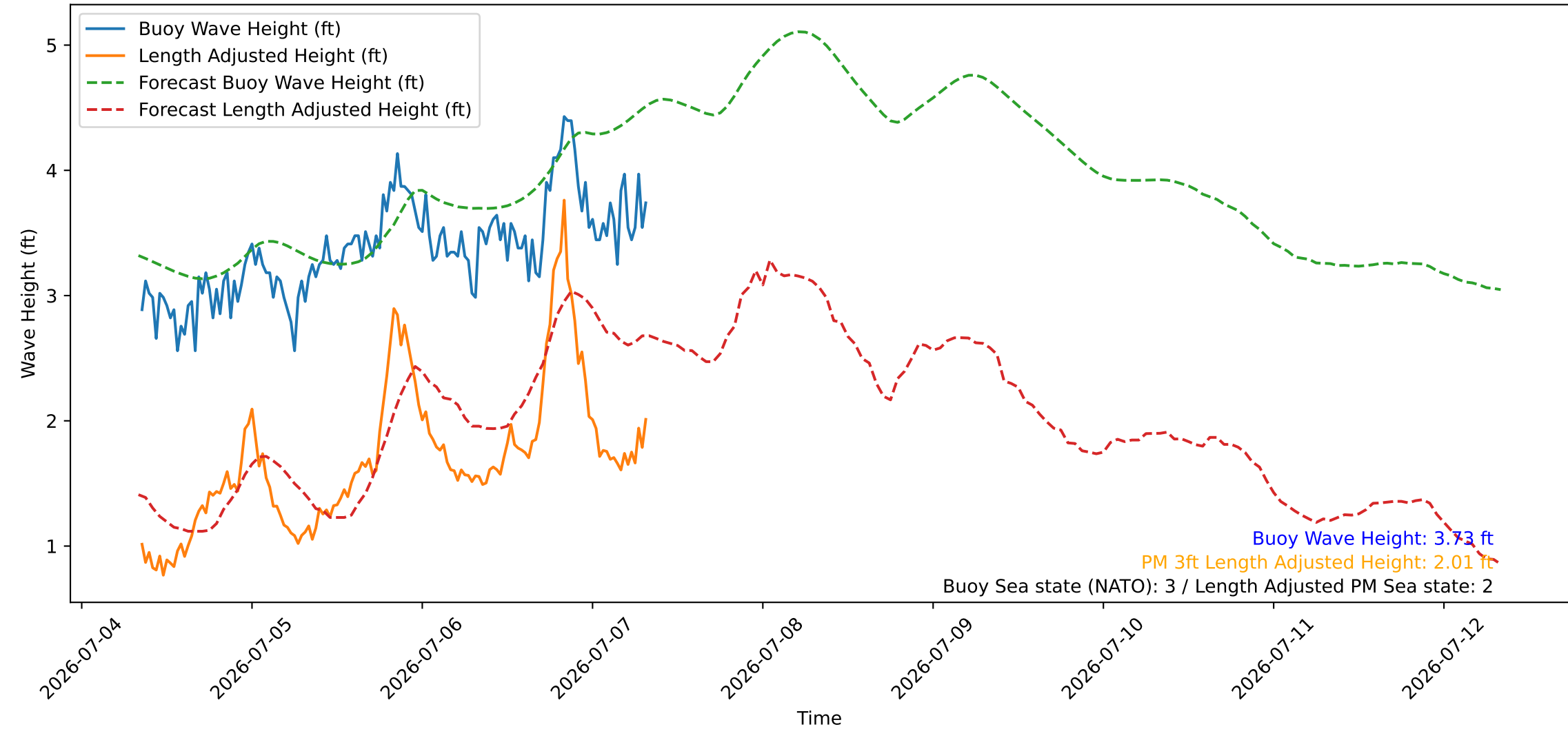
Wave Heights over Time for Green Beach at 2026-07-07 08:21:10
