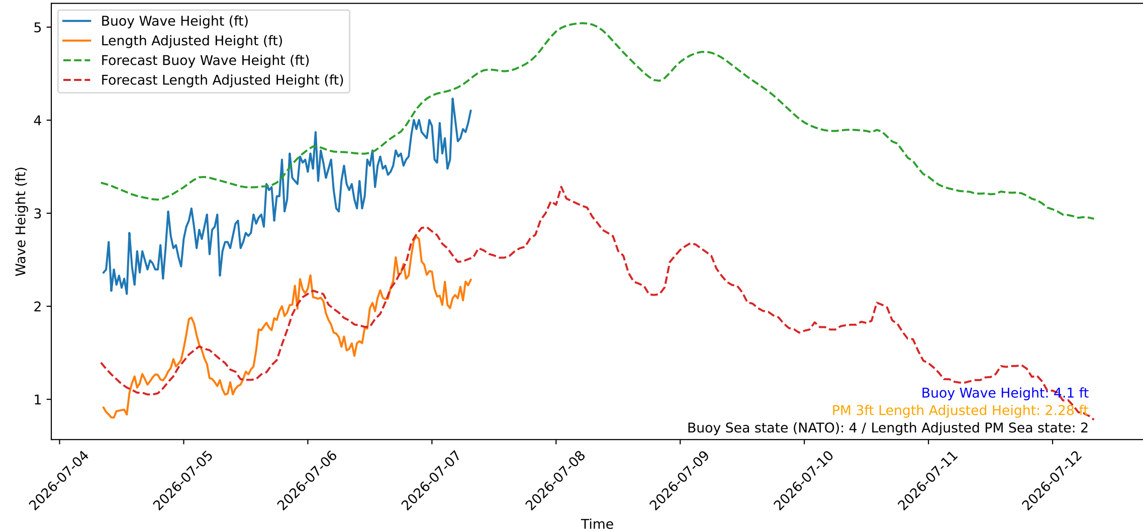
Wave Heights over Time for Oceanside Harbor at 2026-07-07 08:20:27
