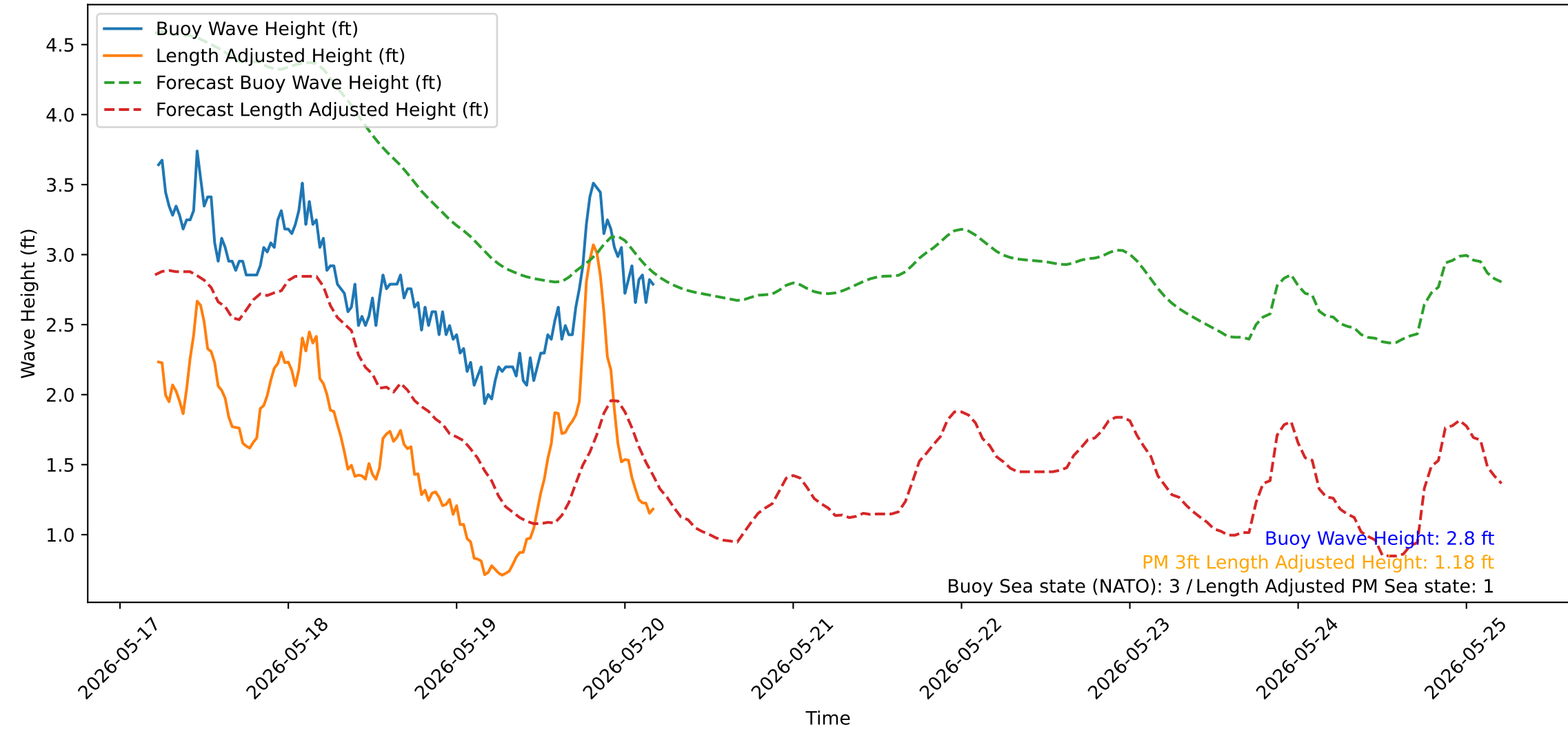
Wave Heights over Time for Red Beach at 2026-05-20 05:00:51
