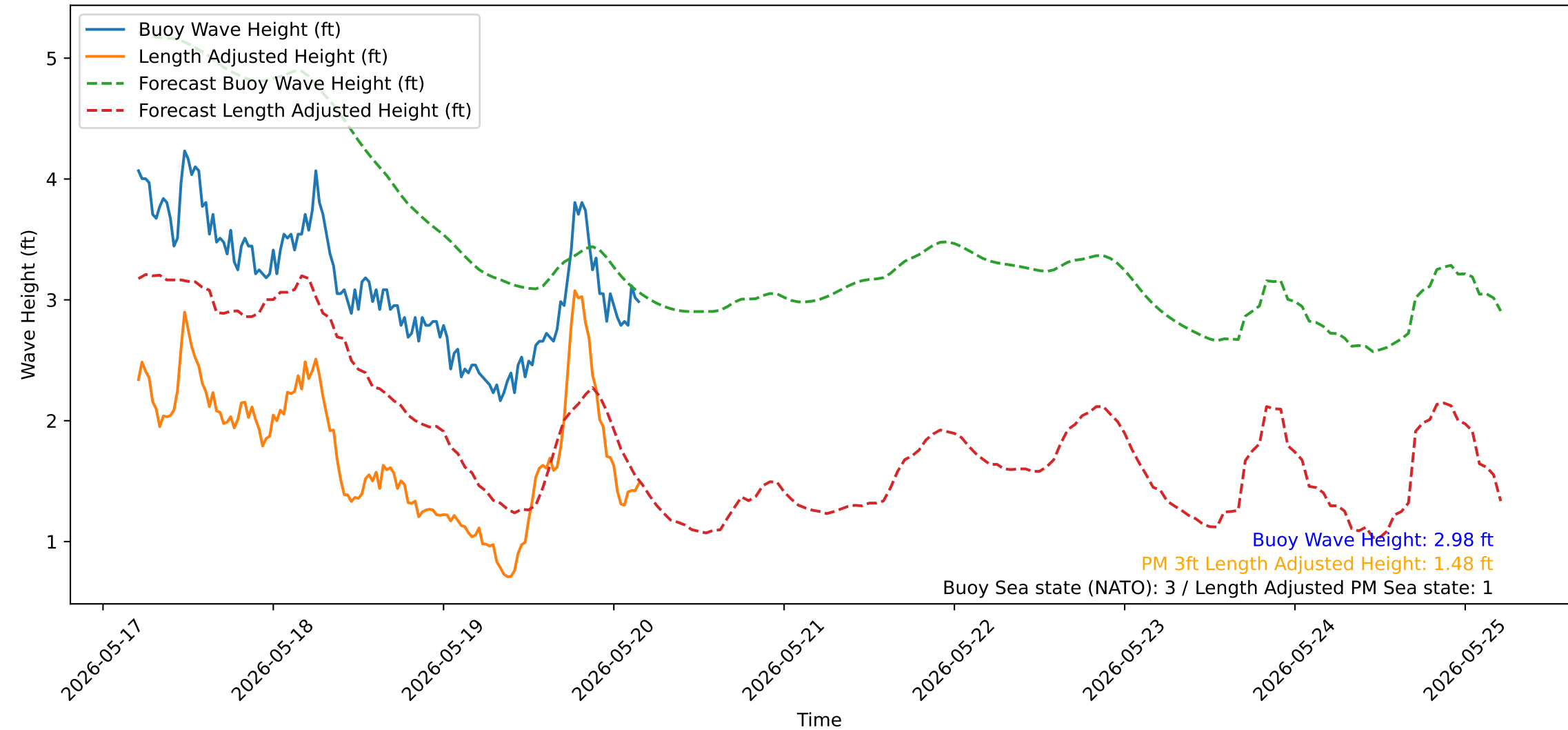
Wave Heights over Time for Green Beach at 2026-05-20 05:01:13
