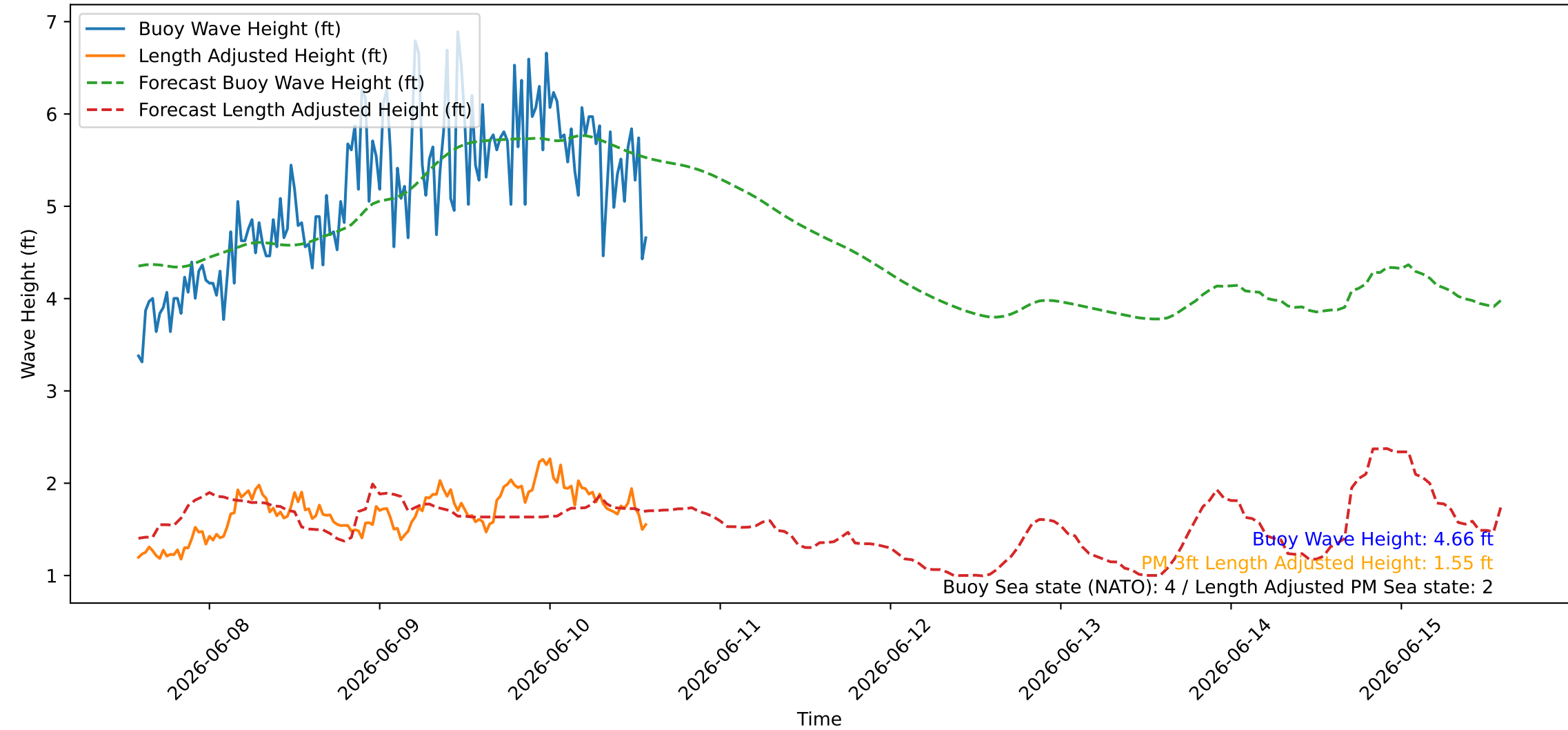
Wave Heights over Time for Green Beach at 2026-06-10 14:11:10
