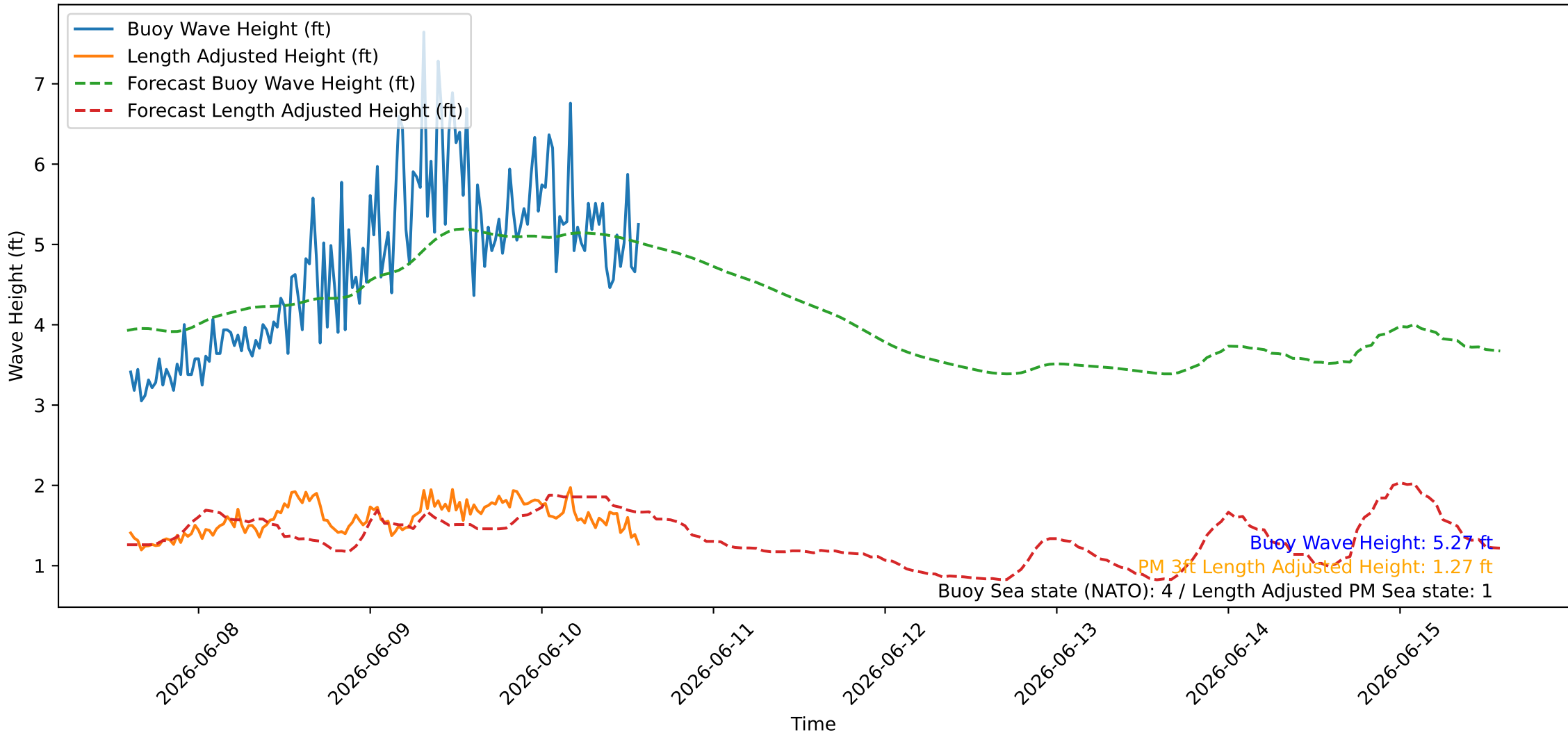
Wave Heights over Time for Red Beach at 2026-06-10 14:10:46
