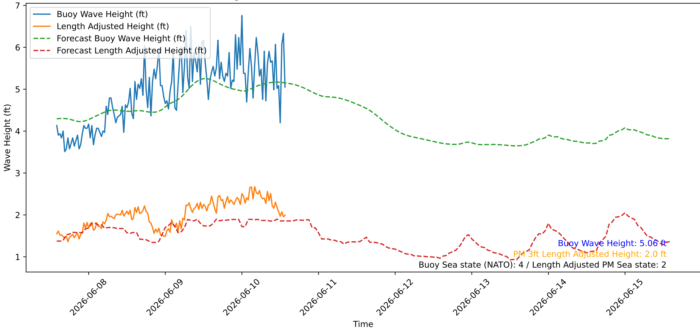
Wave Heights over Time for Oceanside Harbor at 2026-06-10 14:10:27
