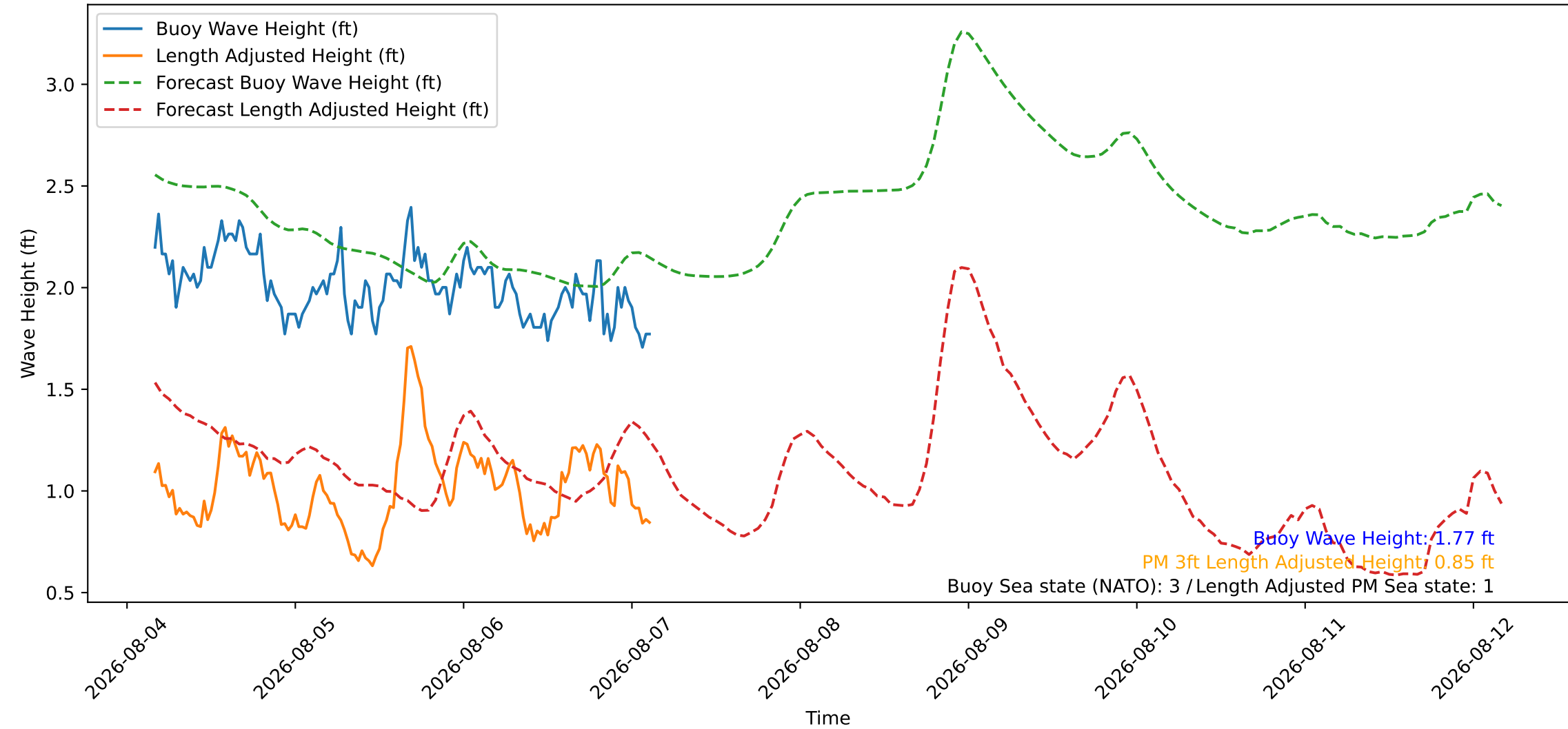
Wave Heights over Time for Red Beach at 2026-08-07 03:40:45
