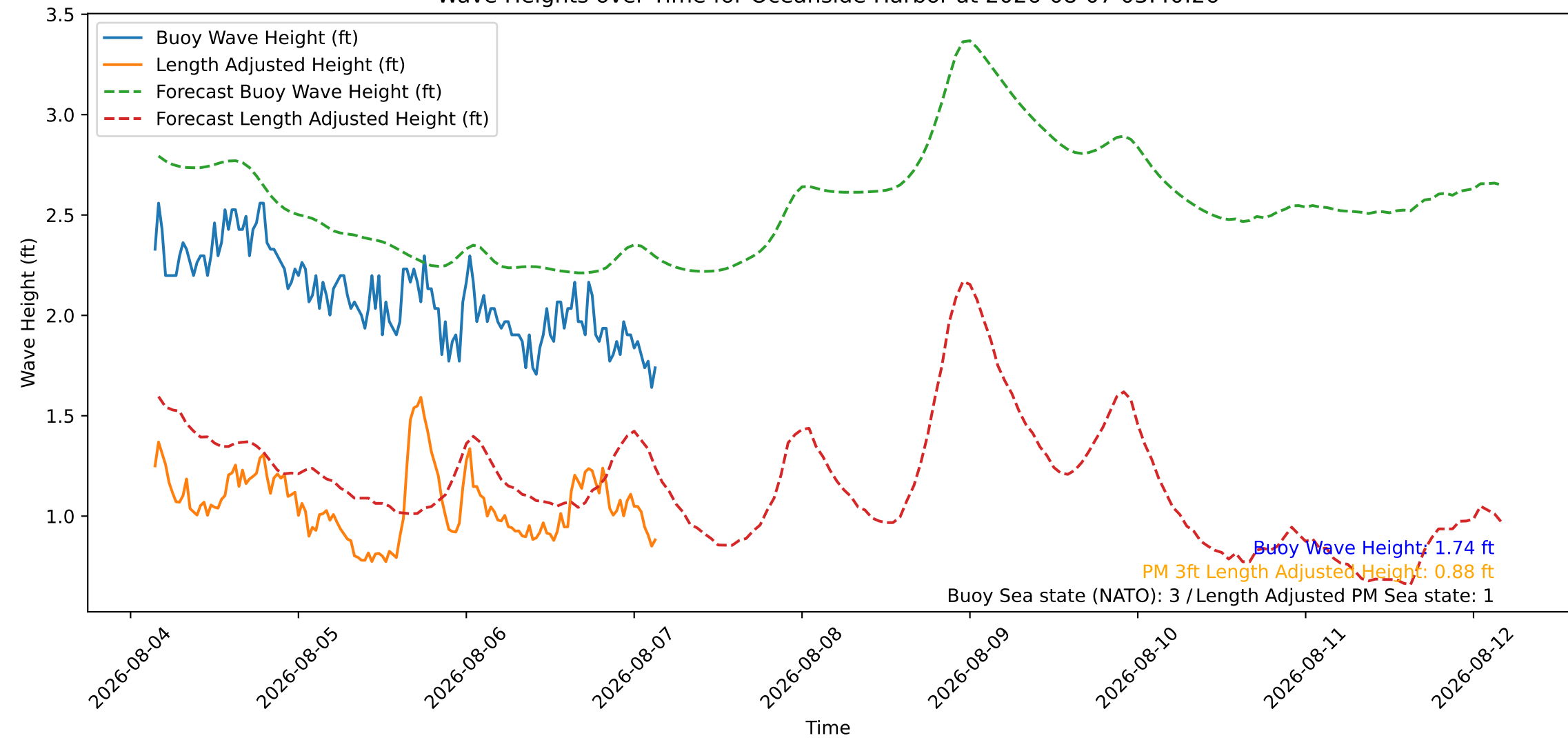
Wave Heights over Time for Oceanside Harbor at 2026-08-07 03:40:26
