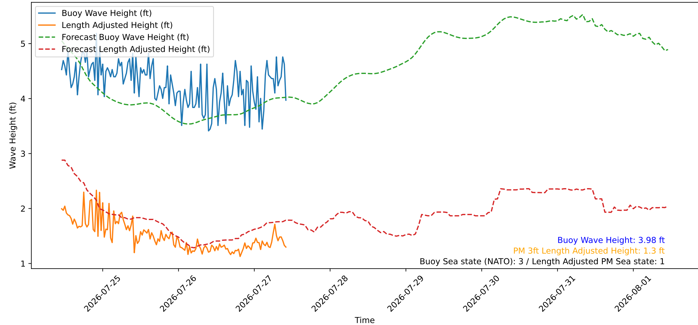
Wave Heights over Time for Green Beach at 2026-07-27 10:51:10
