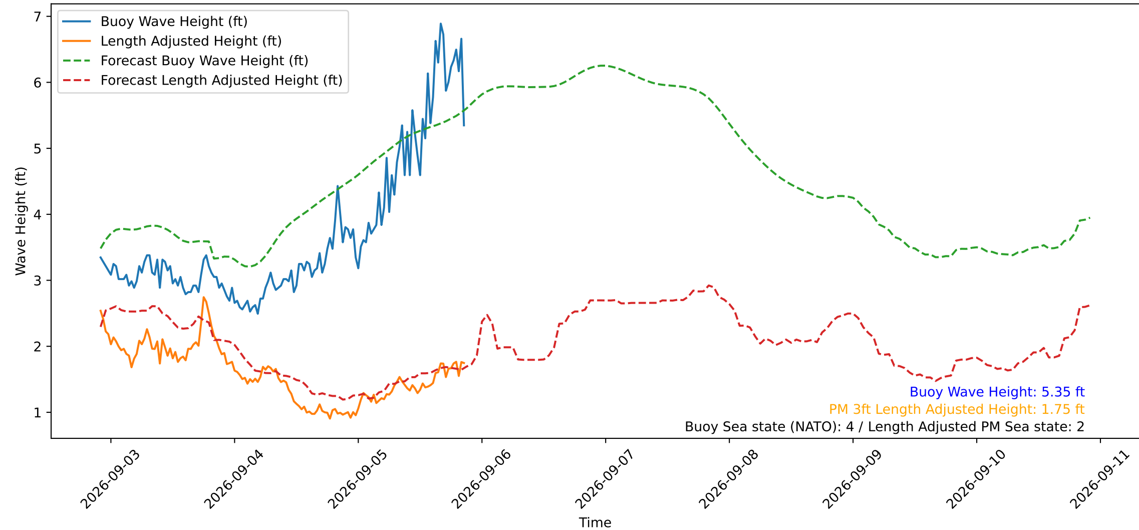
Wave Heights over Time for Green Beach at 2026-09-05 21:31:12
