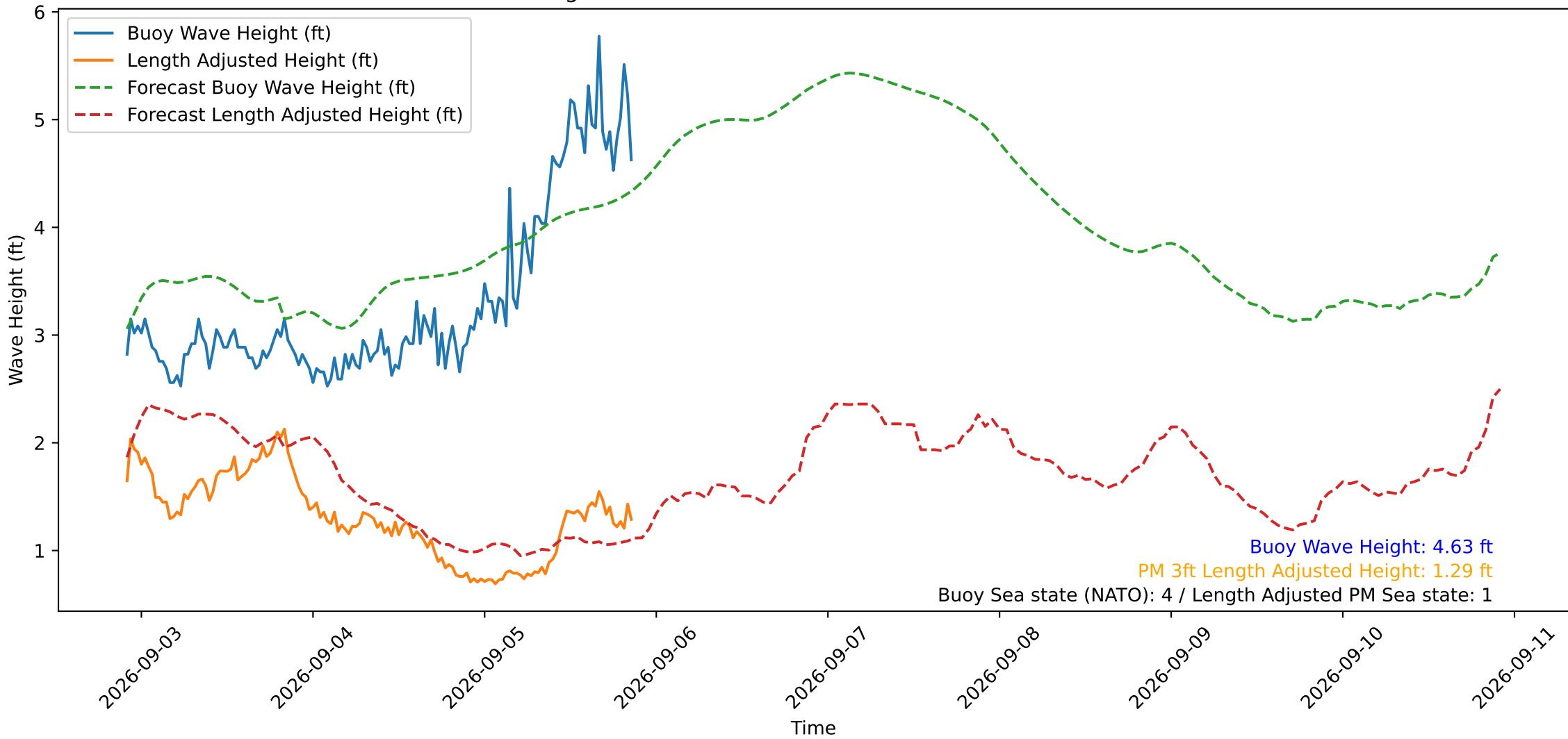
Wave Heights over Time for Red Beach at 2026-09-05 21:30:49
