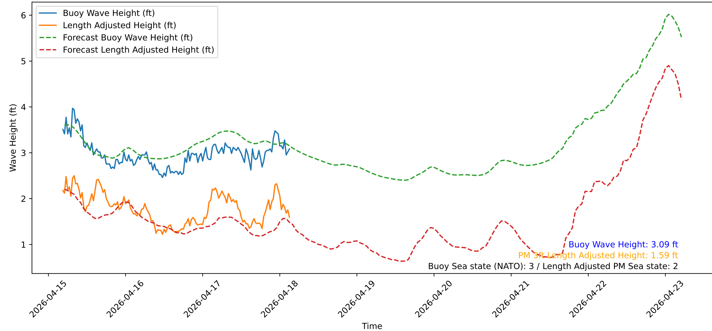
Wave Heights over Time for Green Beach at 2026-04-18 04:31:11
