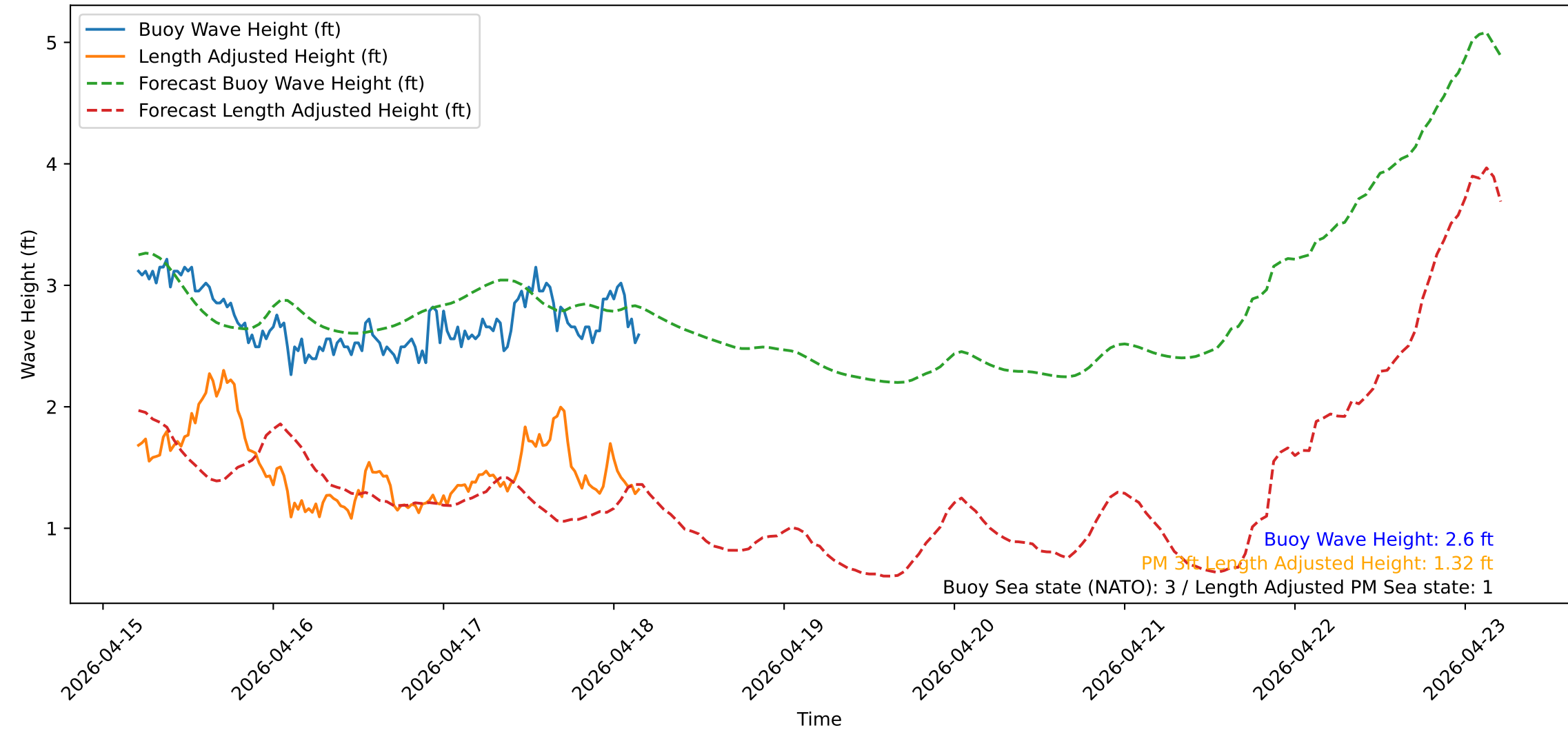
Wave Heights over Time for Red Beach at 2026-04-18 04:30:50
