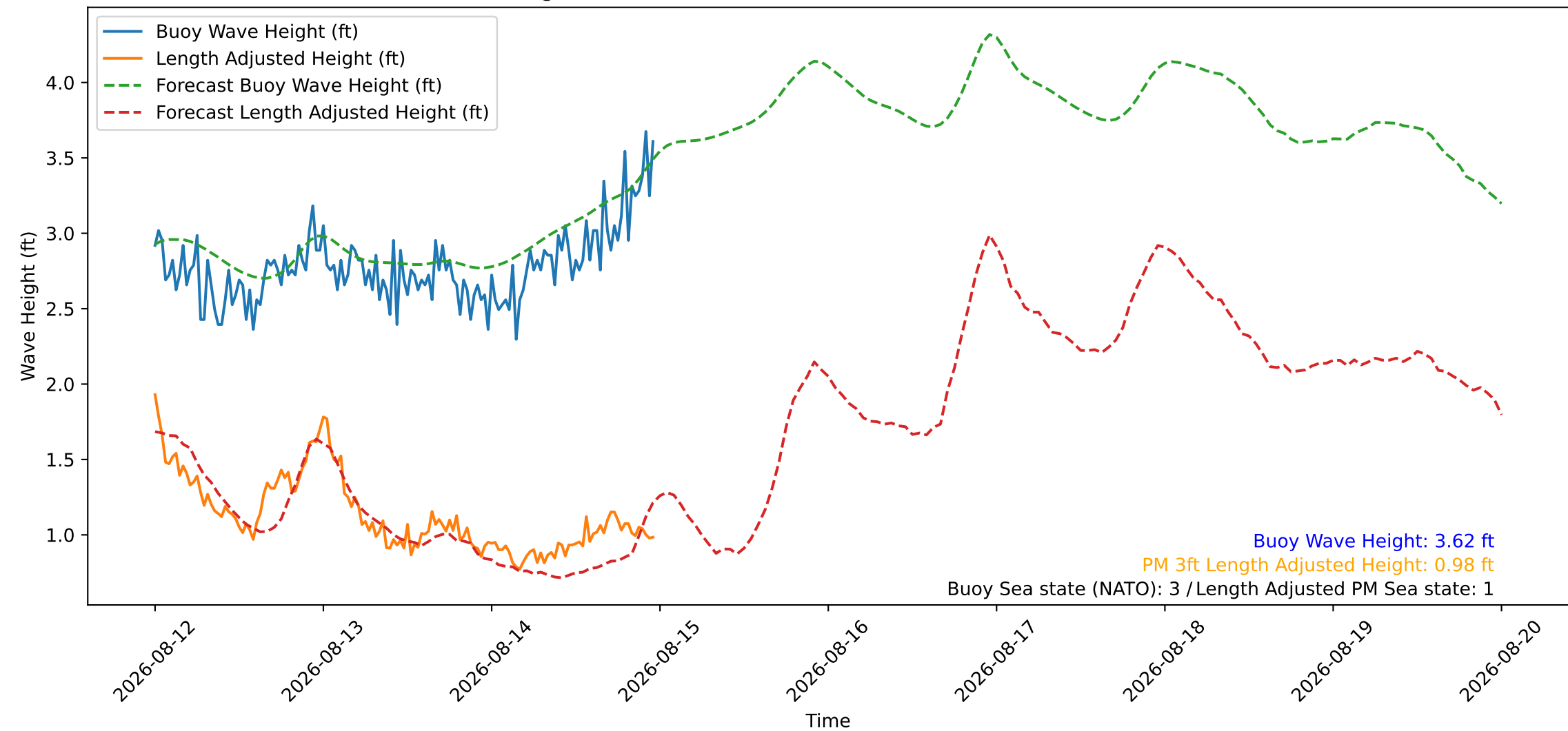
Wave Heights over Time for Oceanside Harbor at 2026-08-14 23:50:26
