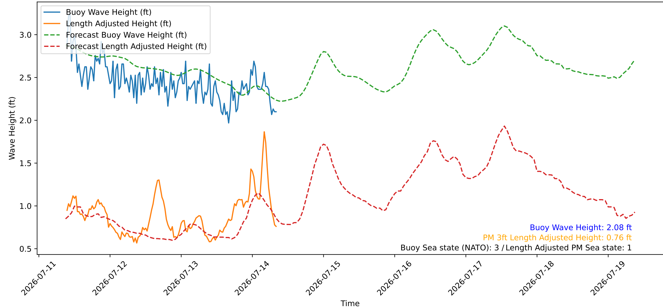
Wave Heights over Time for Red Beach at 2026-07-14 09:00:46
