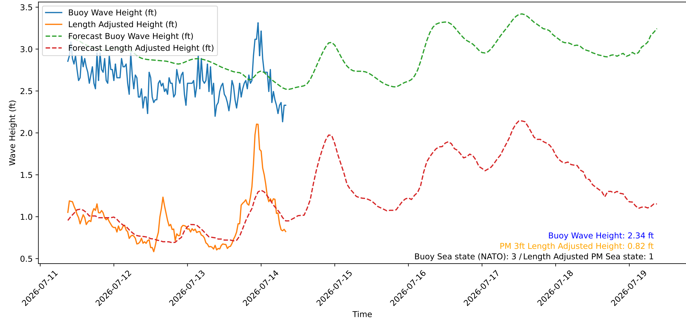
Wave Heights over Time for Green Beach at 2026-07-14 09:01:08
