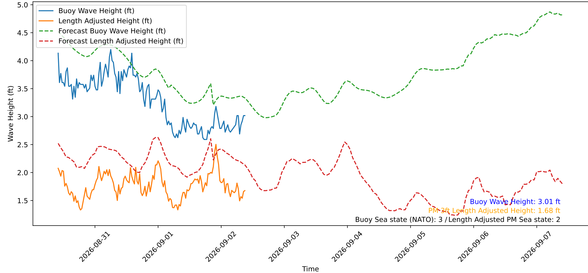
Wave Heights over Time for Red Beach at 2026-09-02 09:50:51
