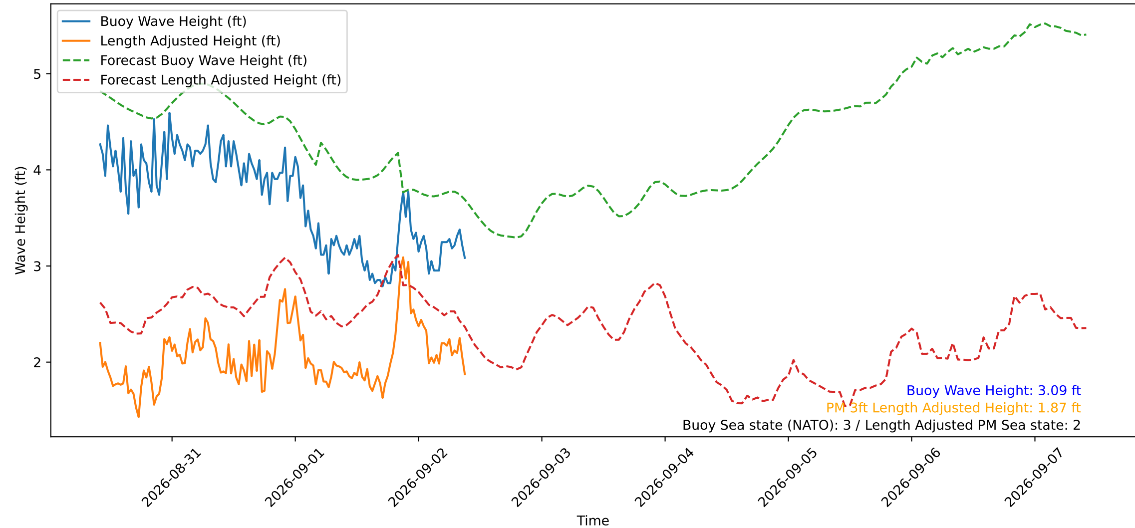
Wave Heights over Time for Green Beach at 2026-09-02 09:51:15
