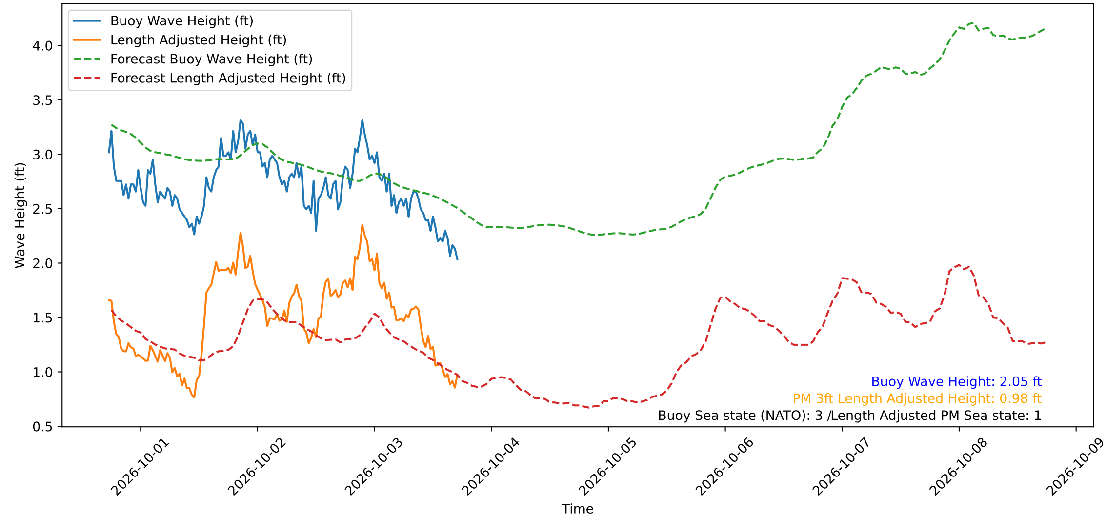
Wave Heights over Time for Oceanside Harbor at 2026-10-03 17:40:30
