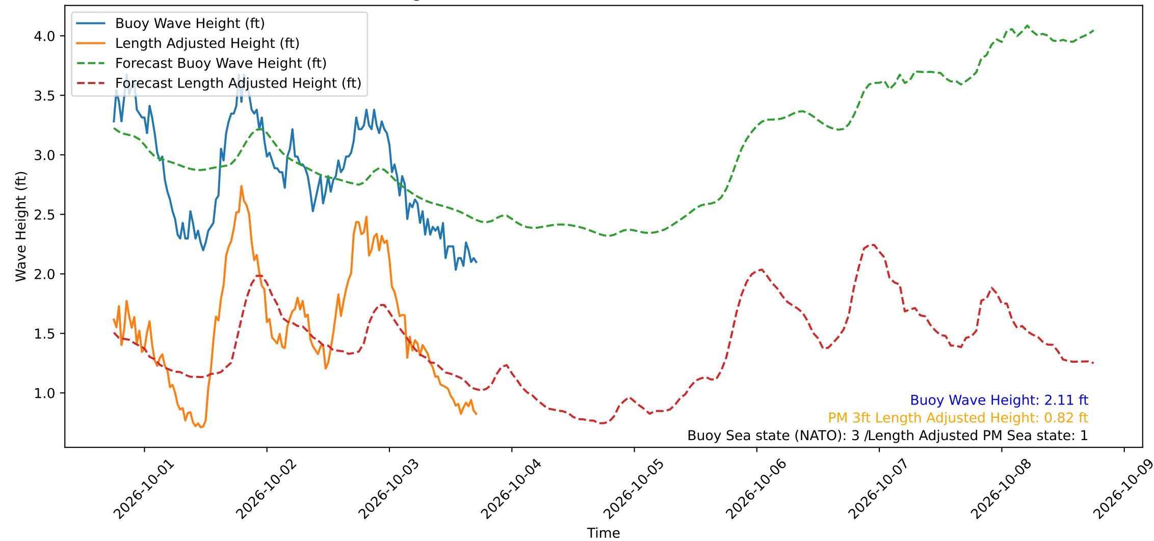
Wave Heights over Time for Green Beach at 2026-10-03 17:41:13
