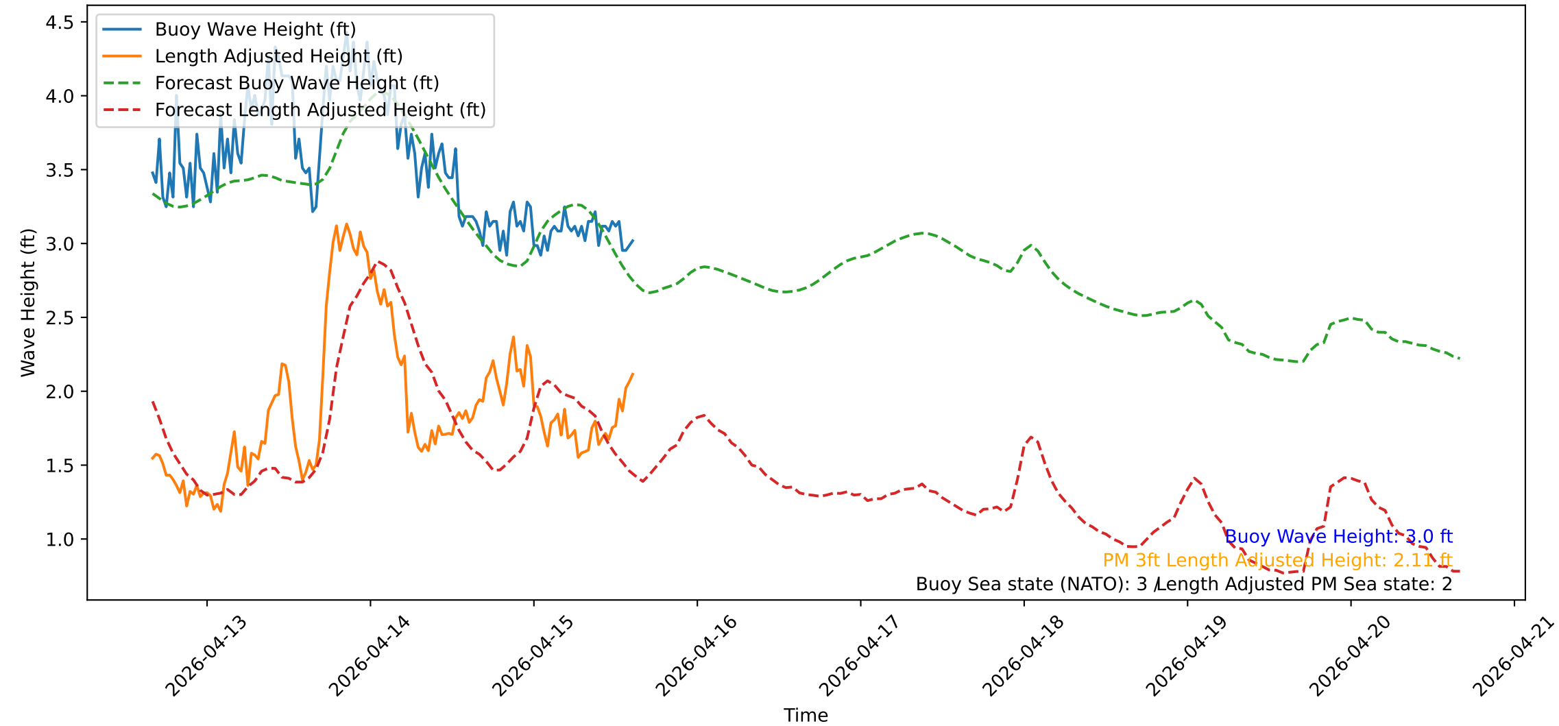
Wave Heights over Time for Red Beach at 2026-04-15 15:30:51
