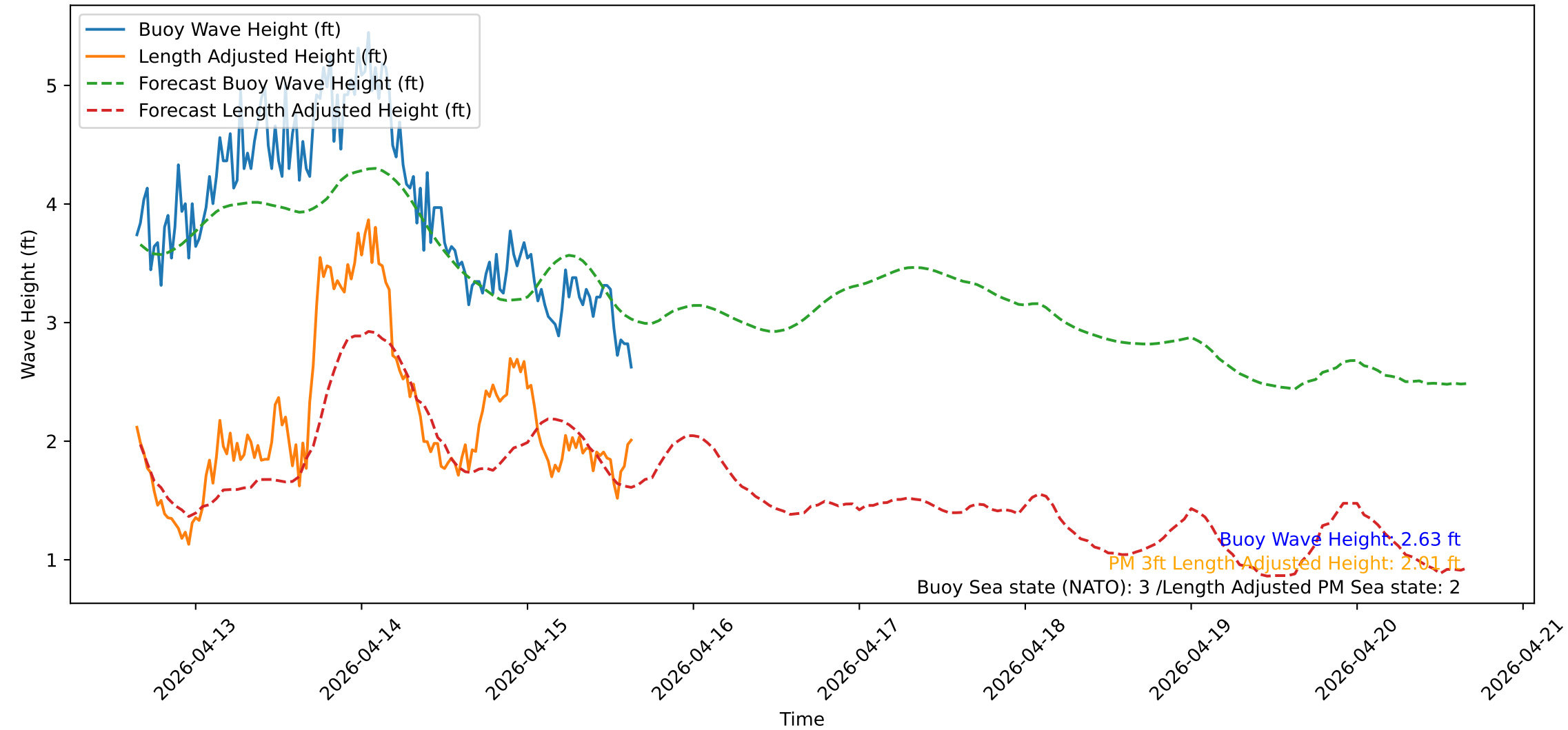
Wave Heights over Time for Oceanside Harbor at 2026-04-15 15:30:32
