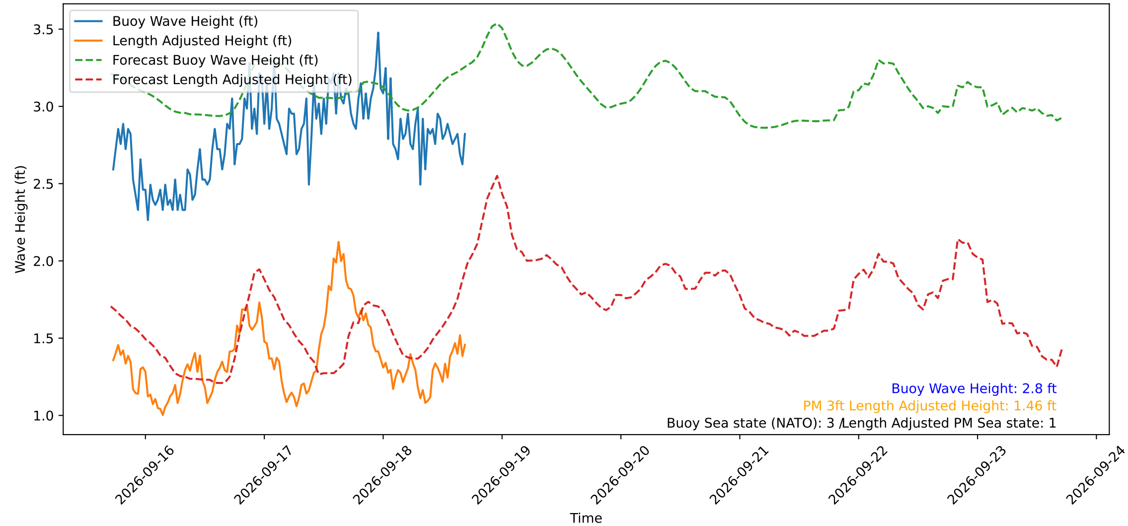
Wave Heights over Time for Green Beach at 2026-09-18 17:21:19
