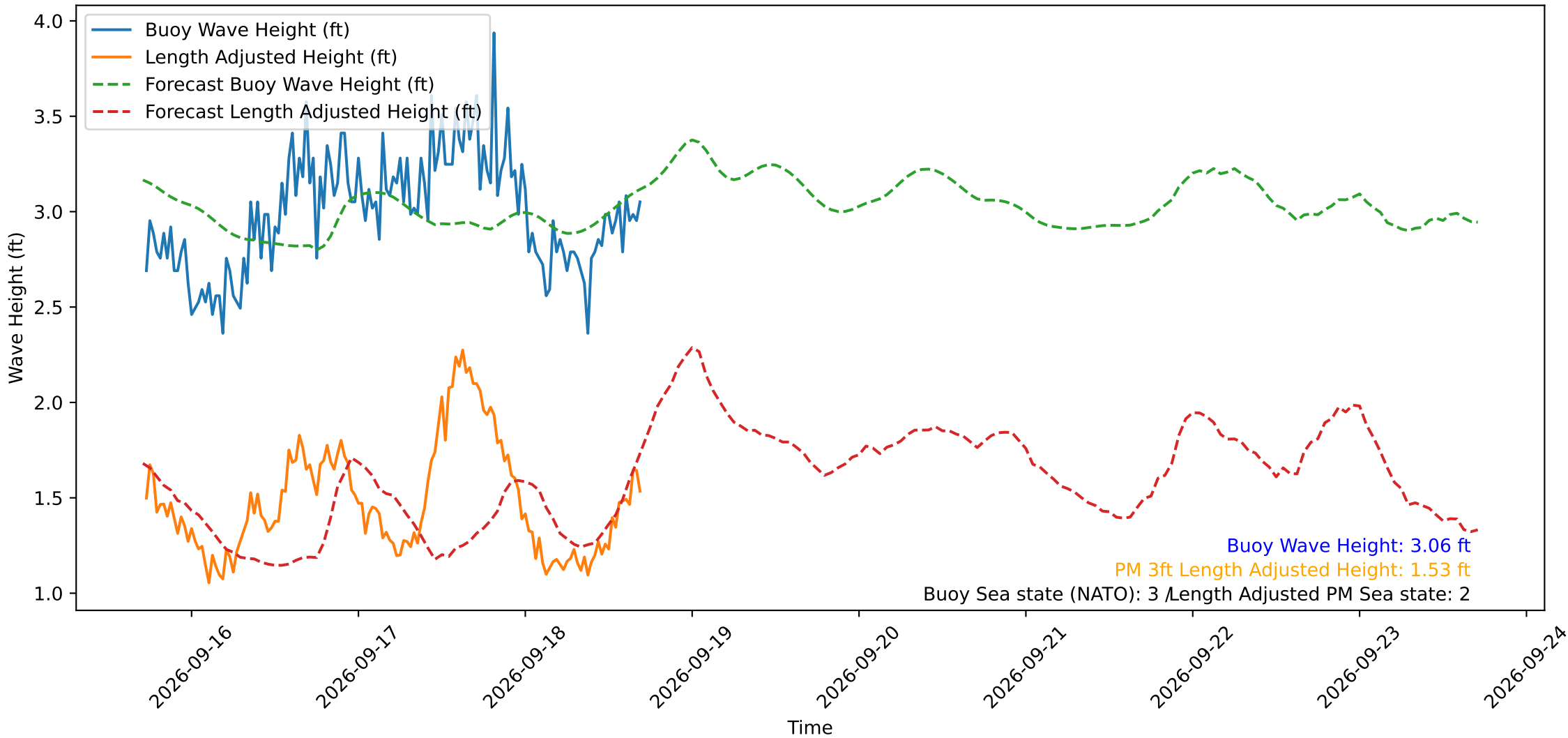
Wave Heights over Time for Oceanside Harbor at 2026-09-18 17:20:31
