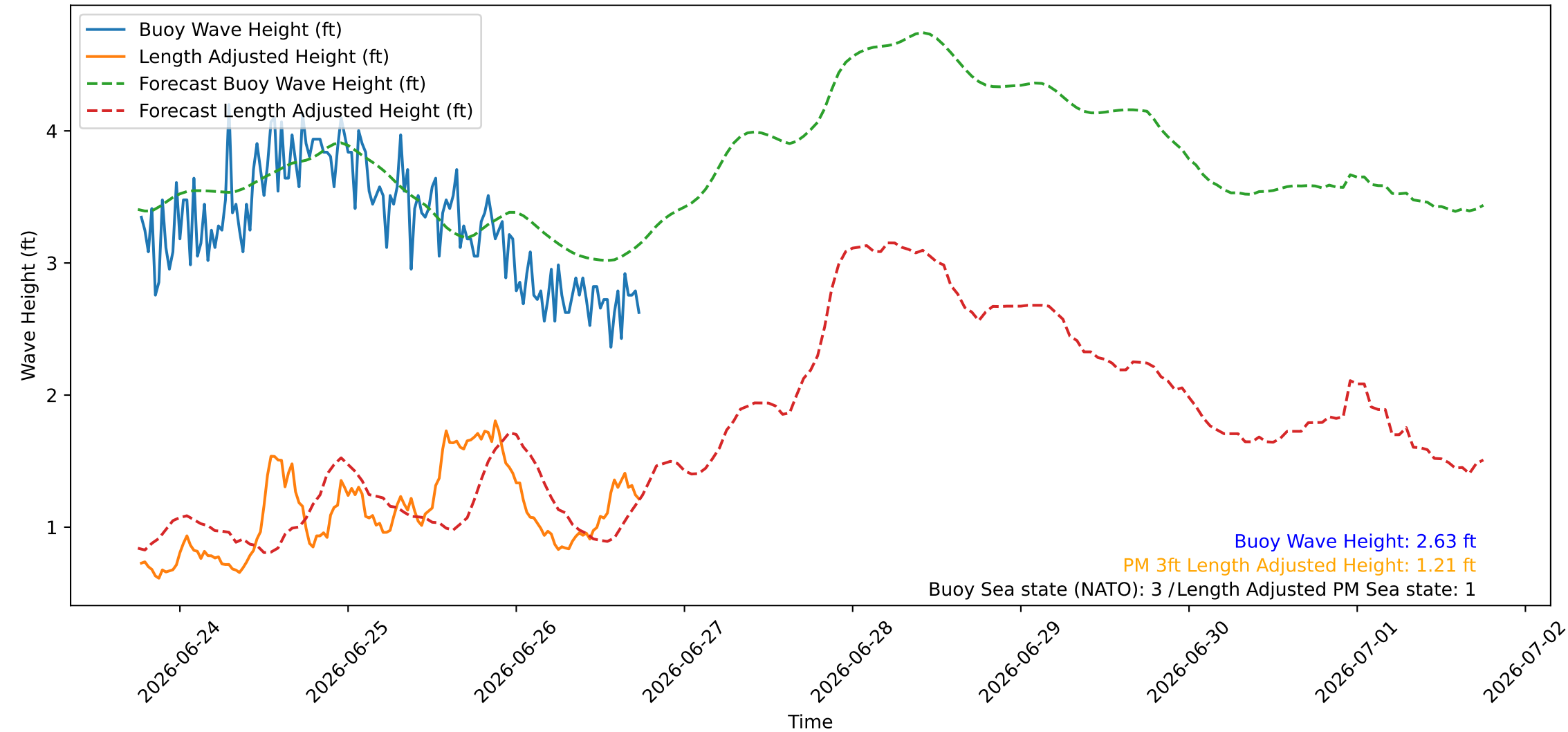
Wave Heights over Time for Green Beach at 2026-06-26 18:21:09
