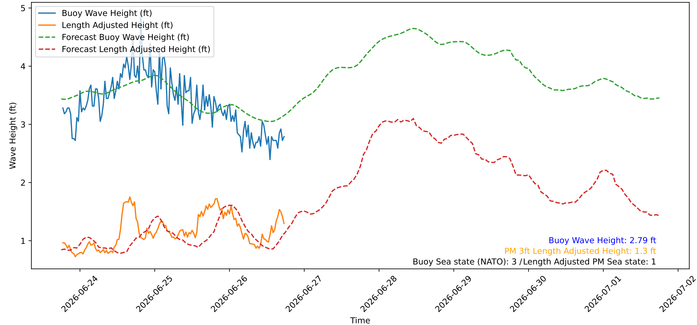
Wave Heights over Time for Oceanside Harbor at 2026-06-26 18:20:27
