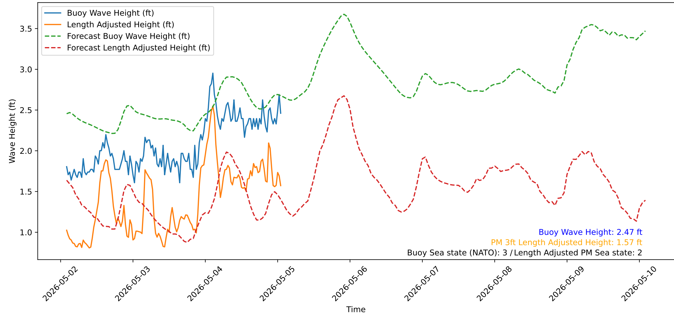
Wave Heights over Time for Red Beach at 2026-05-05 01:50:52
