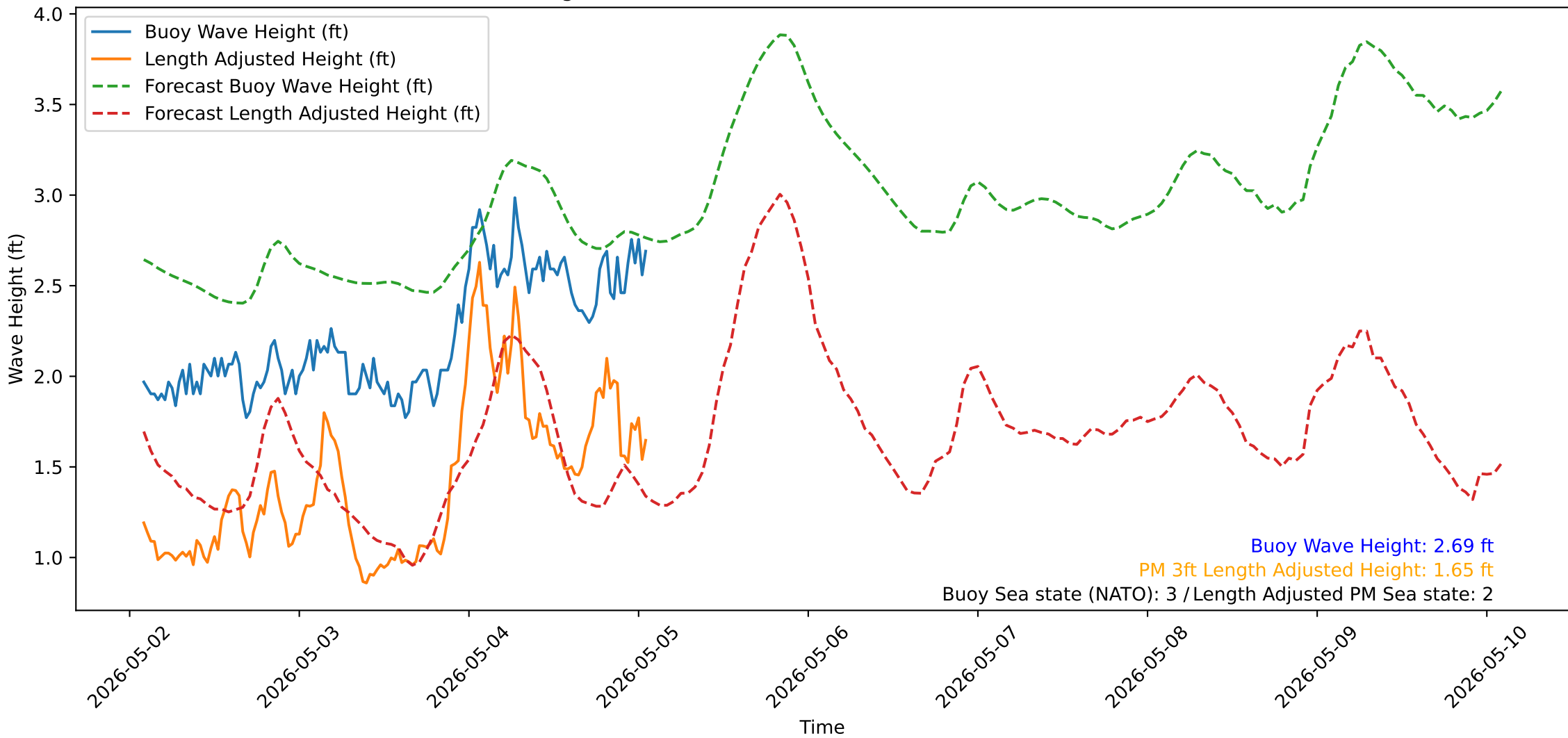
Wave Heights over Time for Green Beach at 2026-05-05 01:51:15
