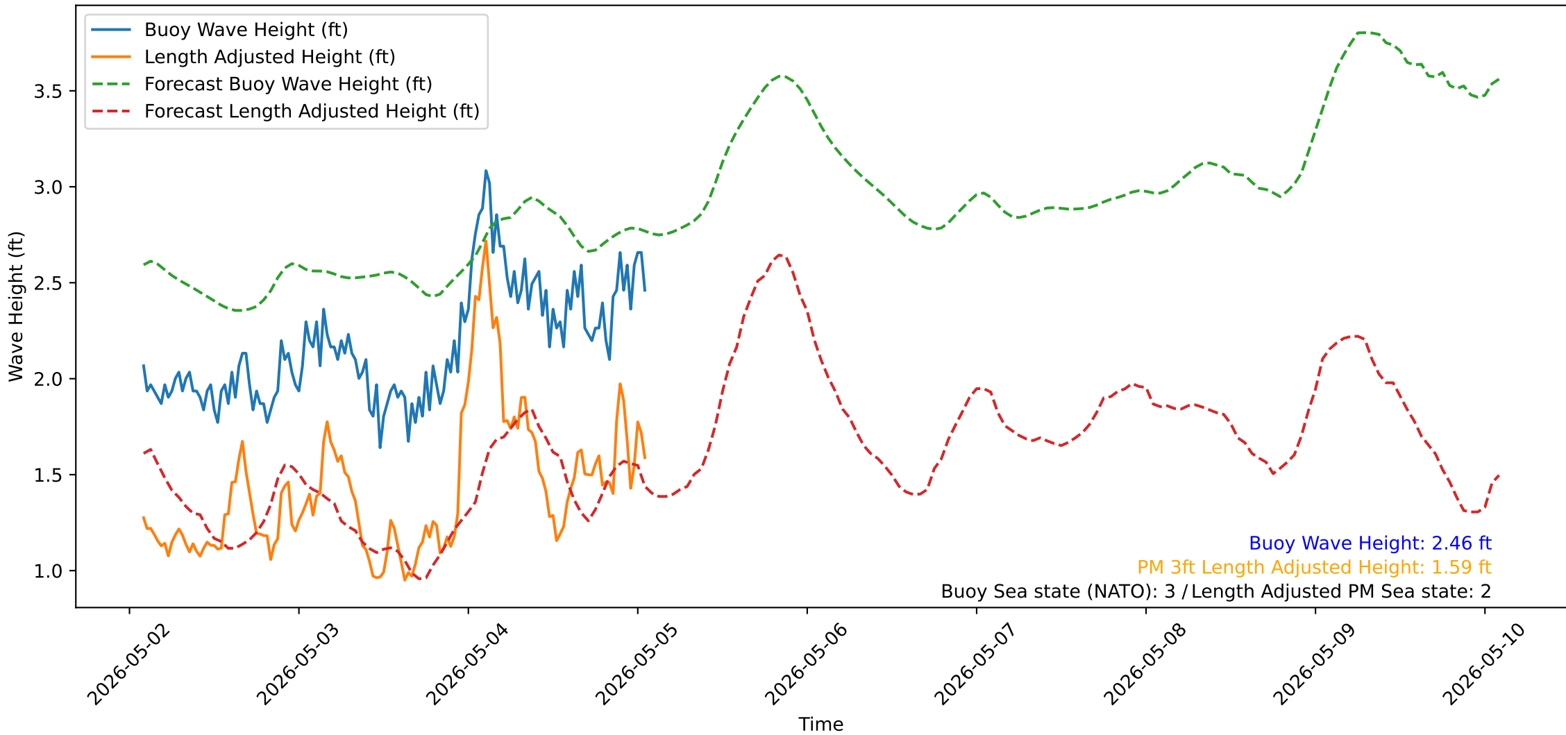
Wave Heights over Time for Oceanside Harbor at 2026-05-05 01:50:32
