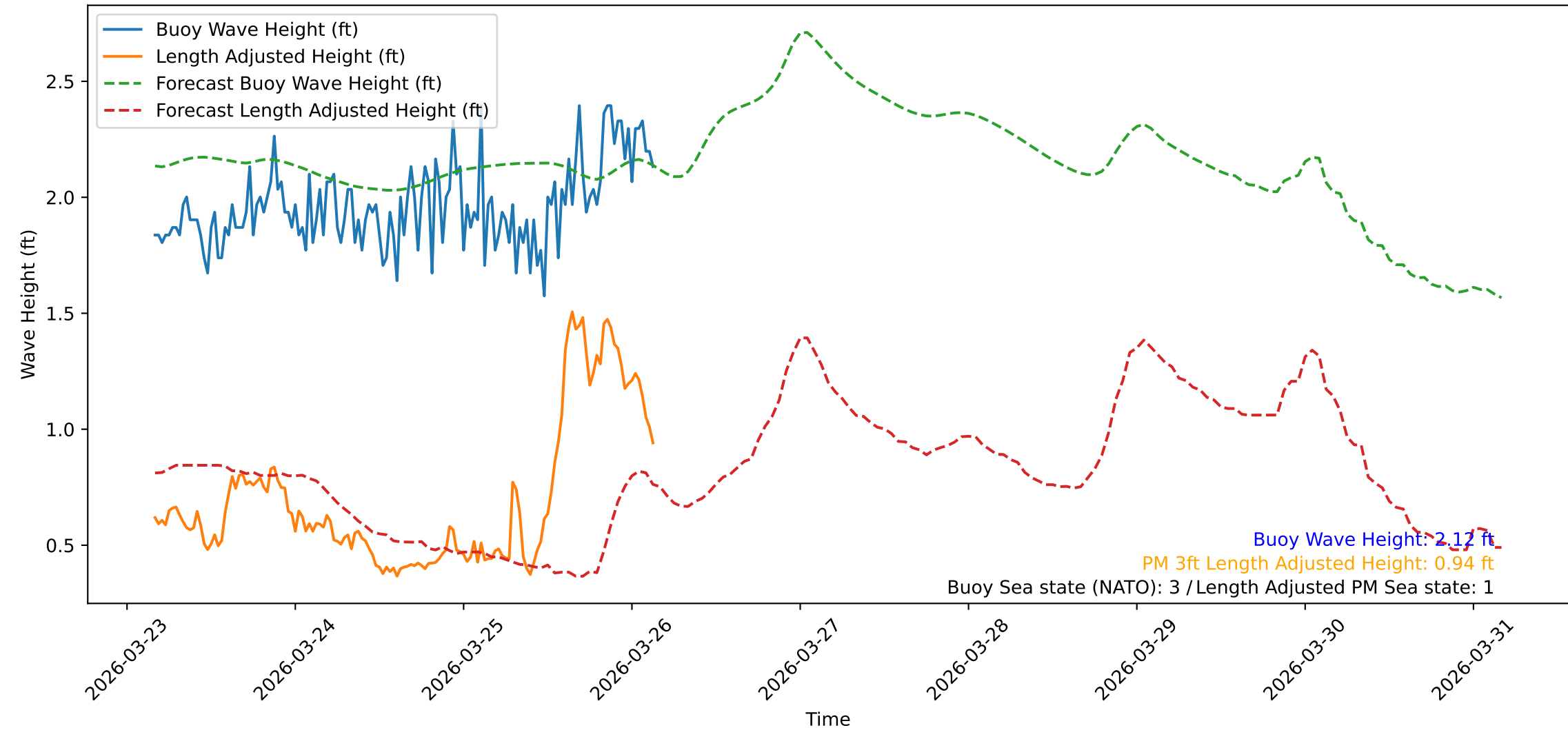
Wave Heights over Time for Red Beach at 2026-03-26 03:50:48
