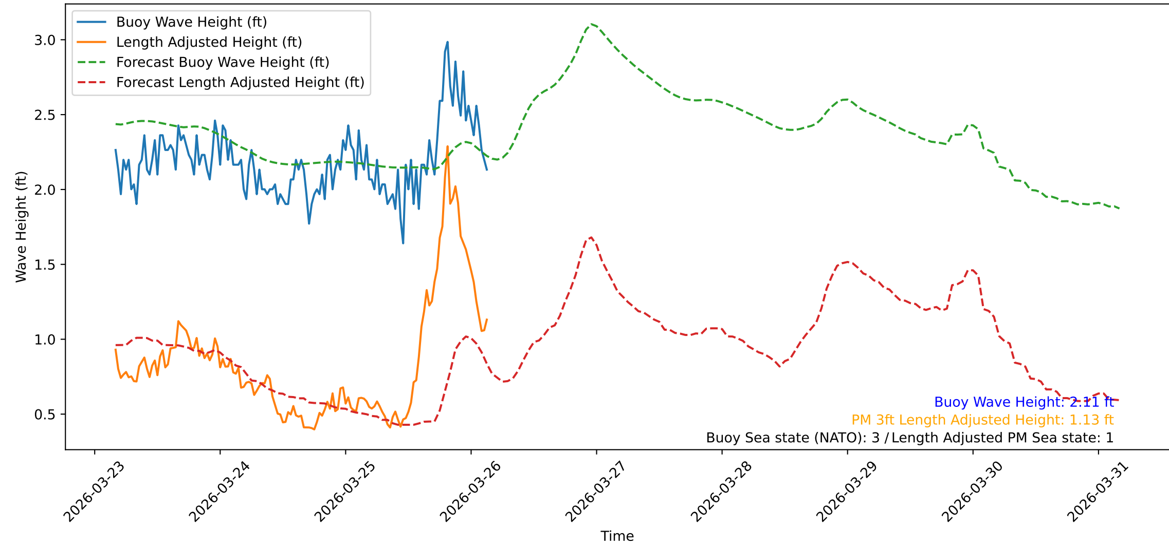
Wave Heights over Time for Green Beach at 2026-03-26 03:51:11
