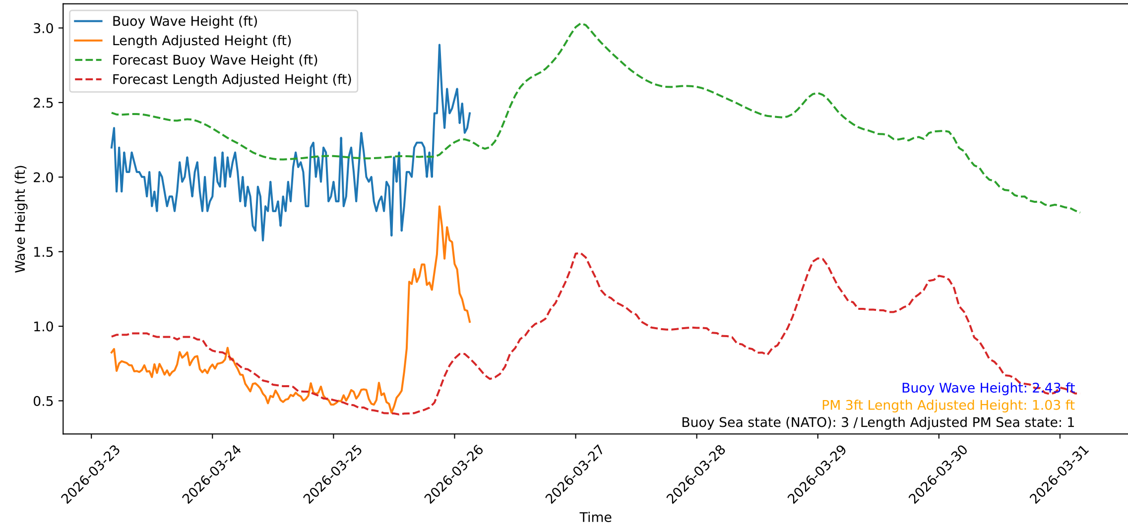
Wave Heights over Time for Oceanside Harbor at 2026-03-26 03:50:32
