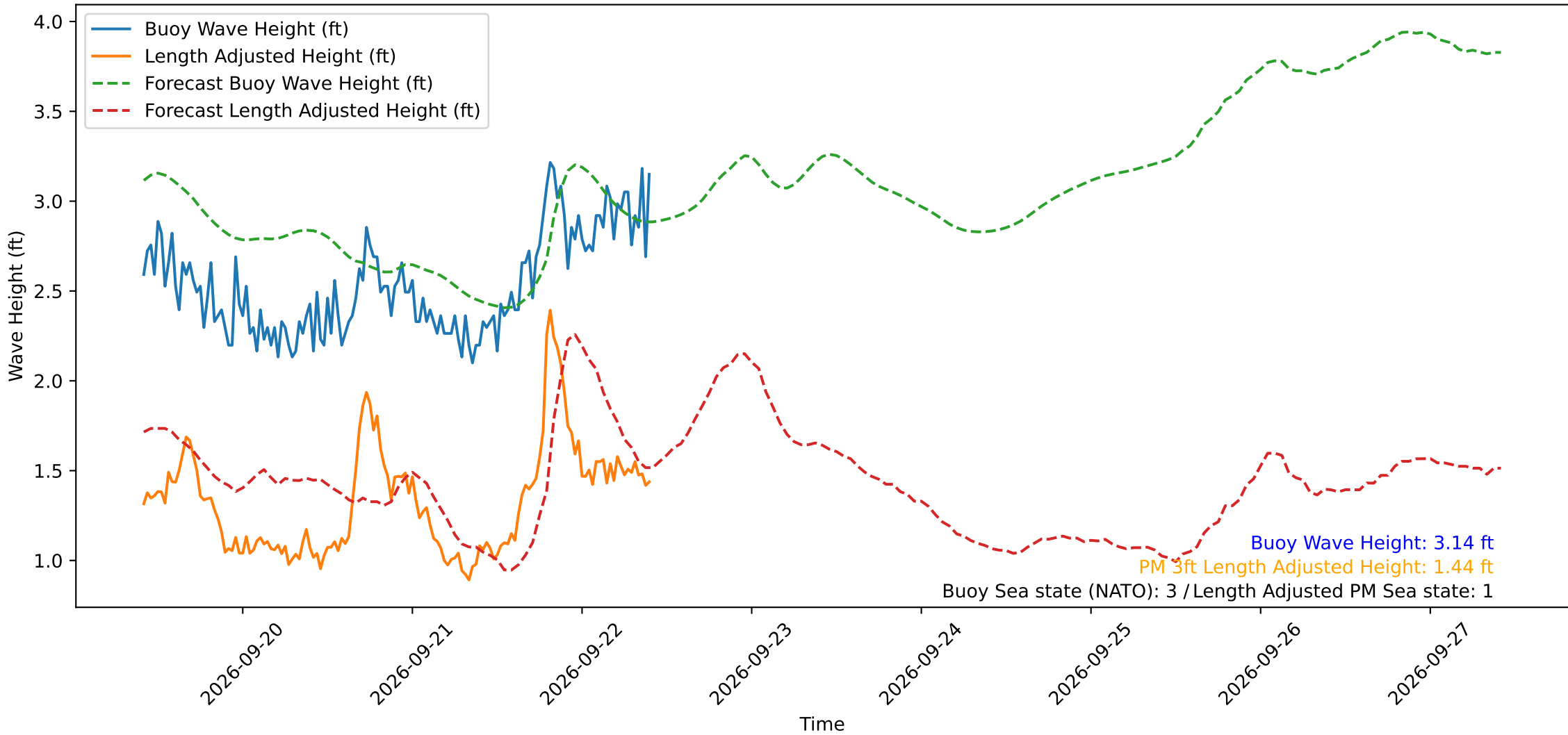
Wave Heights over Time for Oceanside Harbor at 2026-09-22 10:10:30
