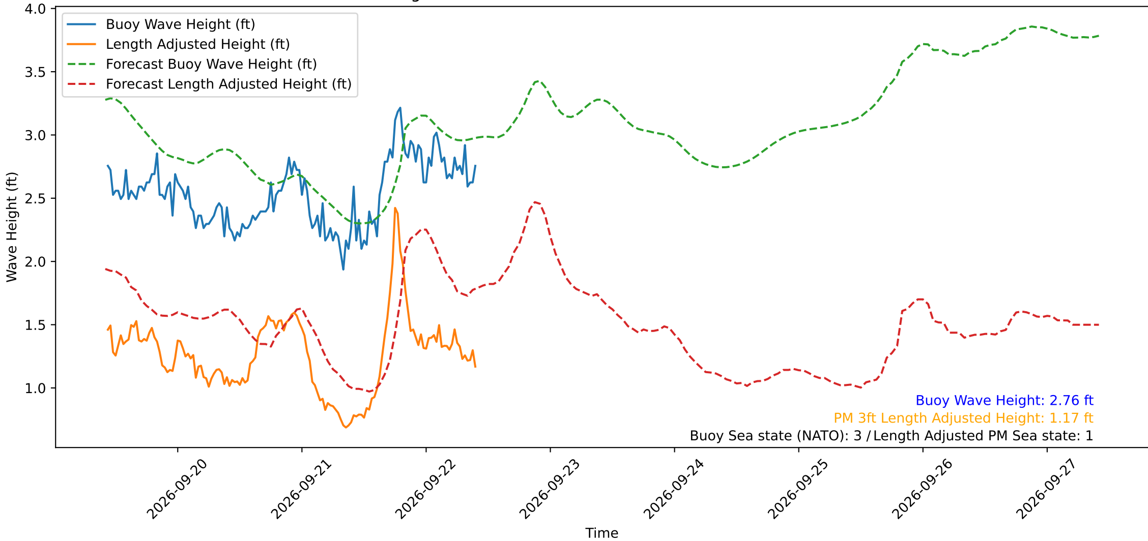
Wave Heights over Time for Green Beach at 2026-09-22 10:11:12
