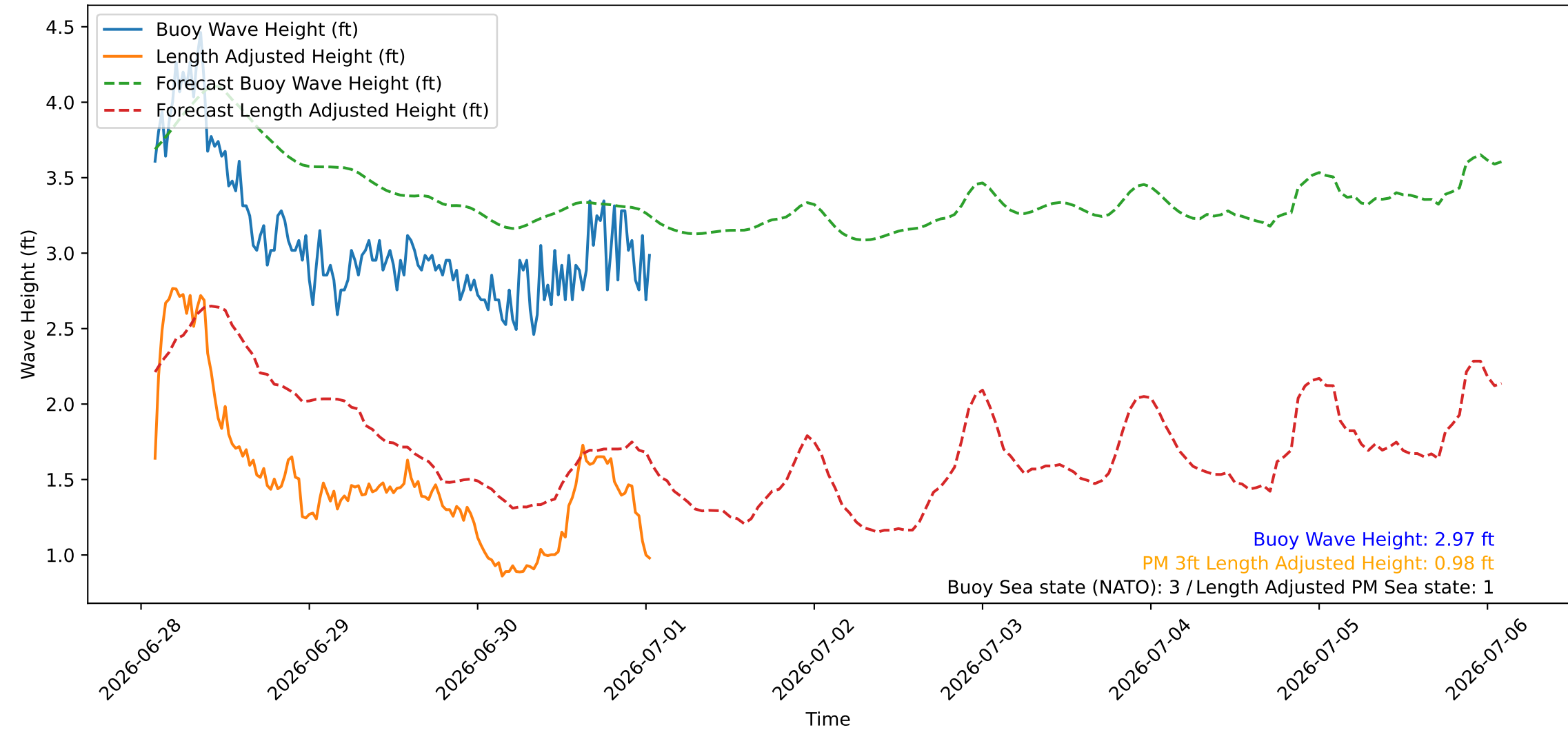
Wave Heights over Time for Red Beach at 2026-07-01 01:30:45
