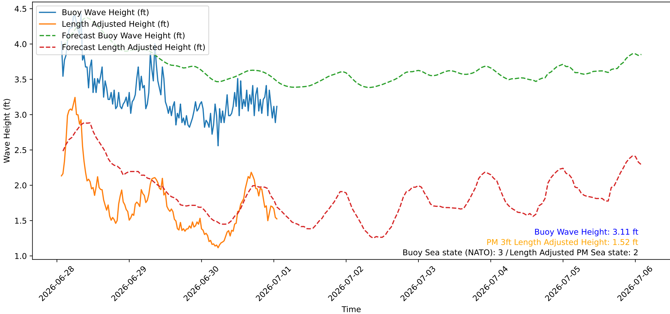
Wave Heights over Time for Oceanside Harbor at 2026-07-01 01:30:27
