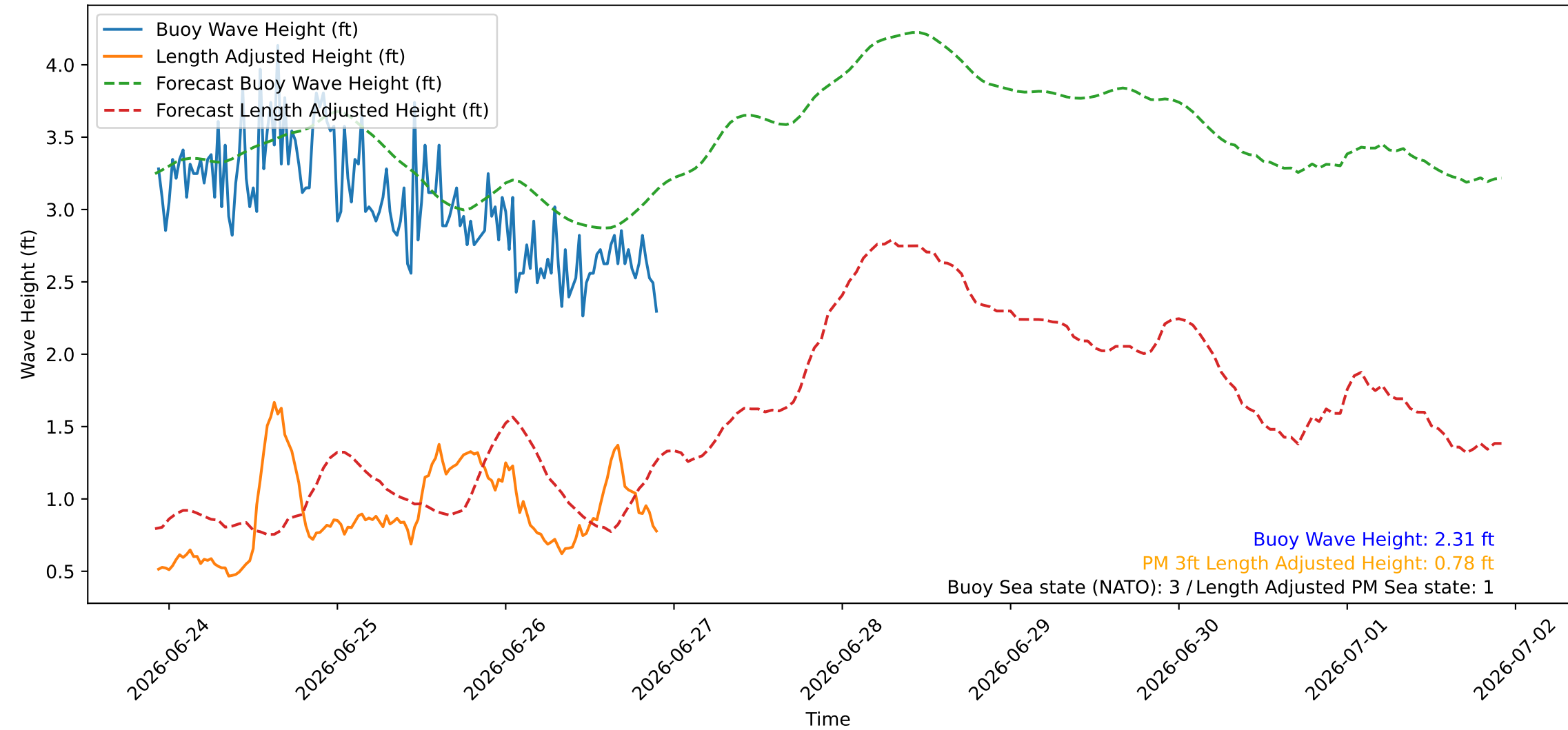
Wave Heights over Time for Red Beach at 2026-06-26 22:10:45
