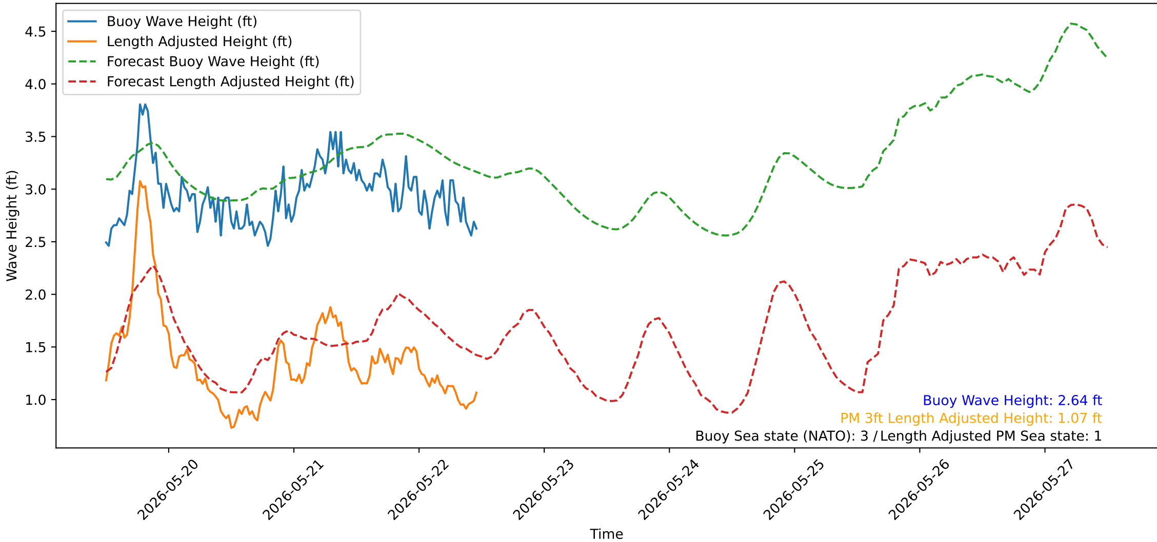
Wave Heights over Time for Green Beach at 2026-05-22 12:01:13
