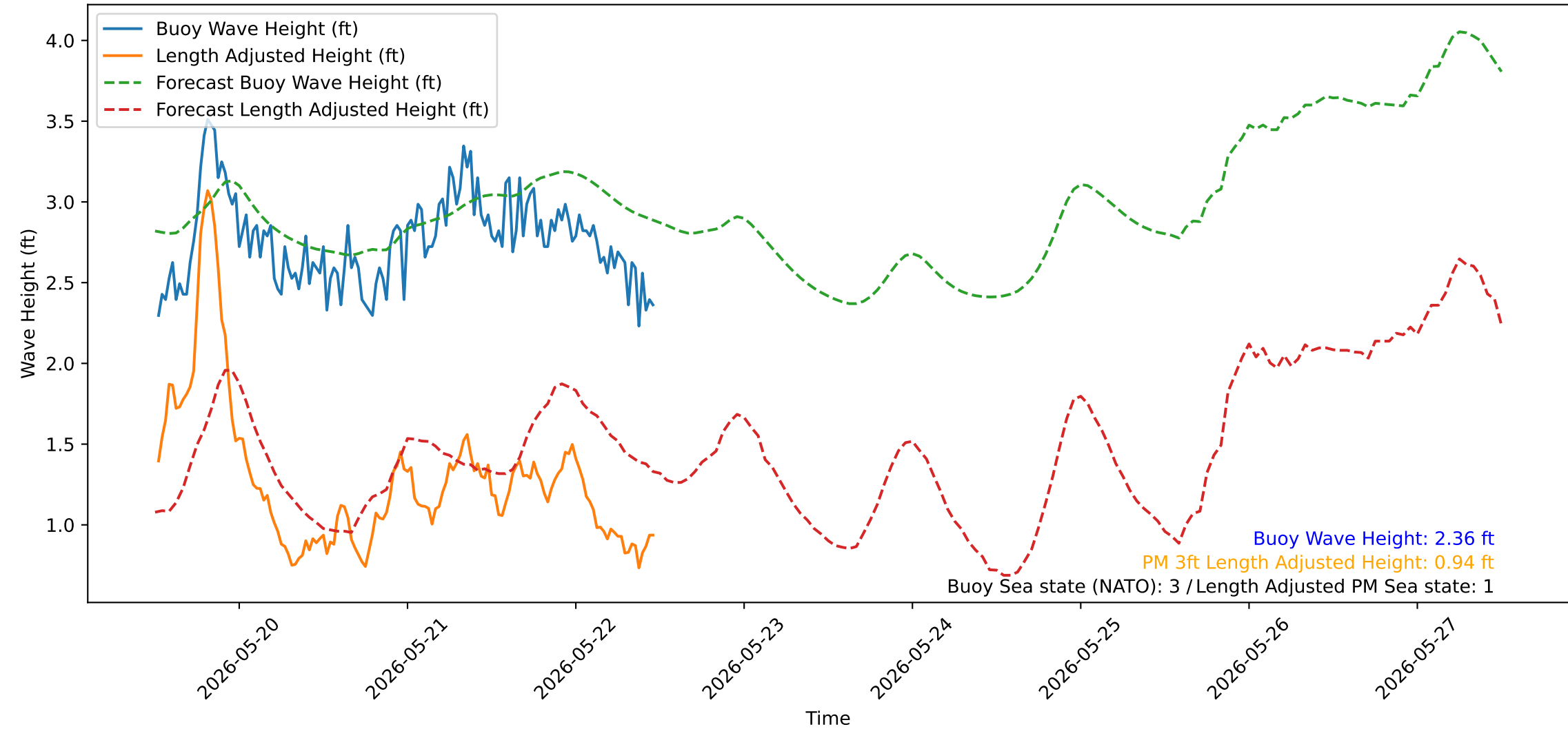
Wave Heights over Time for Red Beach at 2026-05-22 12:00:51
