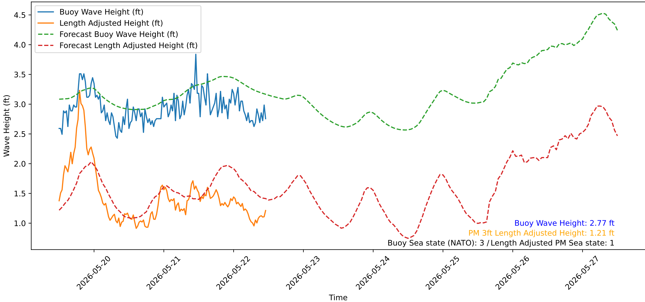
Wave Heights over Time for Oceanside Harbor at 2026-05-22 12:00:32
