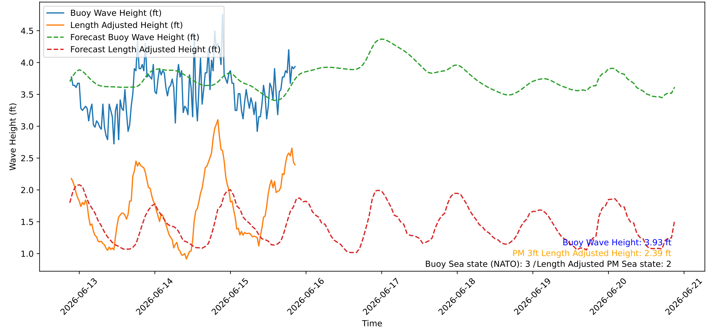
Wave Heights over Time for Red Beach at 2026-06-15 21:10:45
