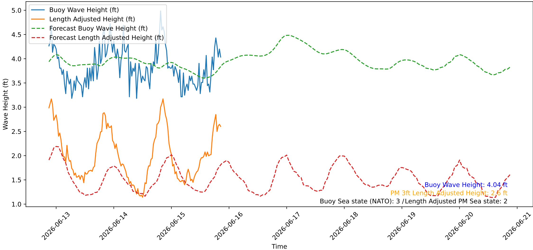
Wave Heights over Time for Oceanside Harbor at 2026-06-15 21:10:26
