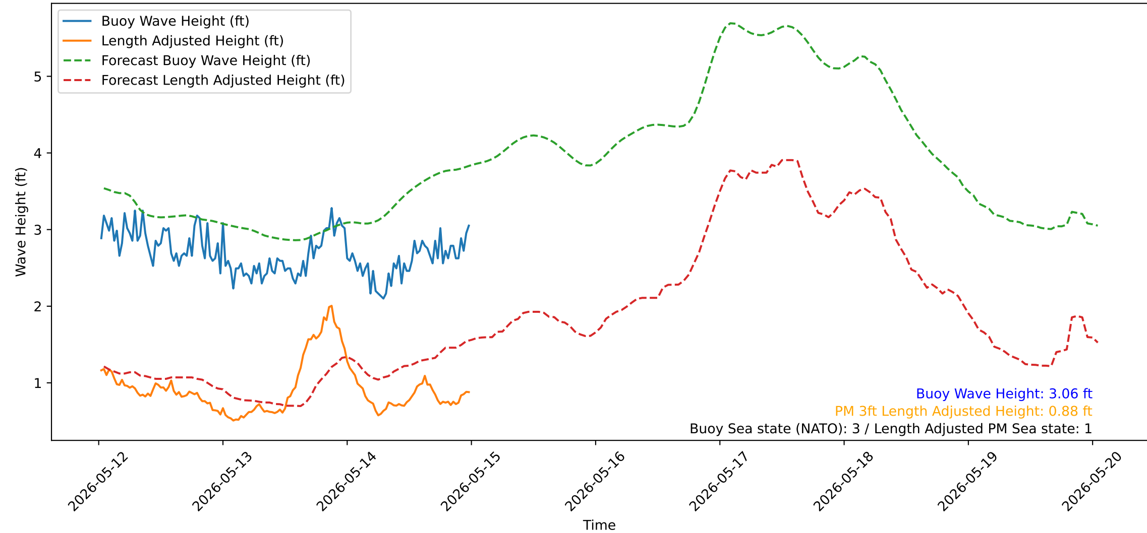
Wave Heights over Time for Green Beach at 2026-05-15 00:31:13
