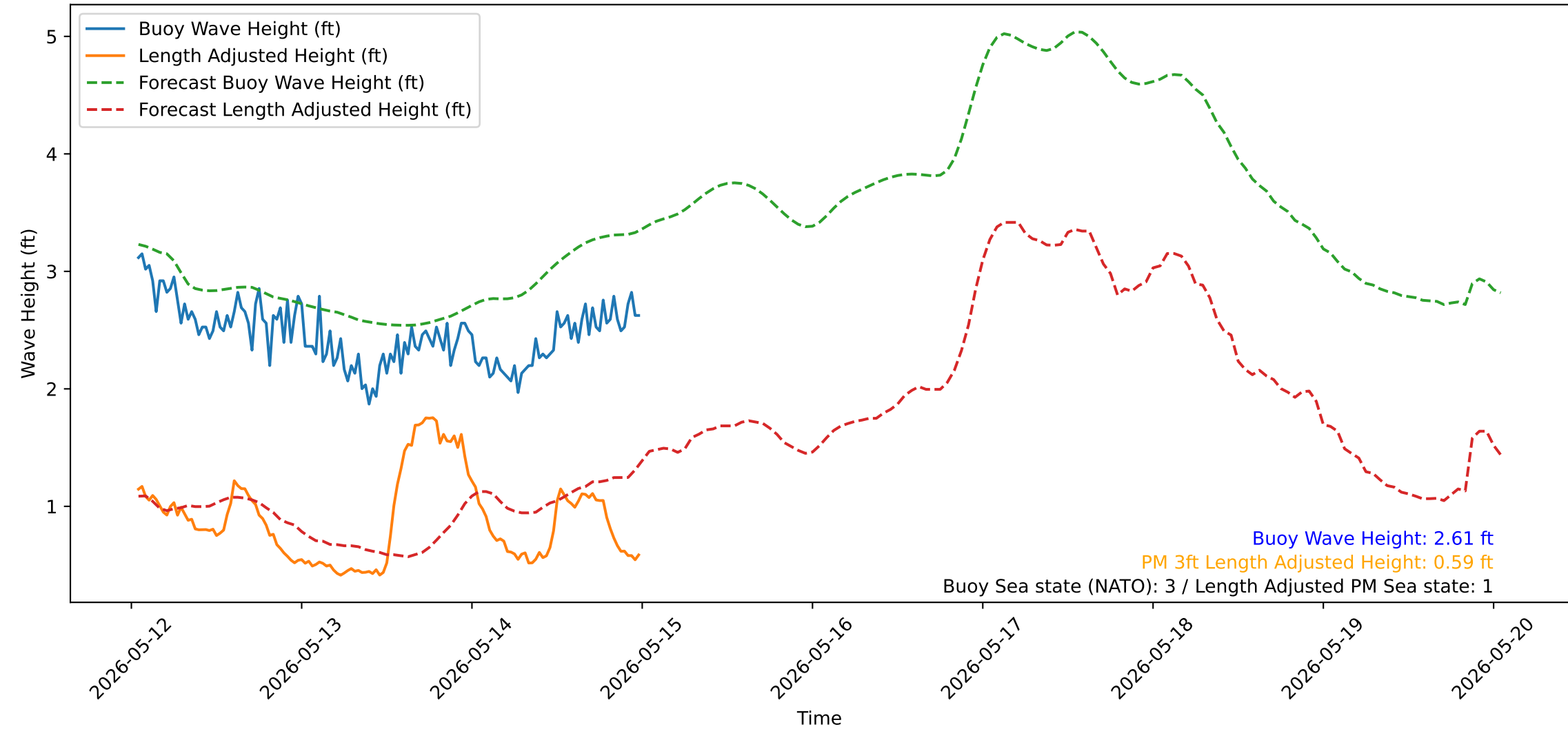
Wave Heights over Time for Red Beach at 2026-05-15 00:30:51
