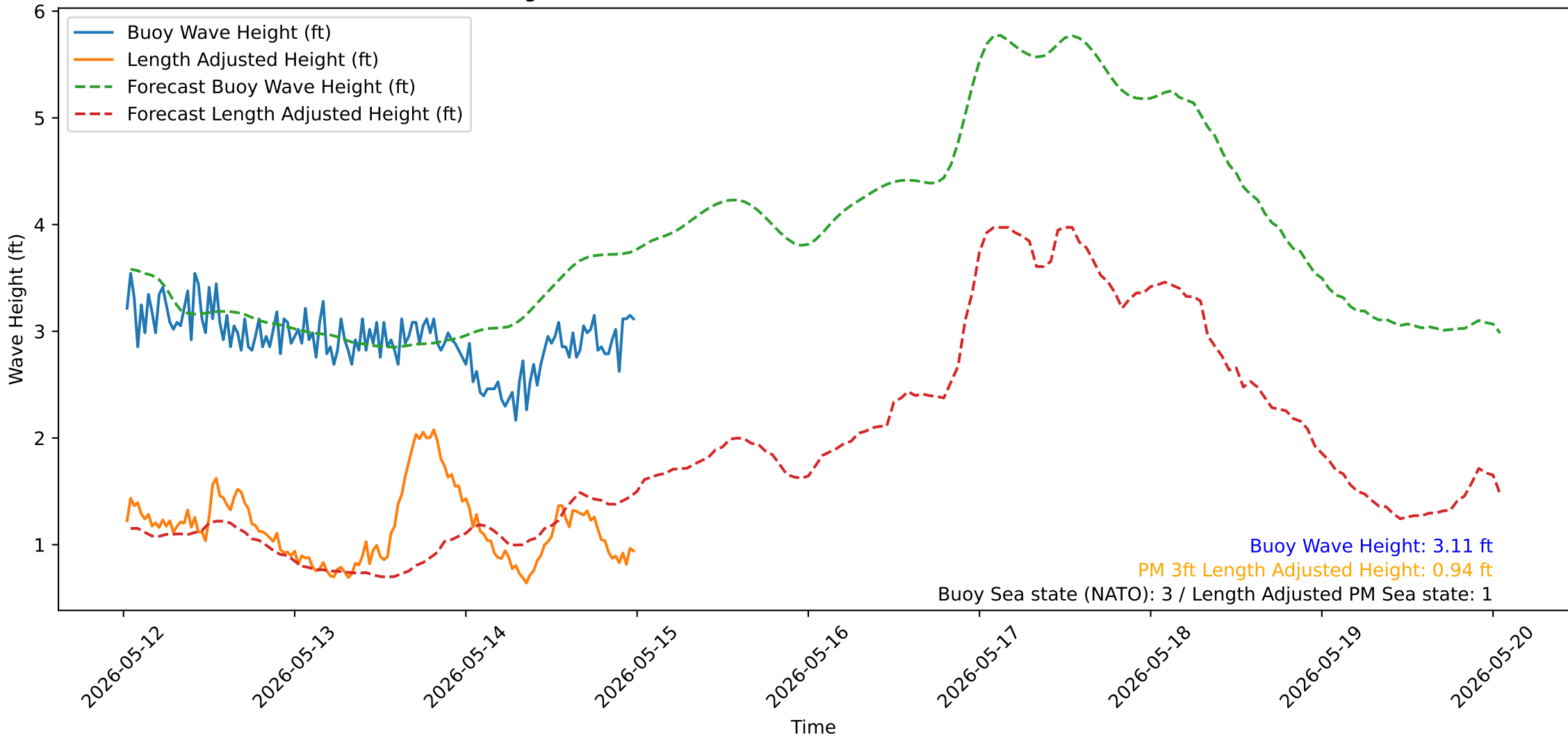
Wave Heights over Time for Oceanside Harbor at 2026-05-15 00:30:31
