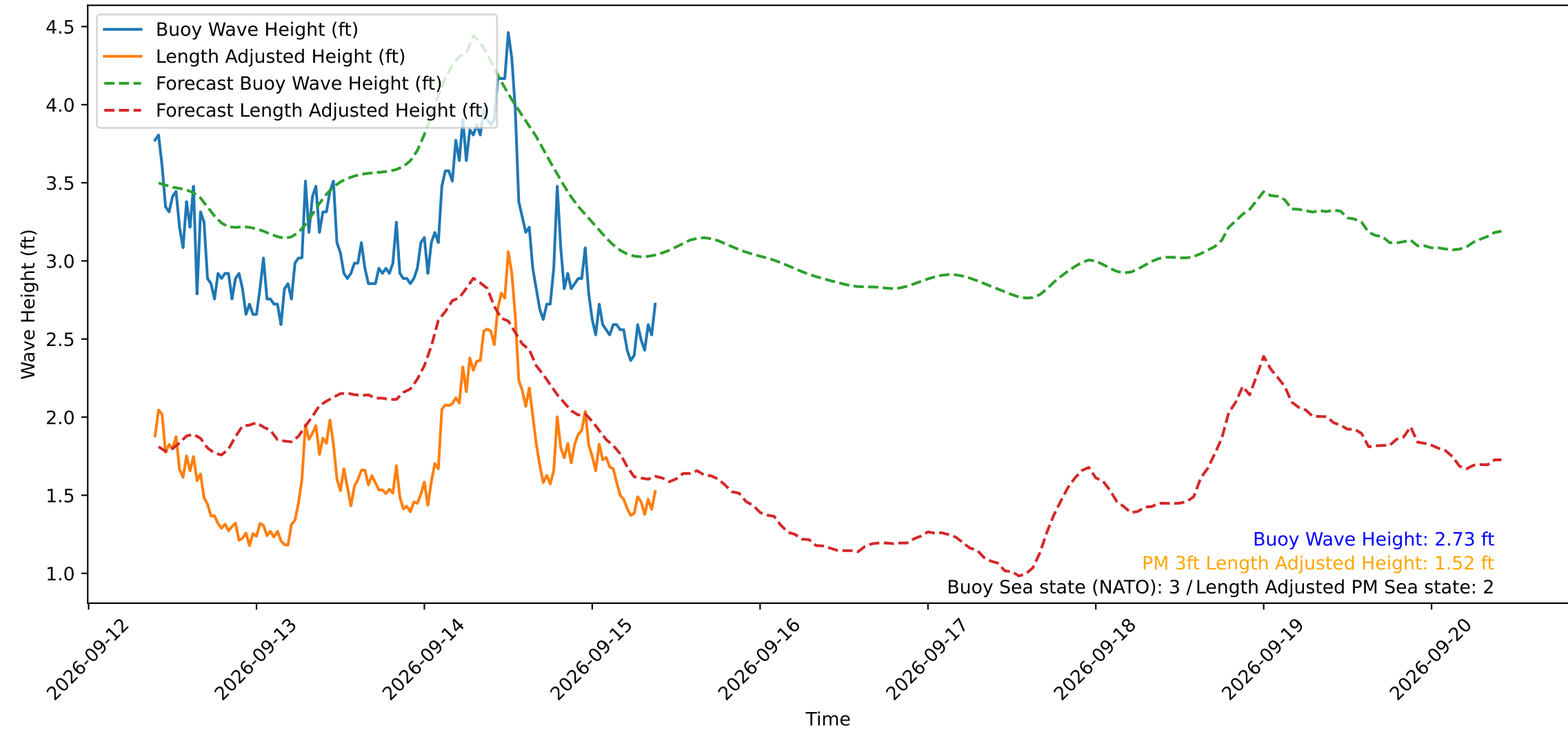
Wave Heights over Time for Oceanside Harbor at 2026-09-15 09:40:29
