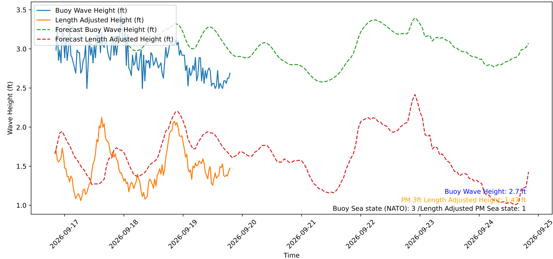
Wave Heights over Time for Green Beach at 2026-09-19 20:01:13
