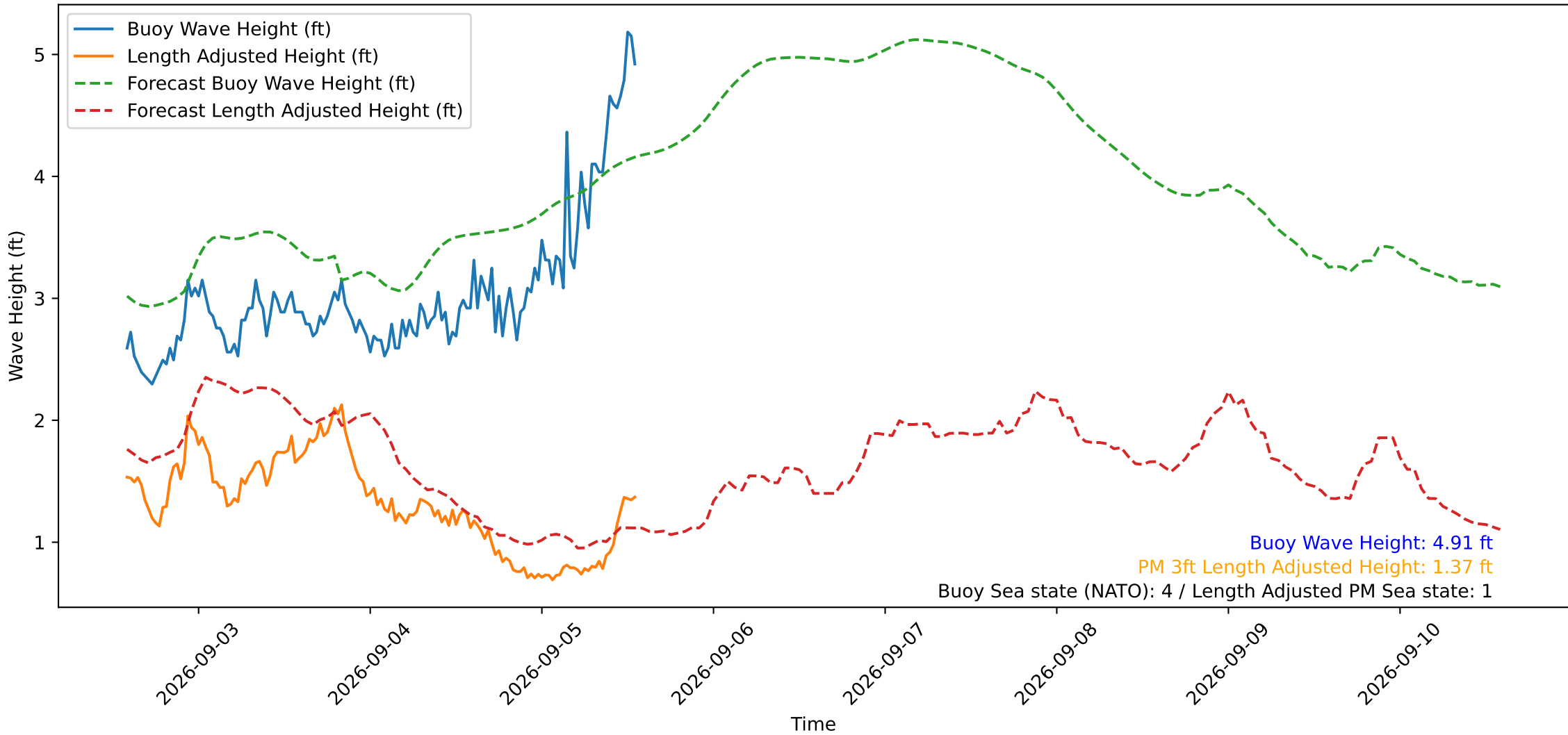
Wave Heights over Time for Red Beach at 2026-09-05 13:50:51
