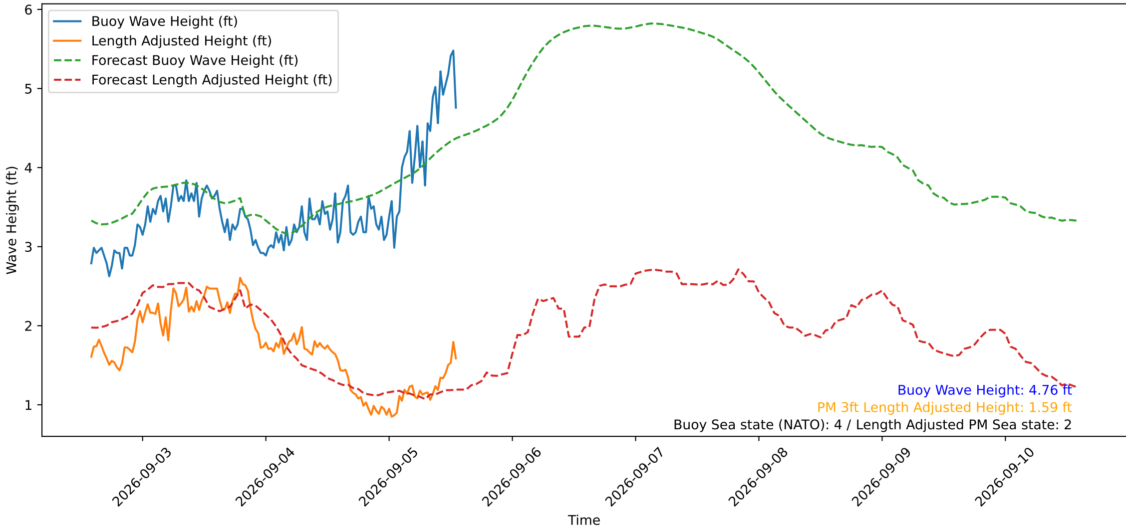
Wave Heights over Time for Oceanside Harbor at 2026-09-05 13:50:30
