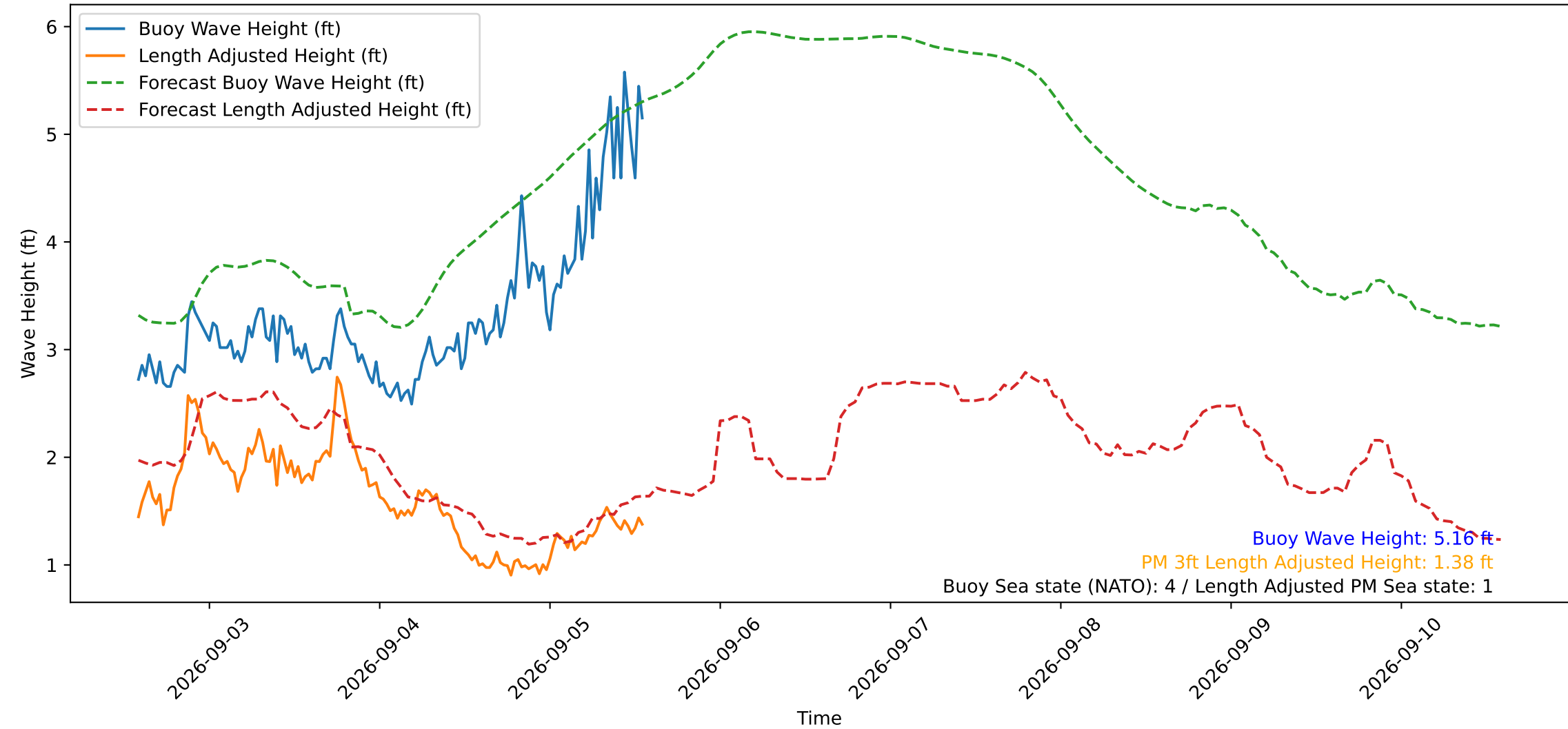
Wave Heights over Time for Green Beach at 2026-09-05 13:51:15
