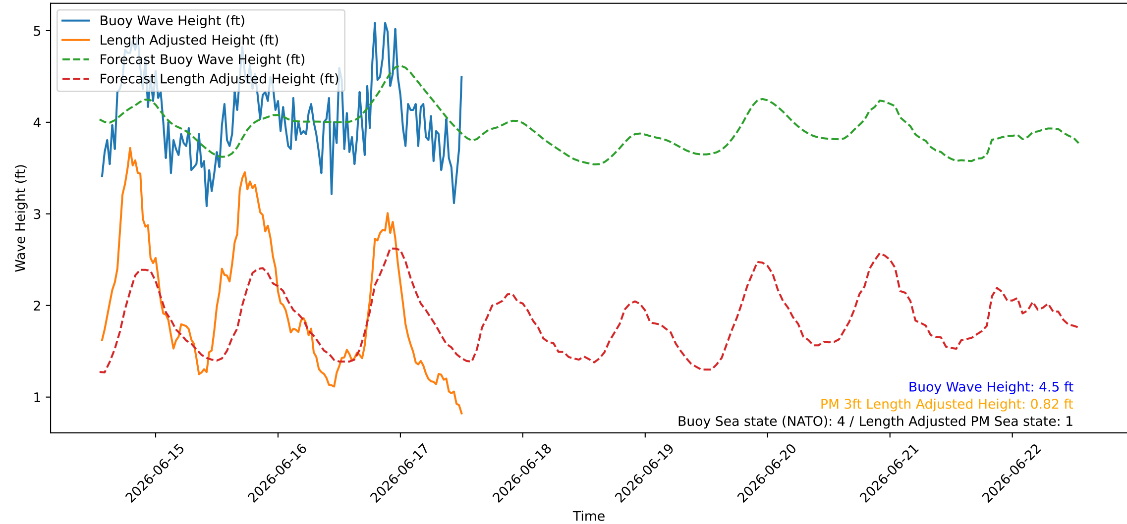
Wave Heights over Time for Green Beach at 2026-06-17 13:21:08
