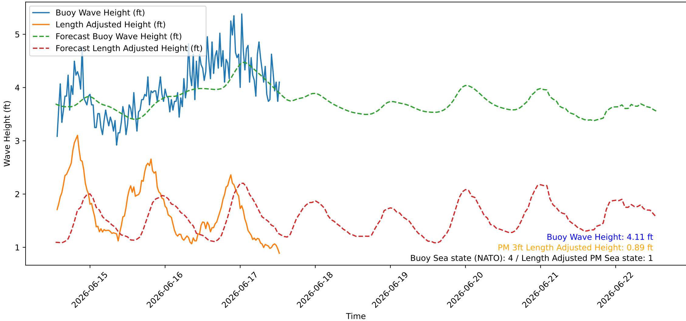
Wave Heights over Time for Red Beach at 2026-06-17 13:20:46
