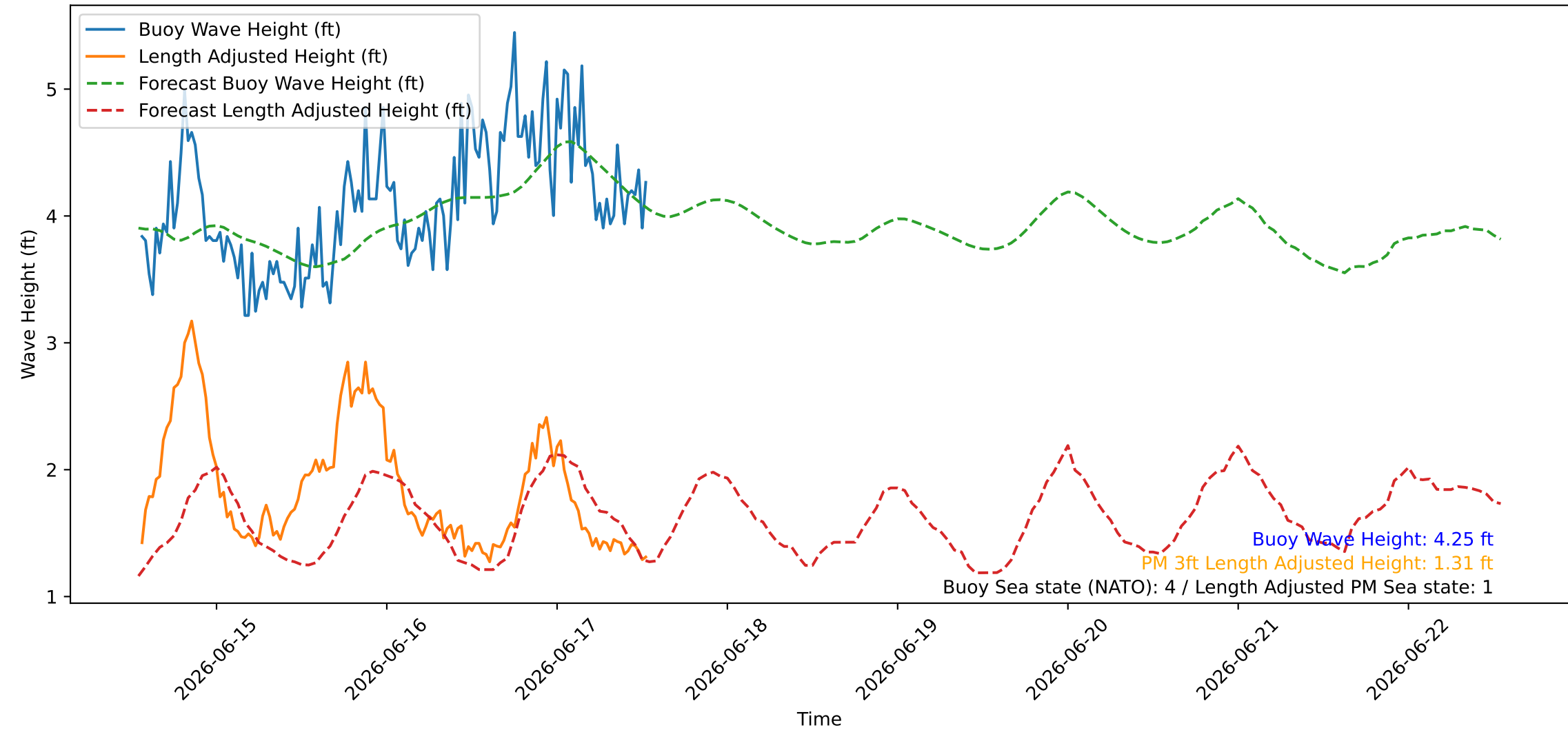
Wave Heights over Time for Oceanside Harbor at 2026-06-17 13:20:26
