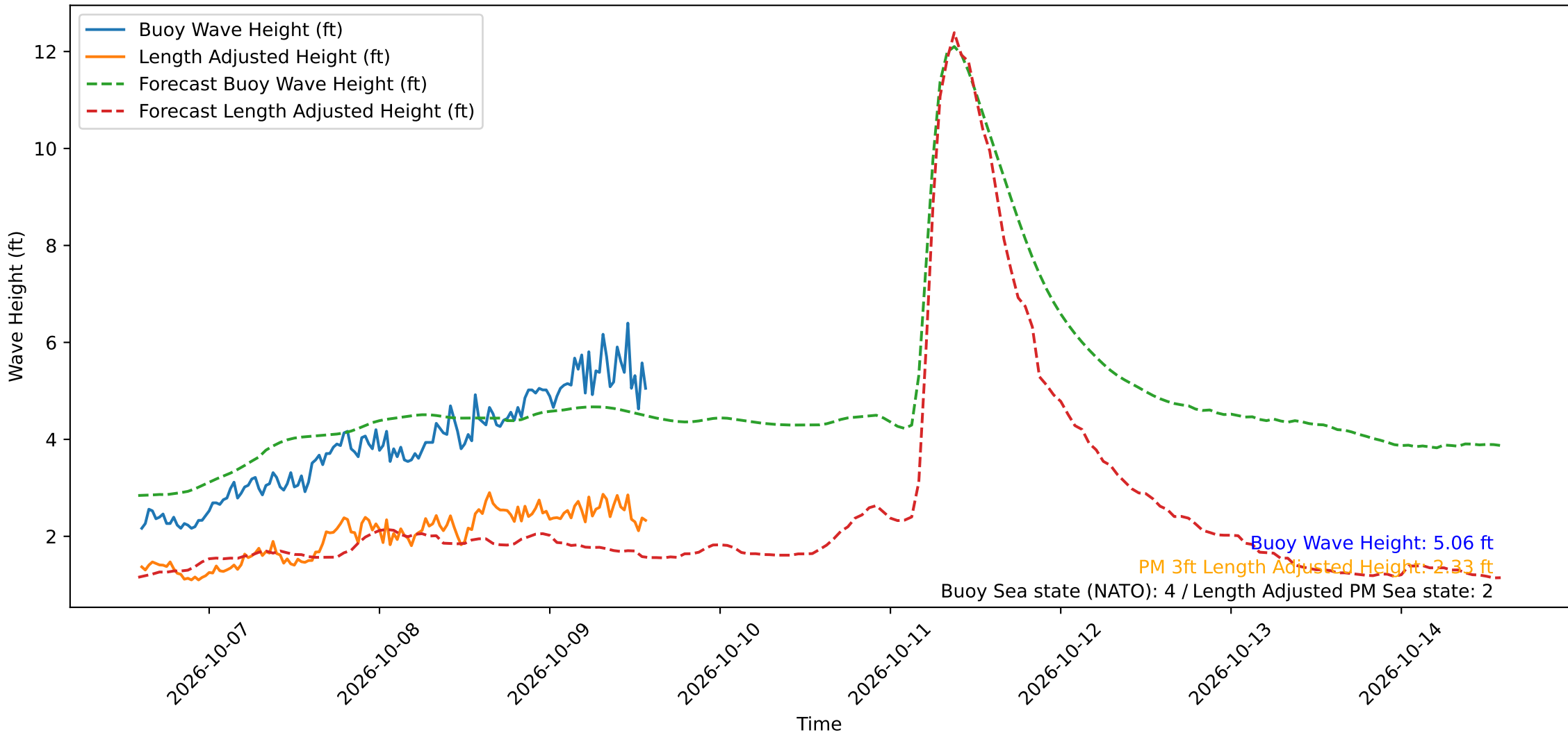
Wave Heights over Time for Oceanside Harbor at 2026-10-09 14:20:29
