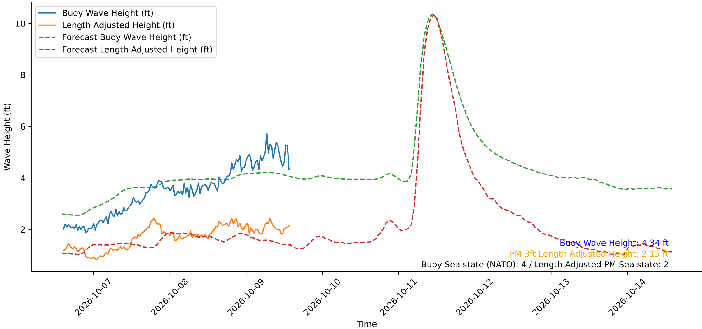
Wave Heights over Time for Red Beach at 2026-10-09 14:20:51
