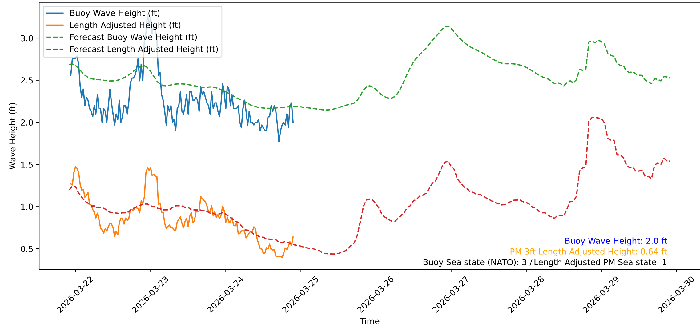
Wave Heights over Time for Green Beach at 2026-03-24 22:21:09
