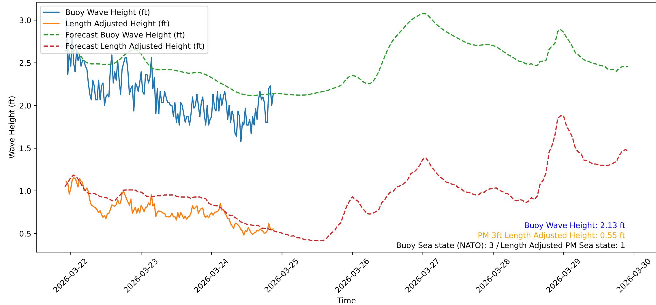
Wave Heights over Time for Oceanside Harbor at 2026-03-24 22:20:31
