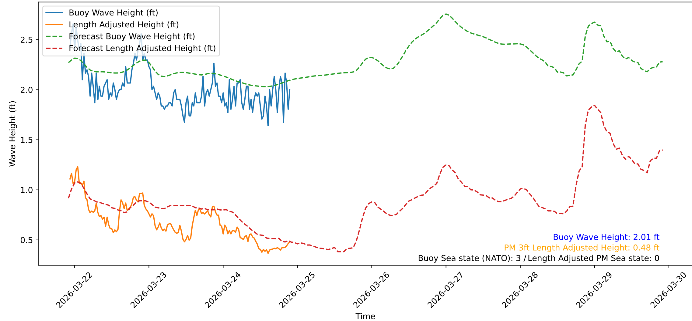
Wave Heights over Time for Red Beach at 2026-03-24 22:20:47
