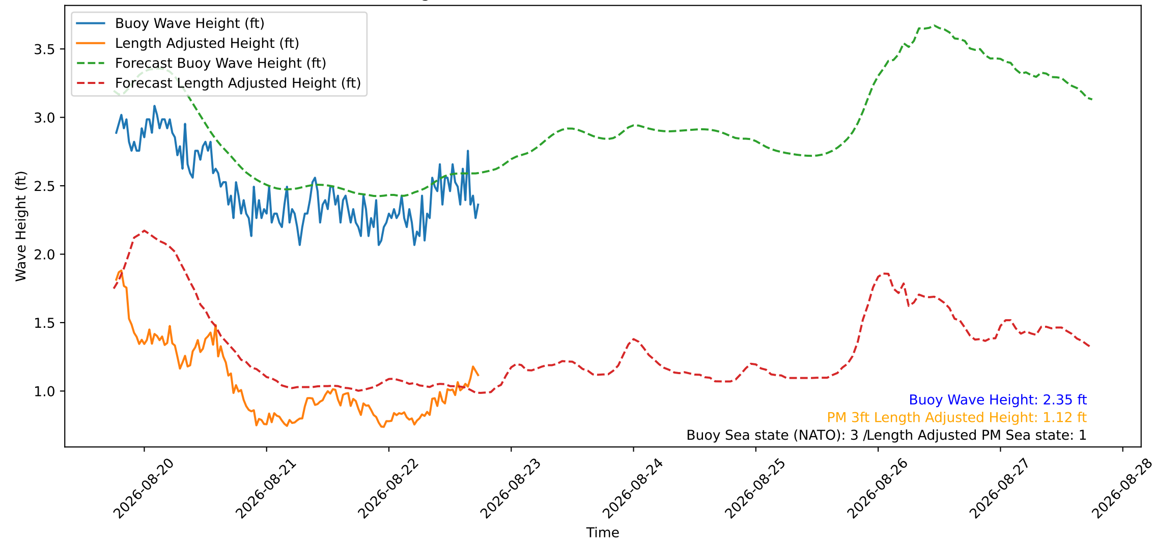
Wave Heights over Time for Red Beach at 2026-08-22 18:20:50
