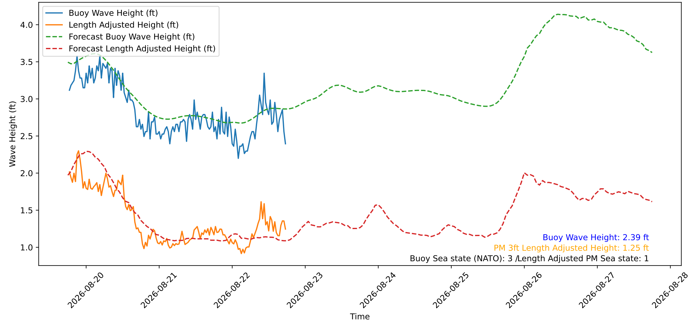
Wave Heights over Time for Oceanside Harbor at 2026-08-22 18:20:29
