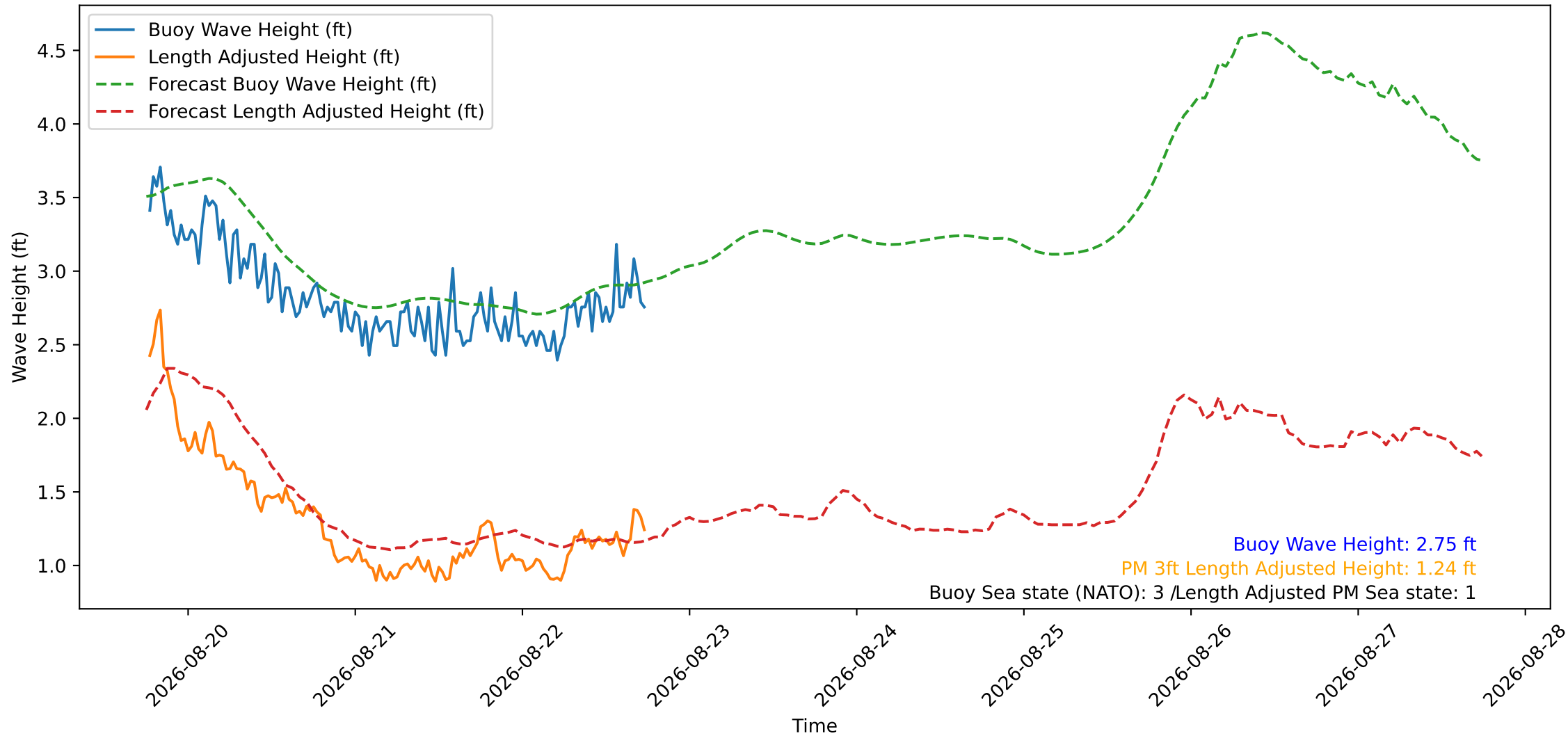
Wave Heights over Time for Green Beach at 2026-08-22 18:21:14
