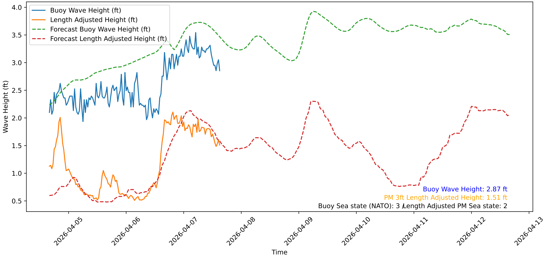
Wave Heights over Time for Red Beach at 2026-04-07 15:50:49
