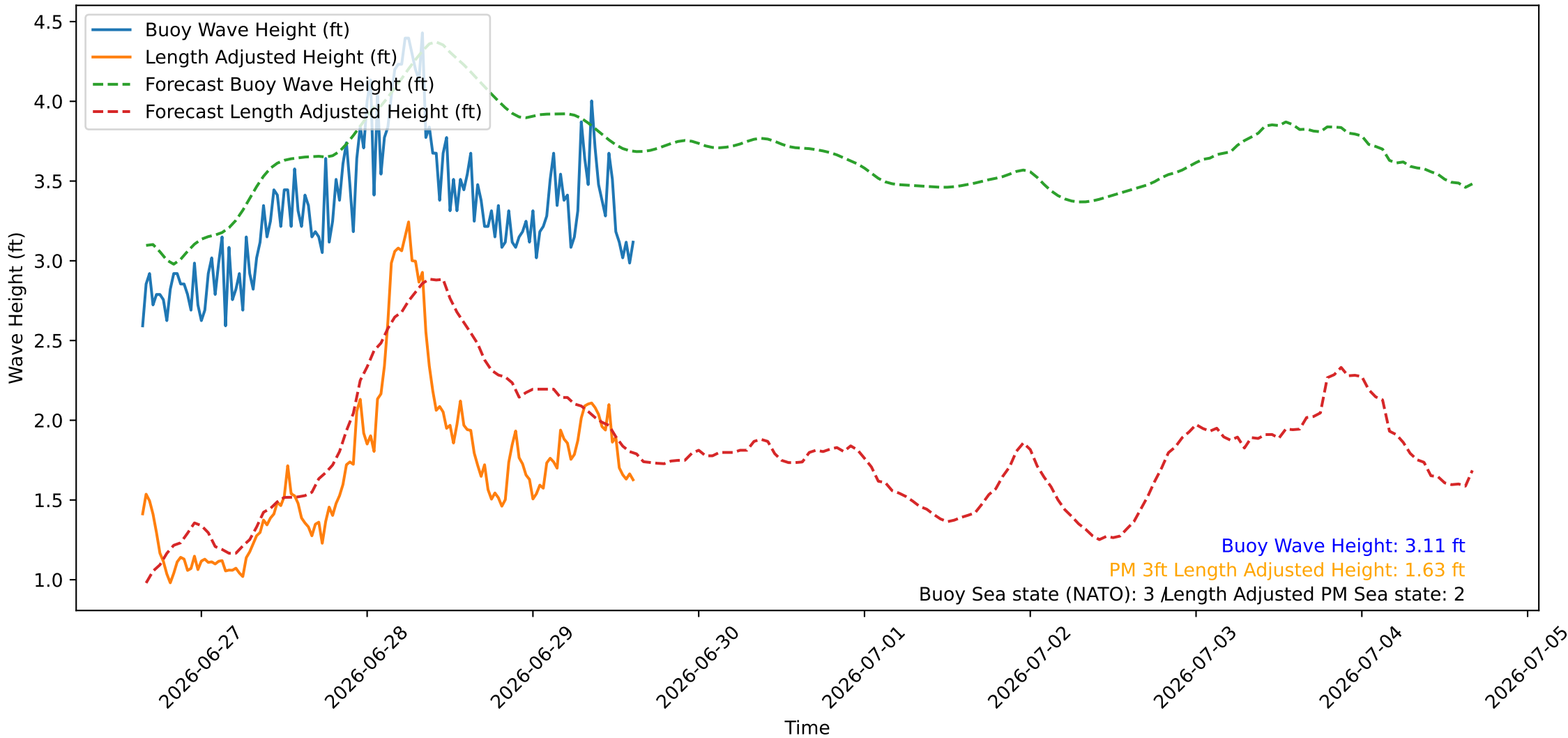
Wave Heights over Time for Oceanside Harbor at 2026-06-29 15:30:26
