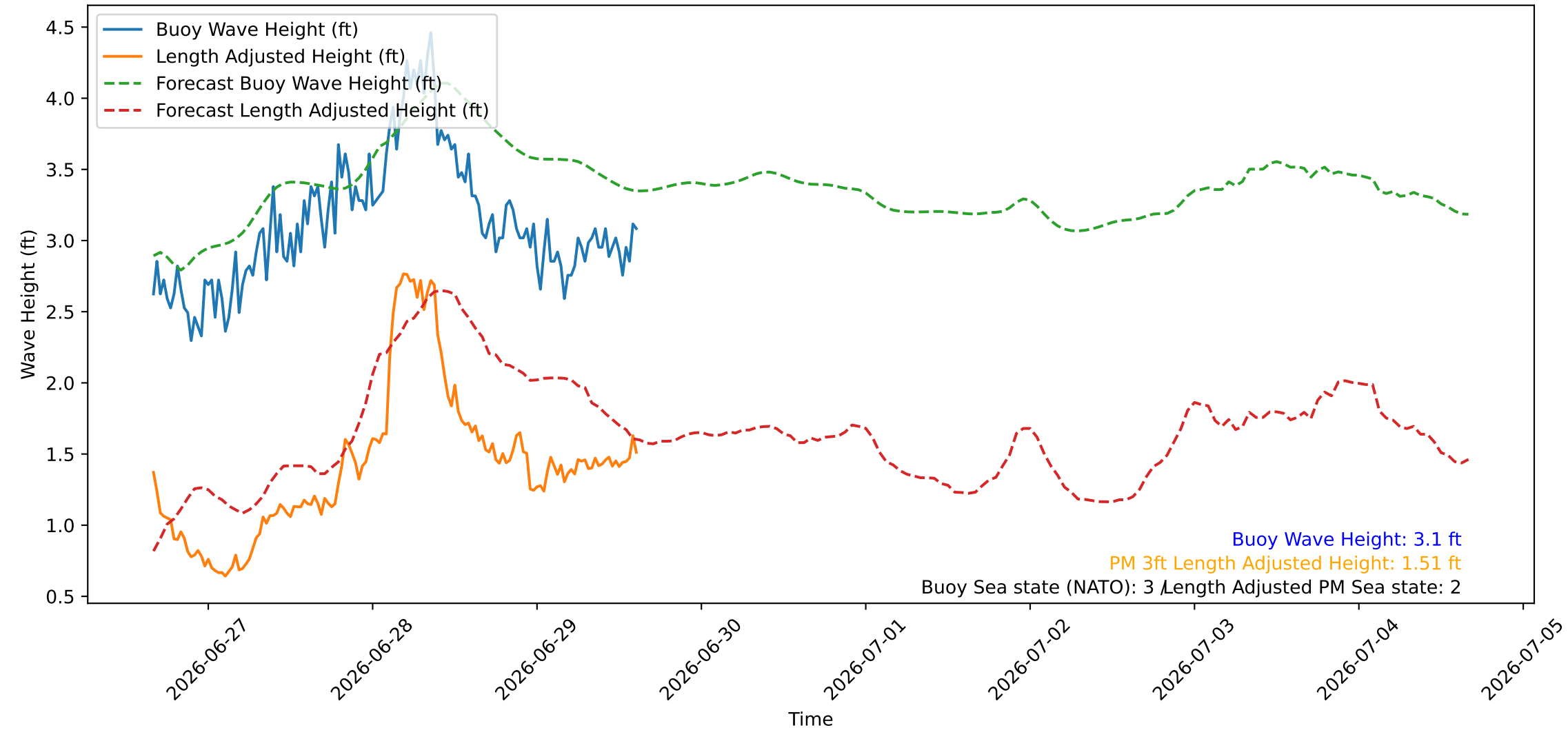
Wave Heights over Time for Red Beach at 2026-06-29 15:30:45
