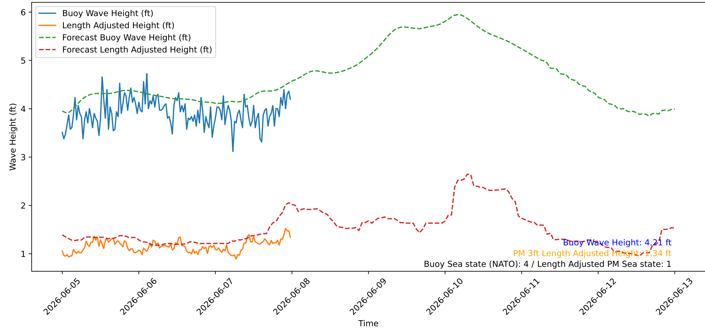
Wave Heights over Time for Green Beach at 2026-06-08 00:11:08
