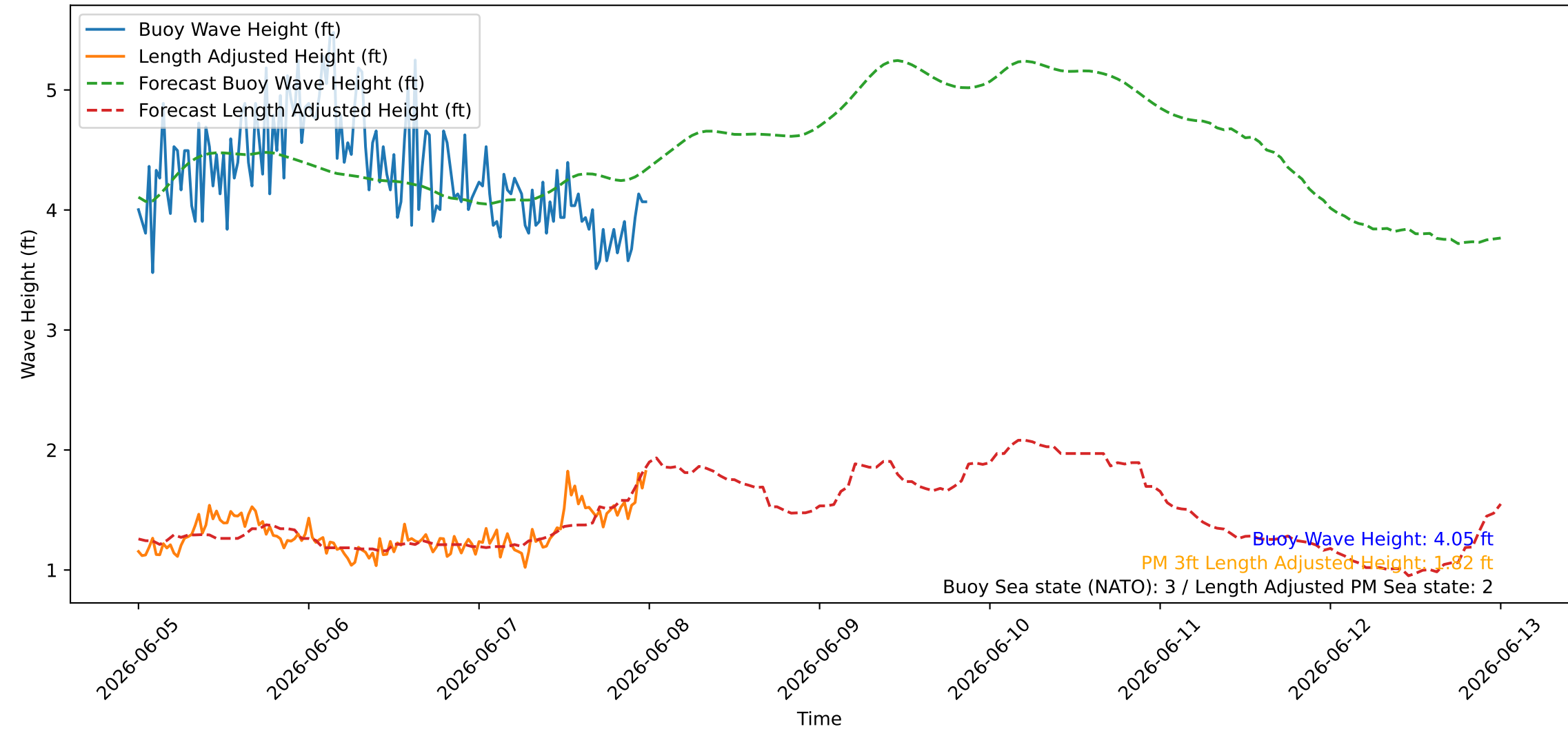
Wave Heights over Time for Oceanside Harbor at 2026-06-08 00:10:26
