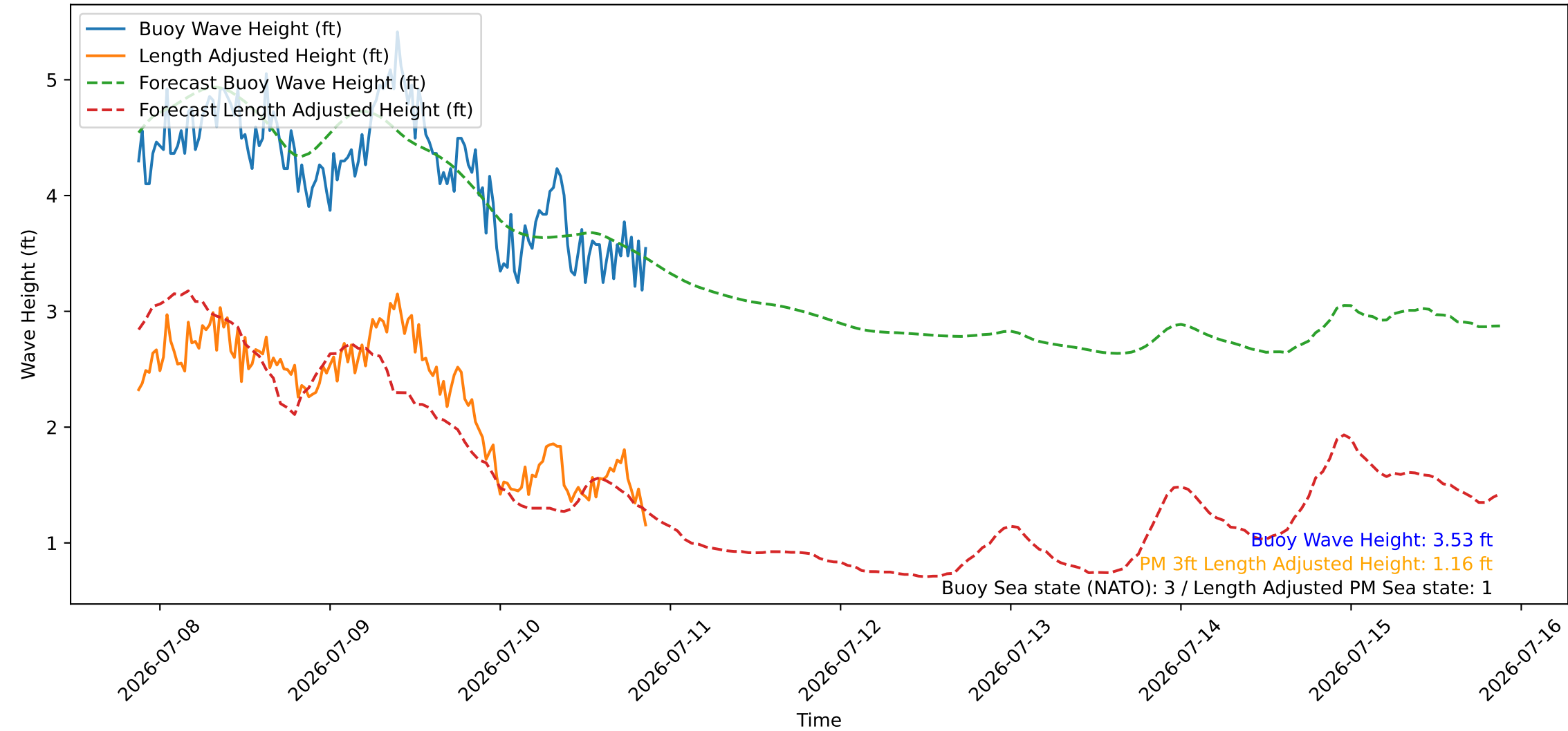
Wave Heights over Time for Oceanside Harbor at 2026-07-10 21:10:26
