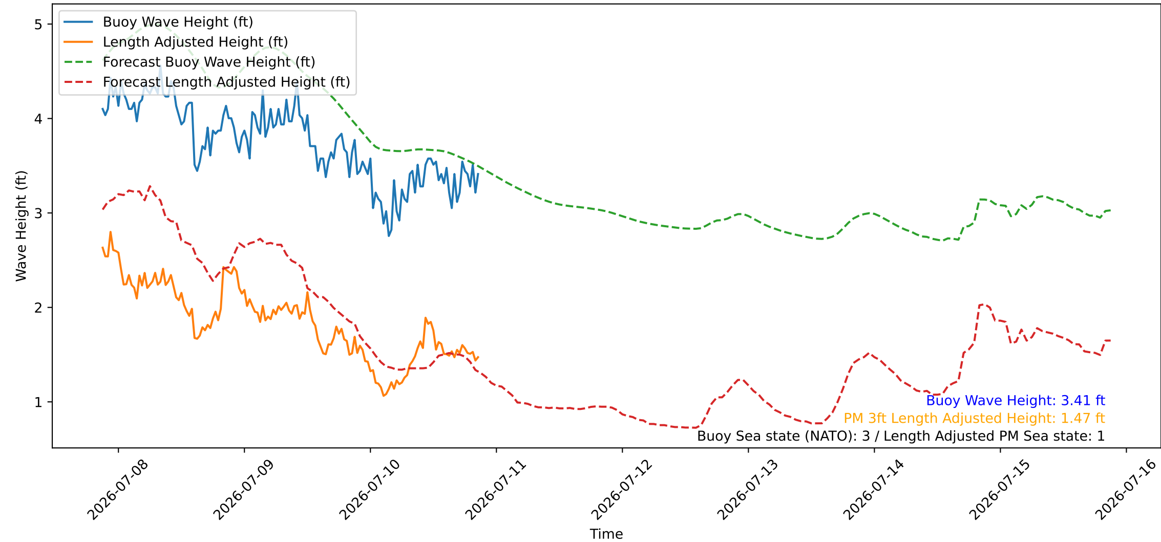
Wave Heights over Time for Green Beach at 2026-07-10 21:11:08
