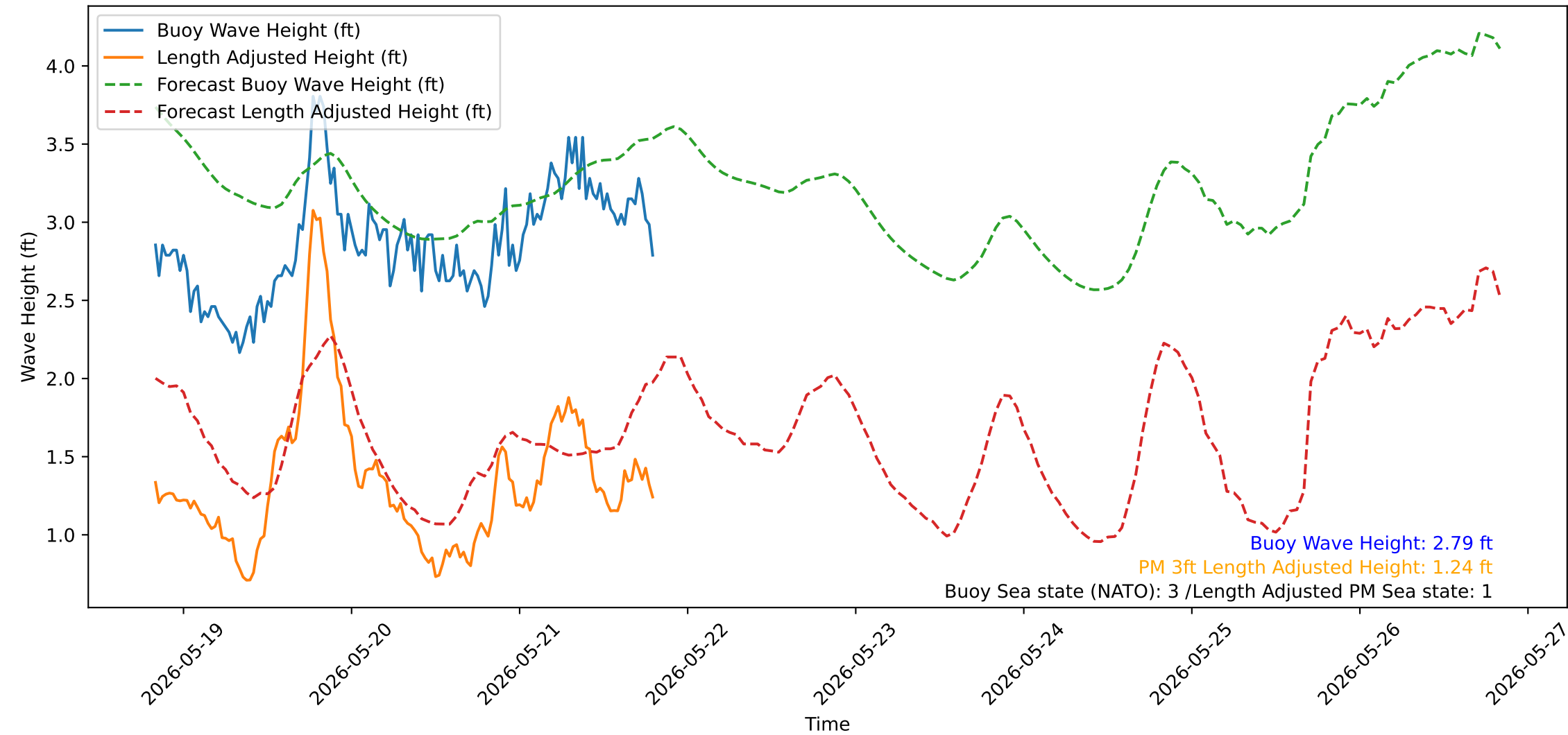
Wave Heights over Time for Green Beach at 2026-05-21 19:51:14
