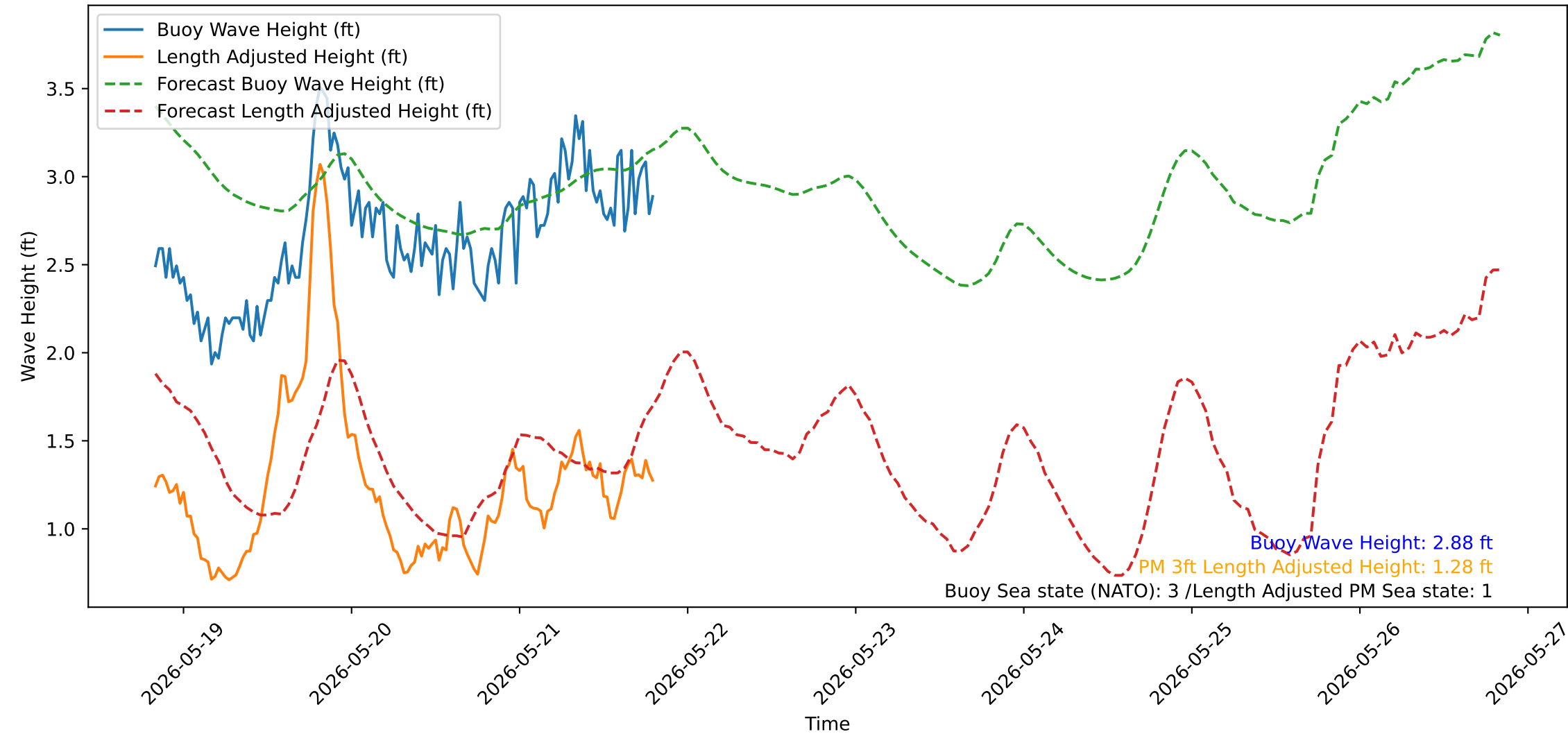
Wave Heights over Time for Red Beach at 2026-05-21 19:50:51
