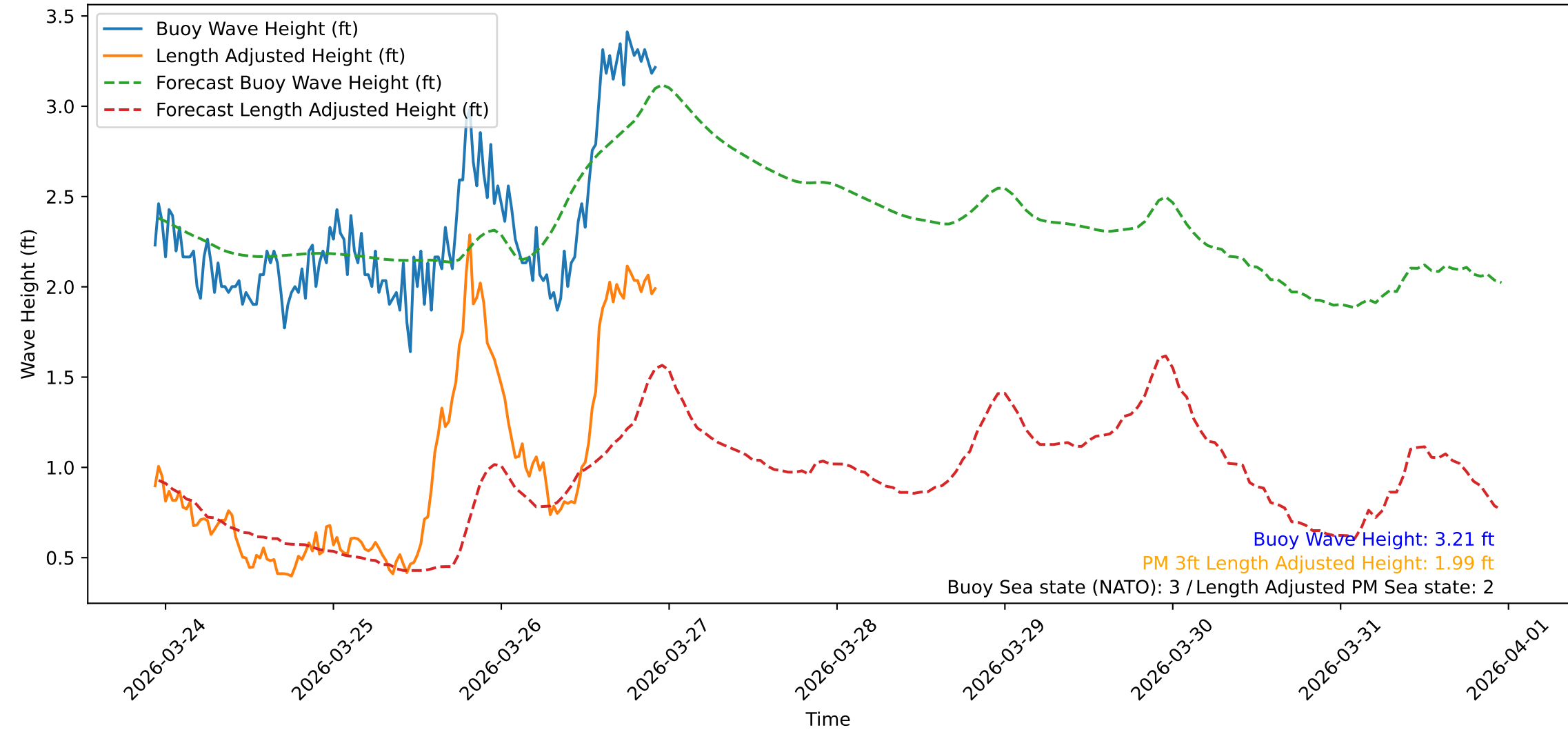
Wave Heights over Time for Green Beach at 2026-03-26 22:41:10
