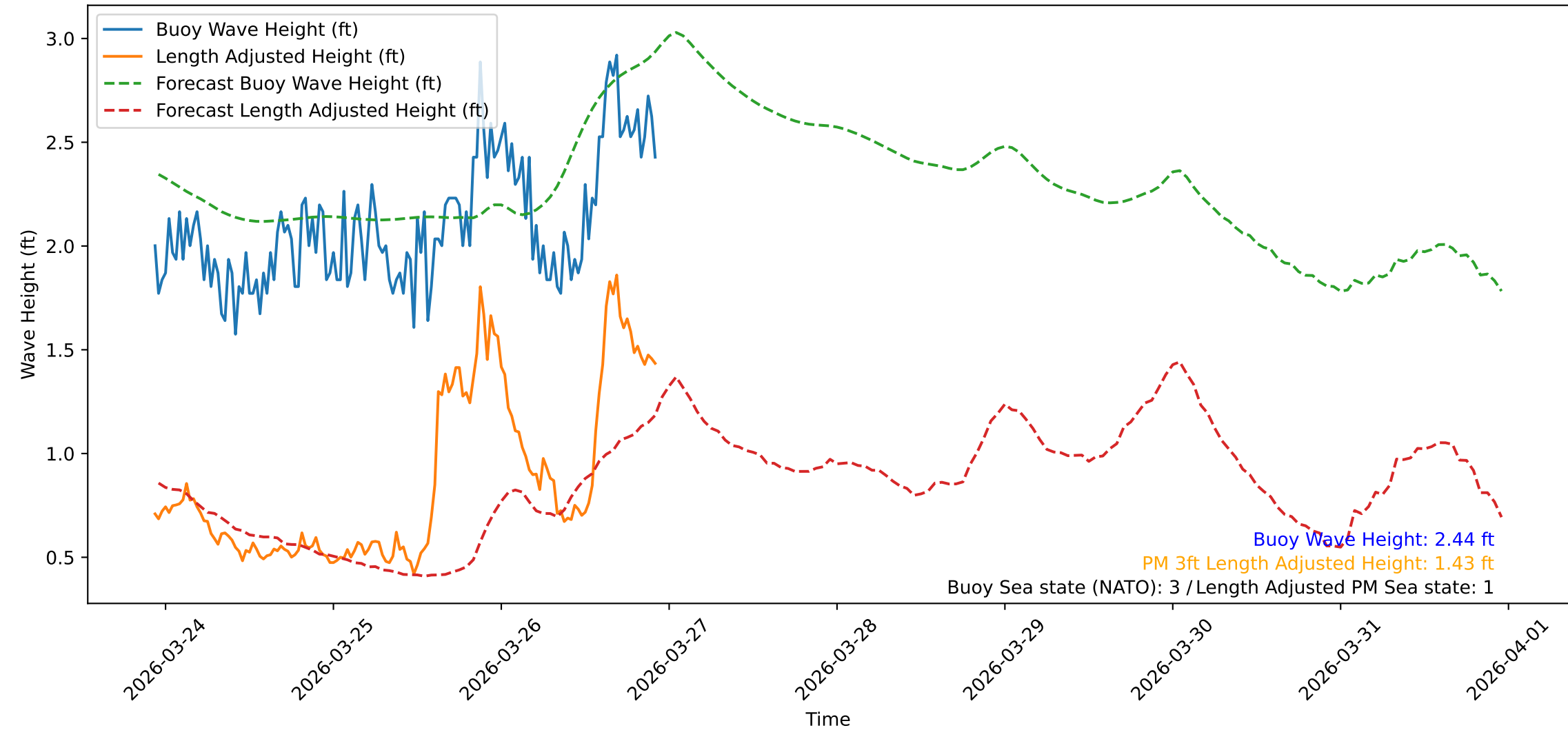
Wave Heights over Time for Oceanside Harbor at 2026-03-26 22:40:31
