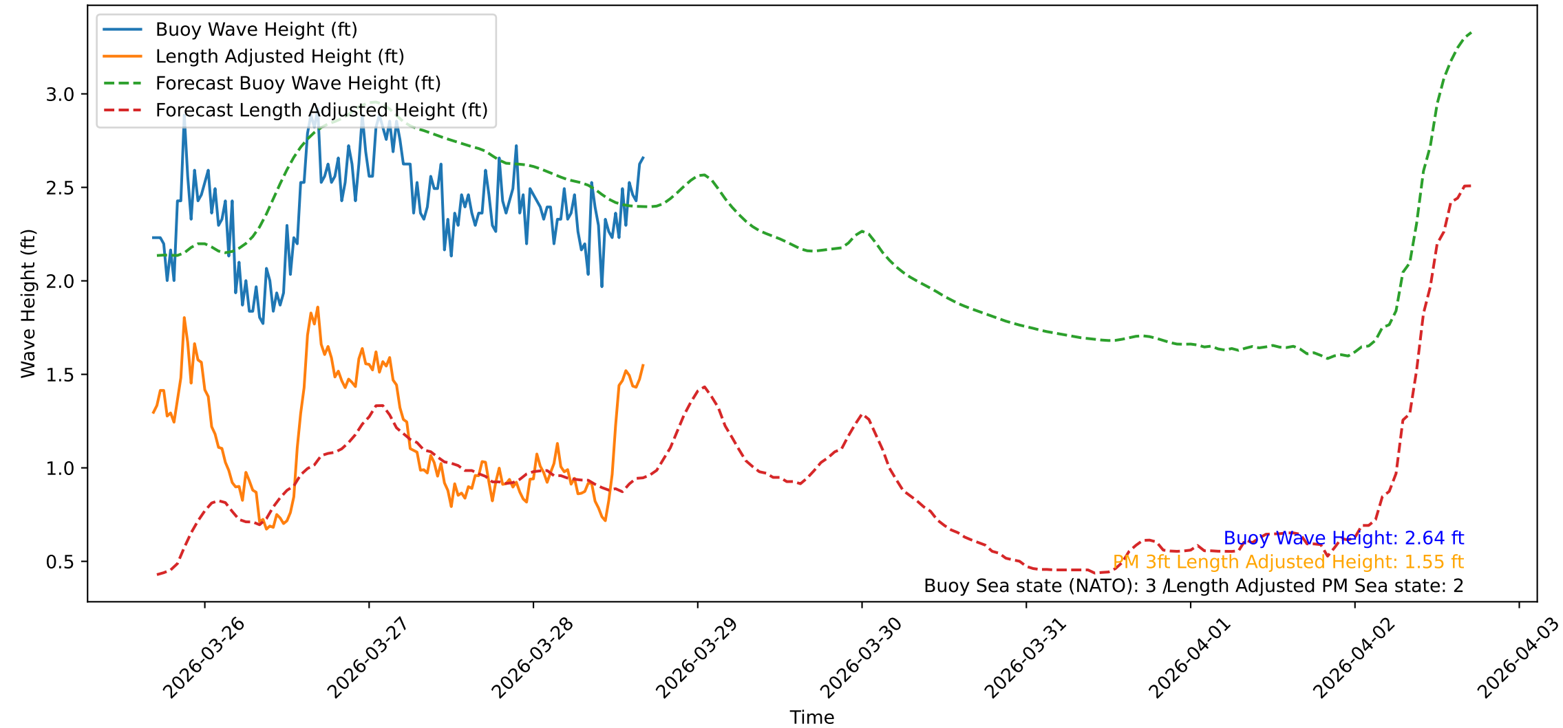
Wave Heights over Time for Oceanside Harbor at 2026-03-28 16:40:30
