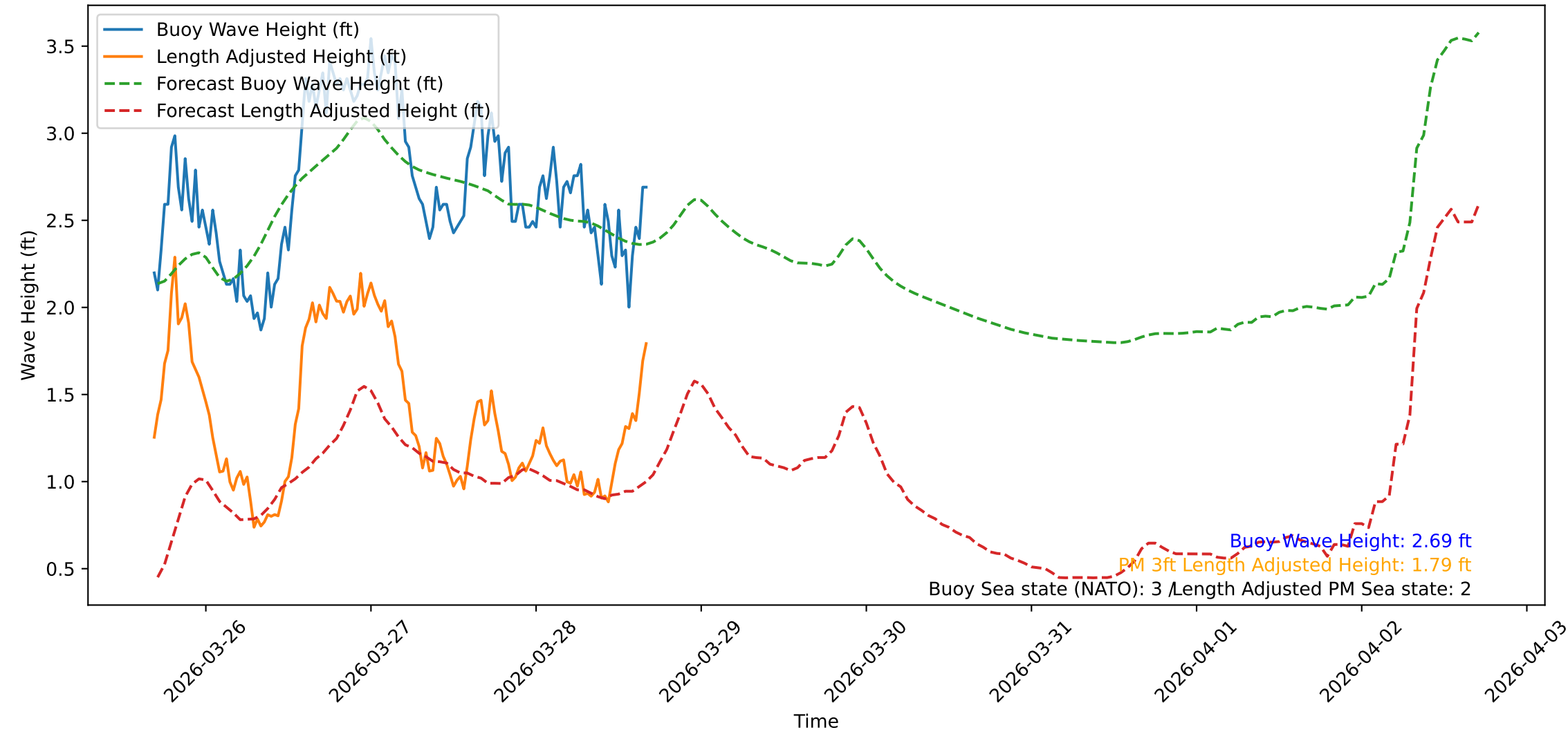
Wave Heights over Time for Green Beach at 2026-03-28 16:41:08
