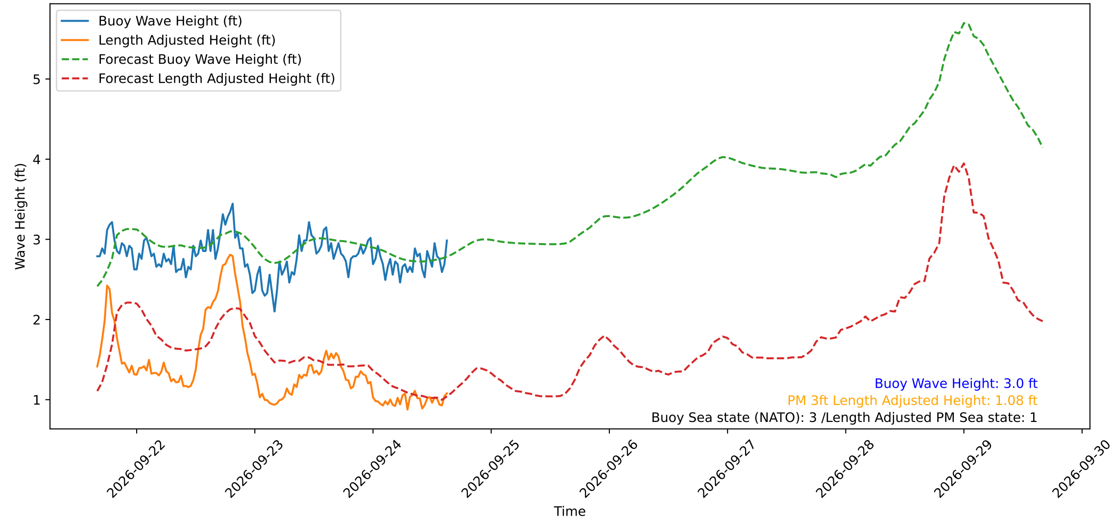
Wave Heights over Time for Green Beach at 2026-09-24 15:41:11
