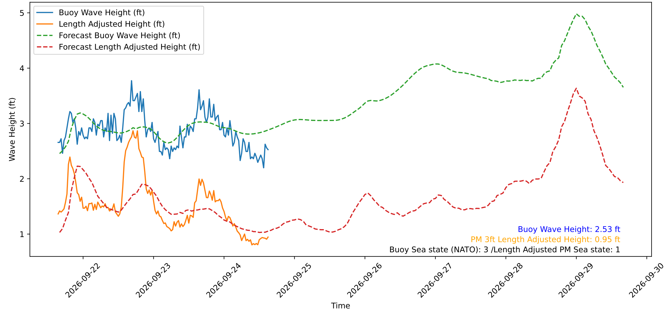
Wave Heights over Time for Oceanside Harbor at 2026-09-24 15:40:29
