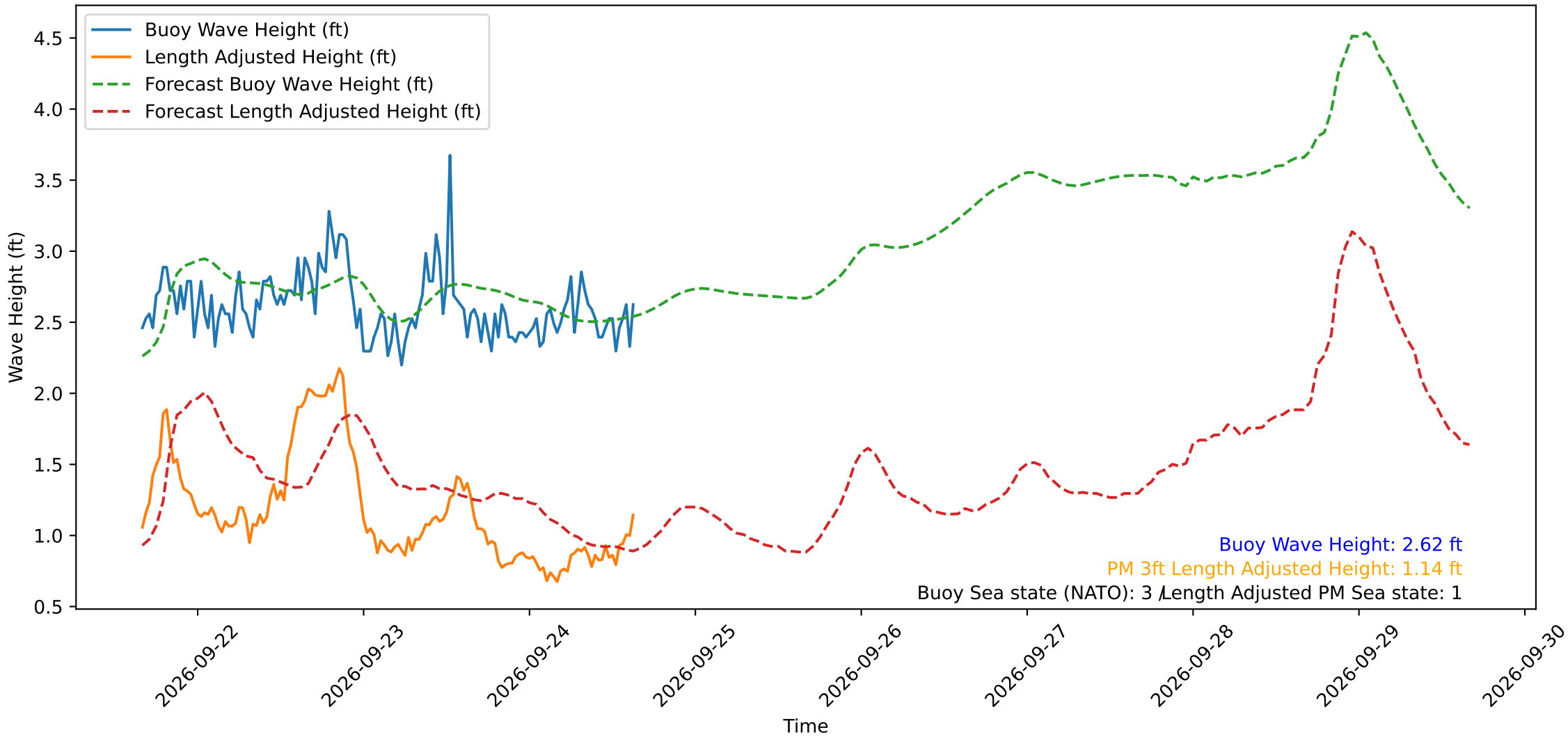
Wave Heights over Time for Red Beach at 2026-09-24 15:40:49
