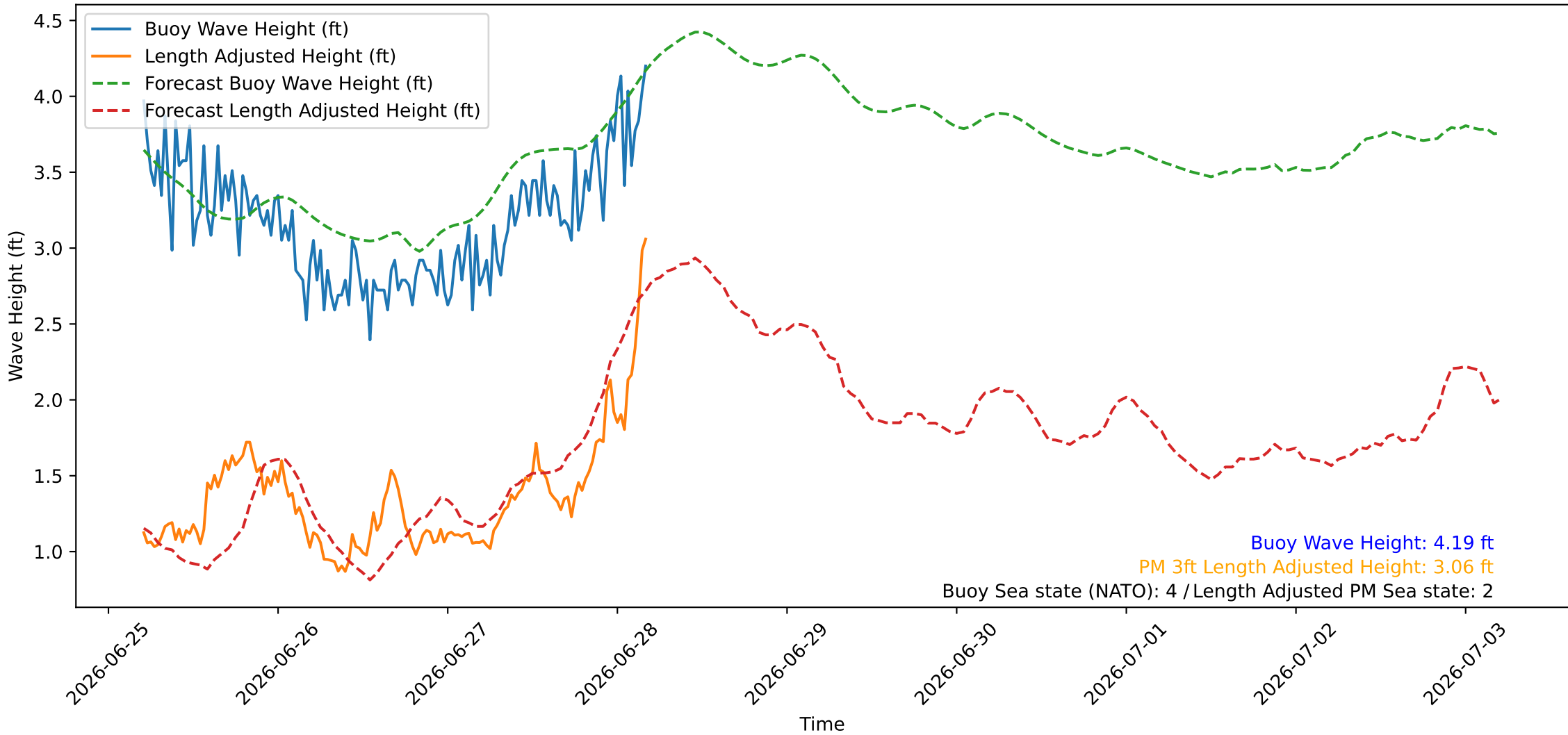
Wave Heights over Time for Oceanside Harbor at 2026-06-28 05:00:26
