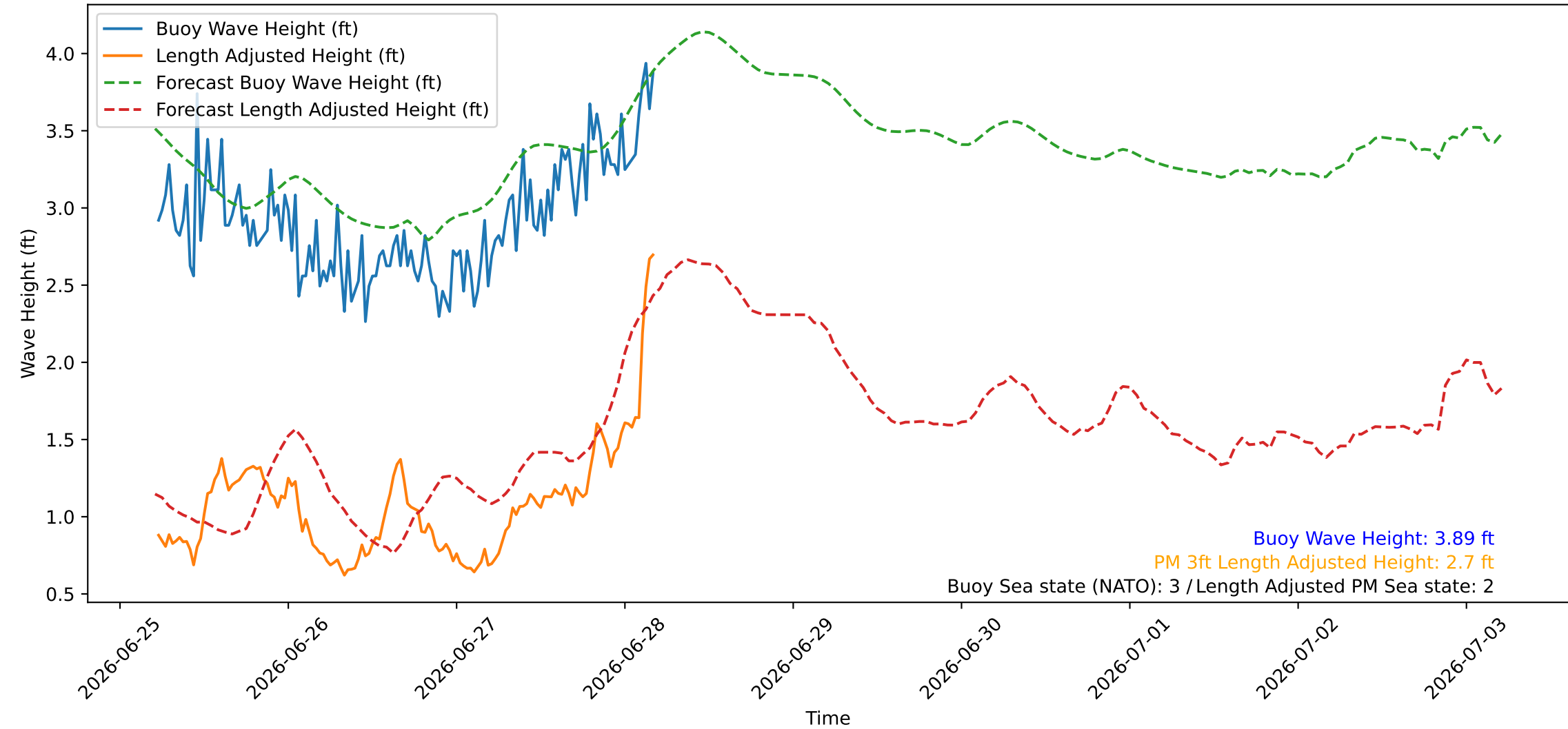
Wave Heights over Time for Red Beach at 2026-06-28 05:00:45
