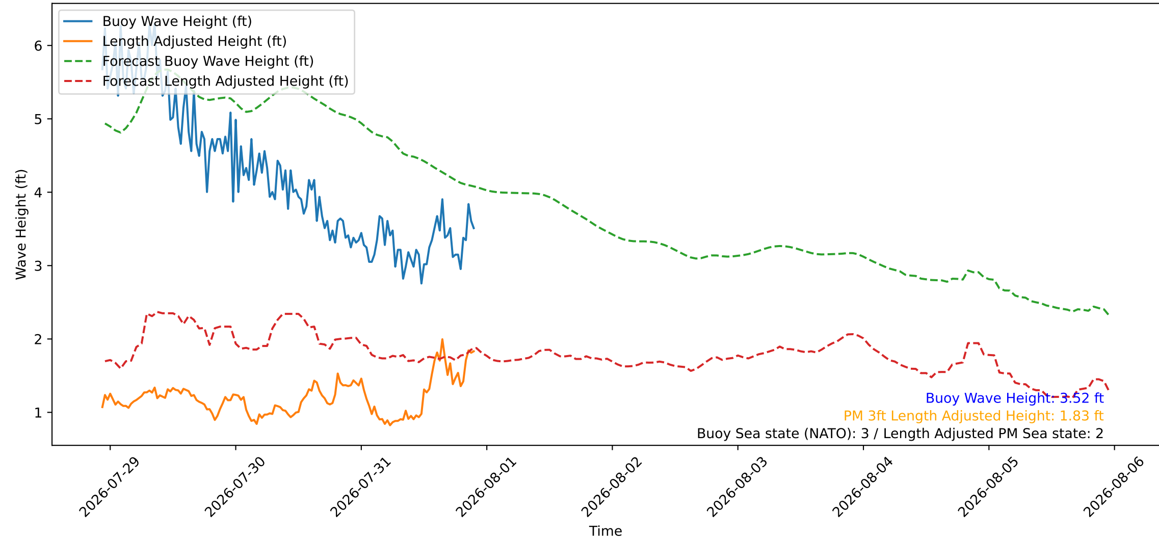
Wave Heights over Time for Green Beach at 2026-07-31 22:31:08
