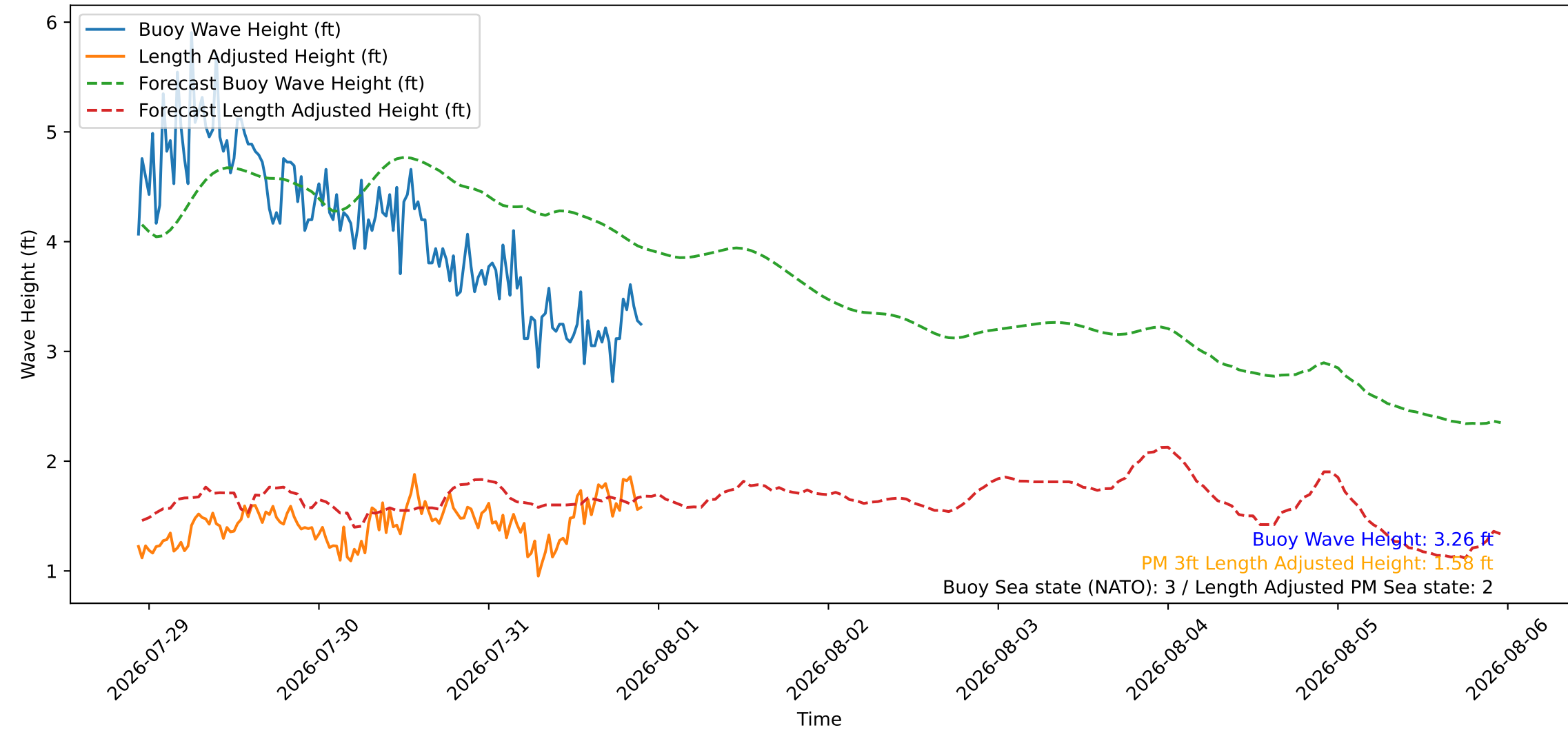
Wave Heights over Time for Oceanside Harbor at 2026-07-31 22:30:26
